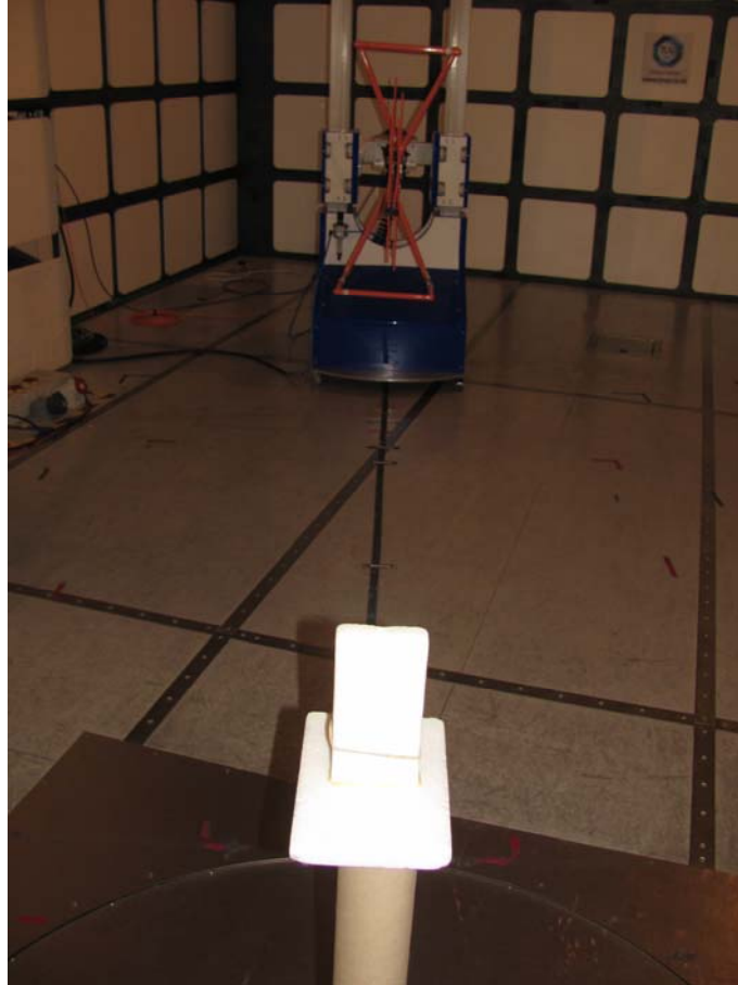
30MHz-1GHz Radiated Emissions
