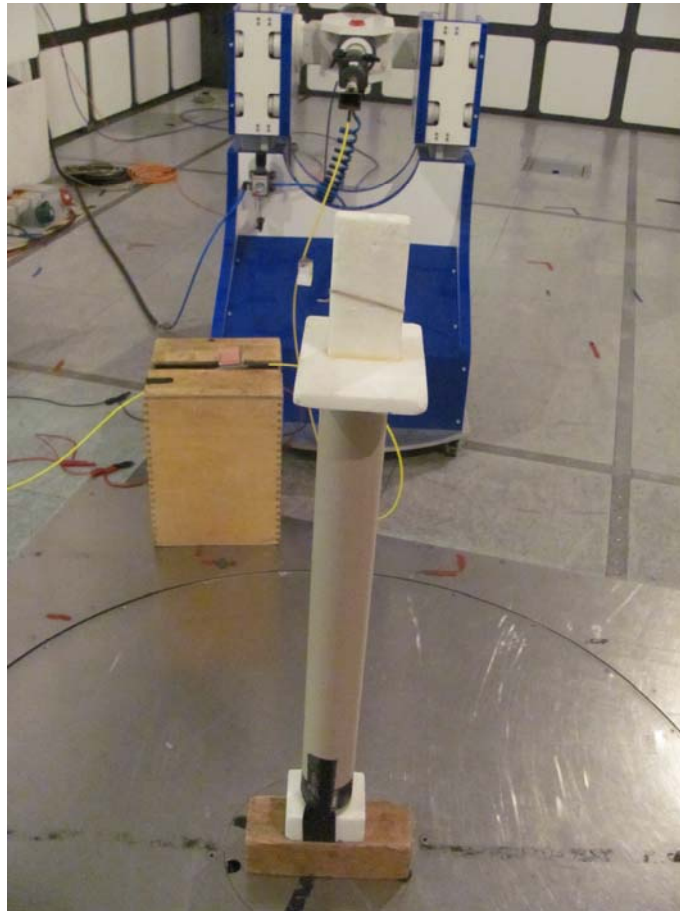
18GHz-25GHz – Radiated Emissions
