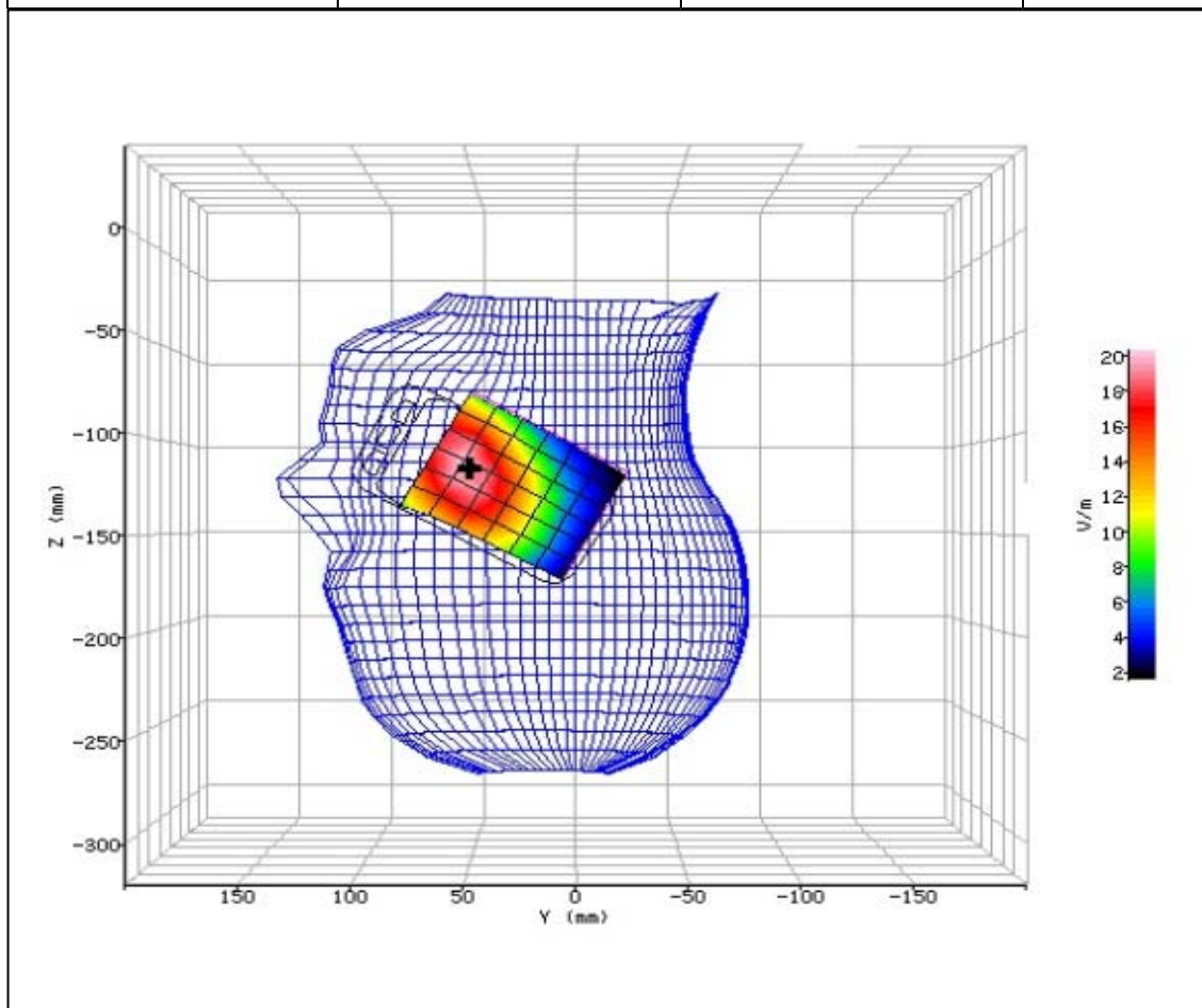
Figure 8: SAR Head Testing Results for the 204SH Mobile Handset at 835MHz.
