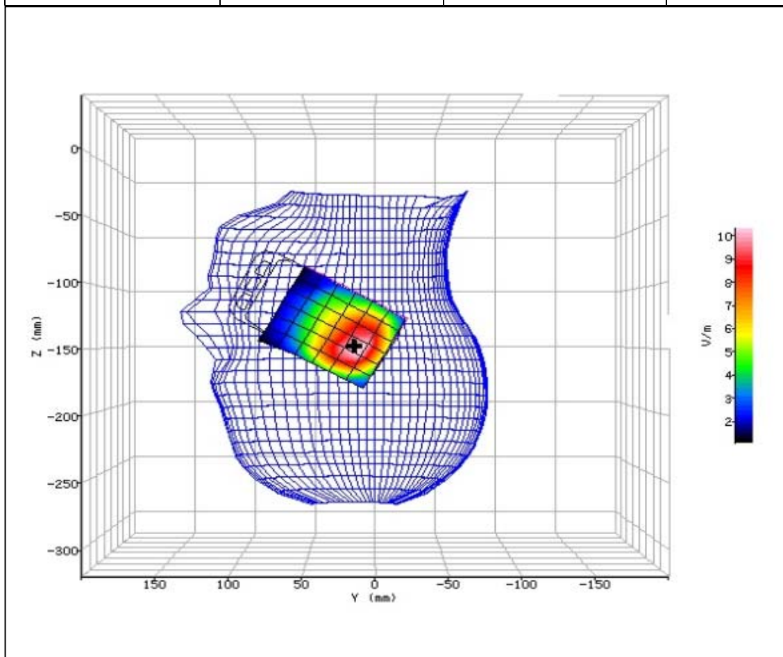
Figure 19: SAR Head Testing Results for the 204SH Mobile Handset at 2412.0MHz.
