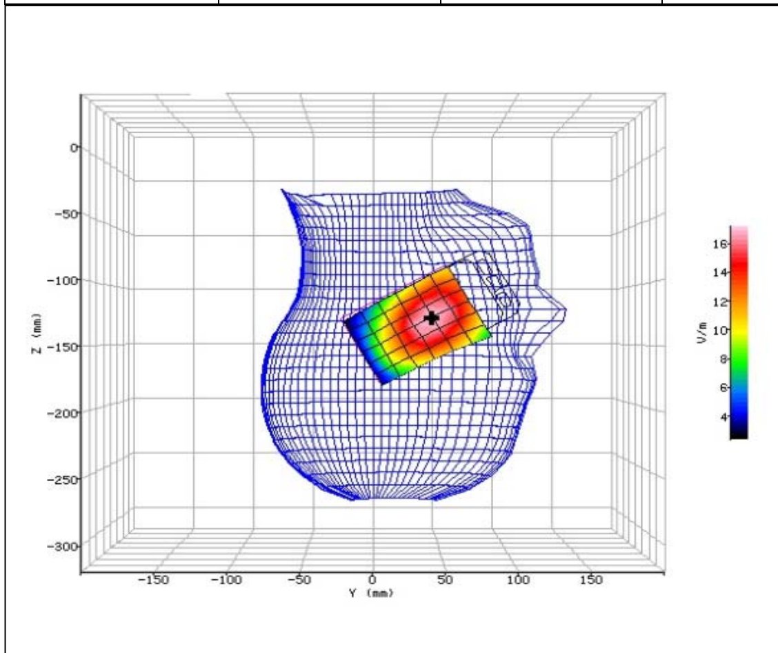
Figure 11: SAR Head Testing Results for the 204SH Mobile Handset at 835MHz.
