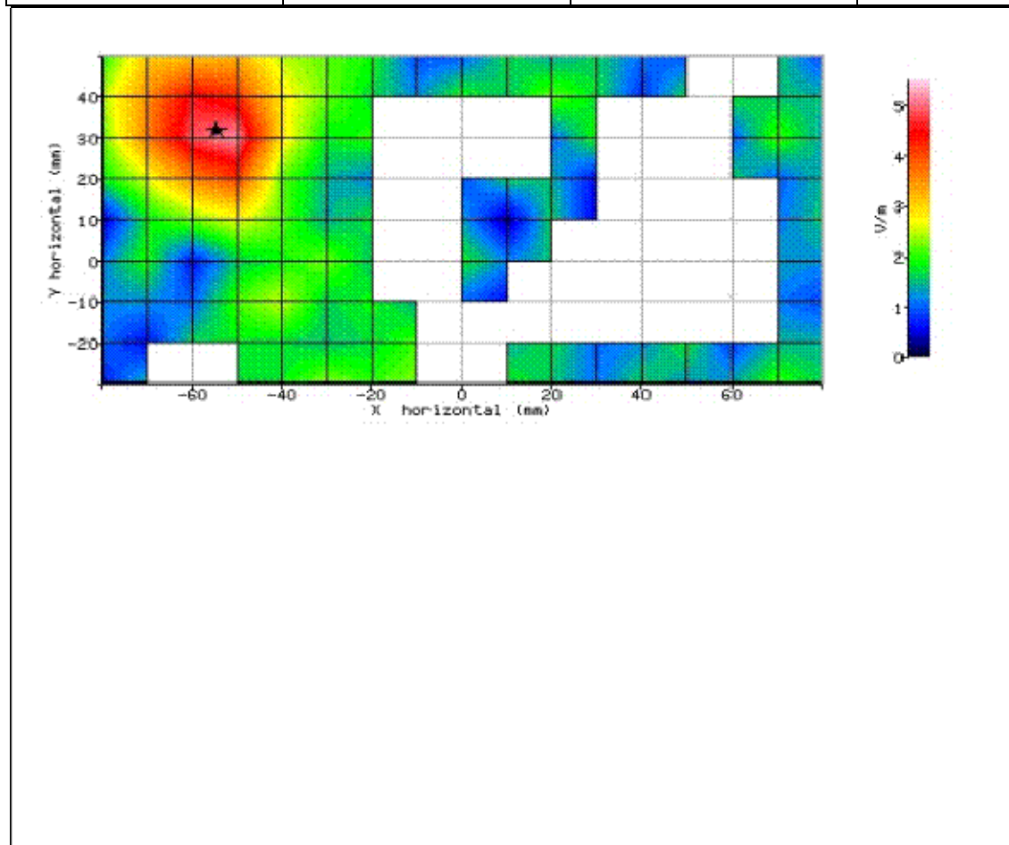
Figure 56: SAR Body Testing Results for the SHL22 Mobile Handset at 5260.0MHz.
