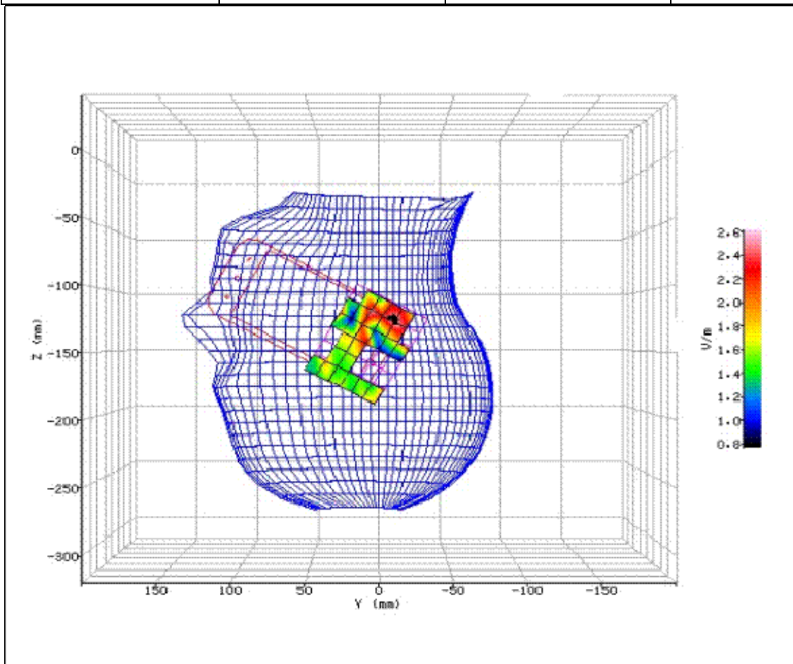
Figure 52: SAR Head Testing Results for the SHL22 Mobile Handset at 5260.0MHz.
