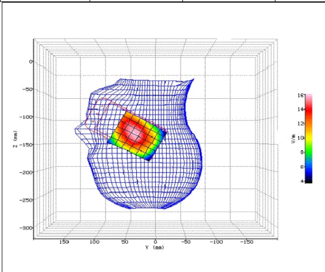
Figure 18: SAR Head Testing Results for the SHL22 Mobile Handset at 835MHz.
