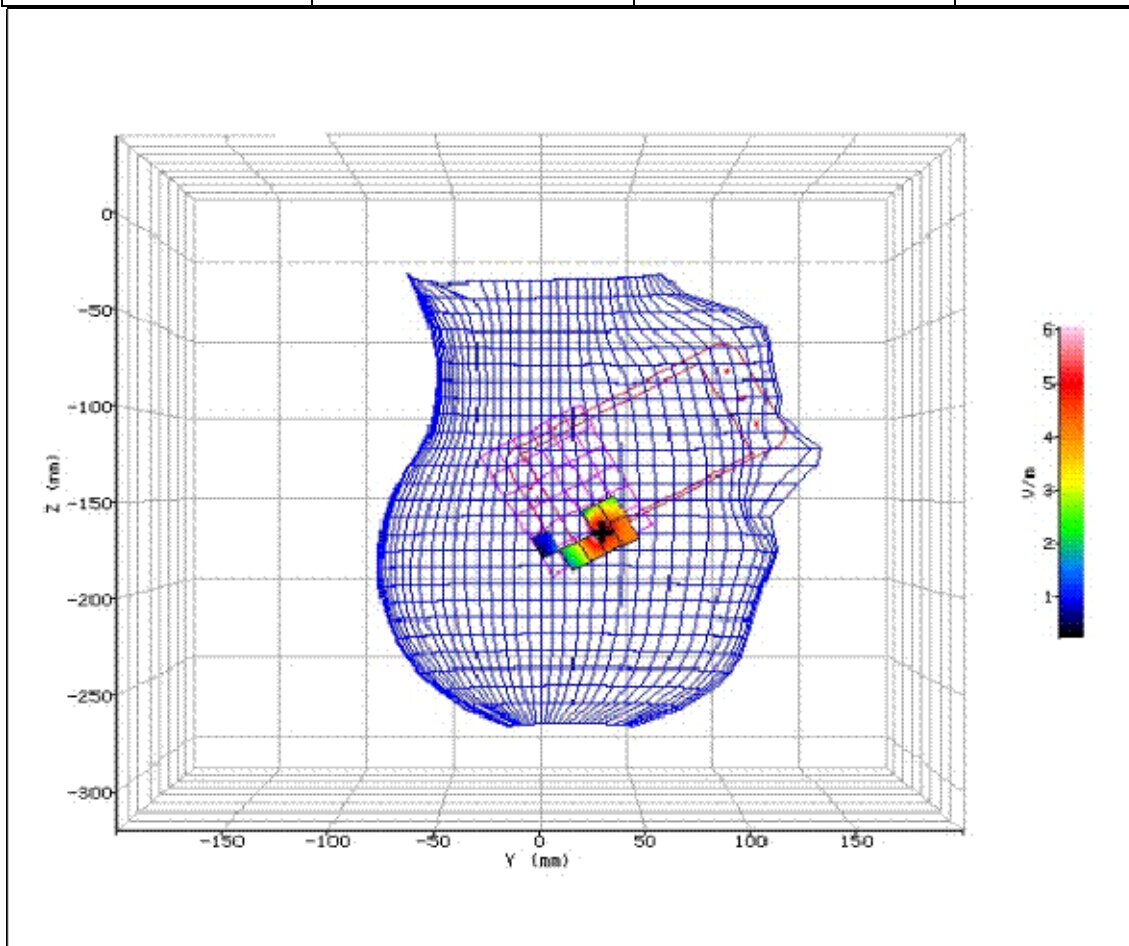
Figure 45: SAR Head Testing Results for the SHL22 Mobile Handset at 5240.0MHz.
