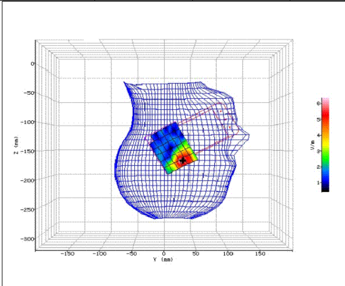
Figure 53: SAR Head Testing Results for the SHL22 Mobile Handset at 5260.0MHz.
