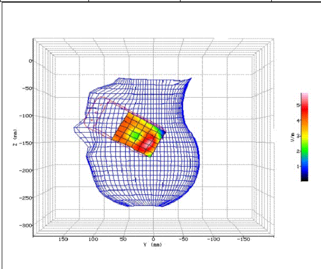
Figure 27: SAR Head Testing Results for the SHL22 Mobile Handset at 1880MHz.
