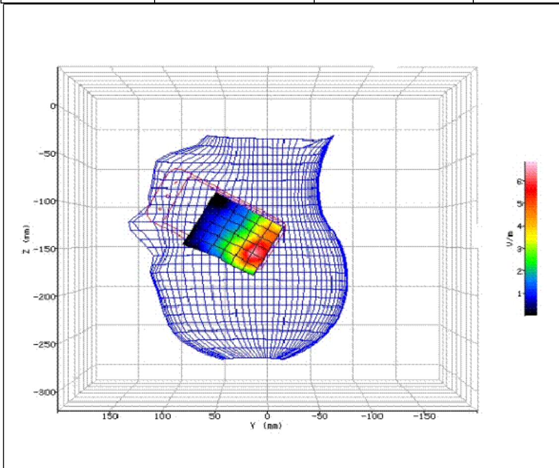
Figure 36: SAR Head Testing Results for the SHL22 Mobile Handset at 2437.0MHz.
