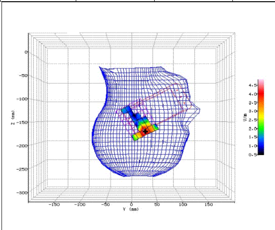
Figure 54: SAR Head Testing Results for the SHL22 Mobile Handset at 5260.0MHz.
