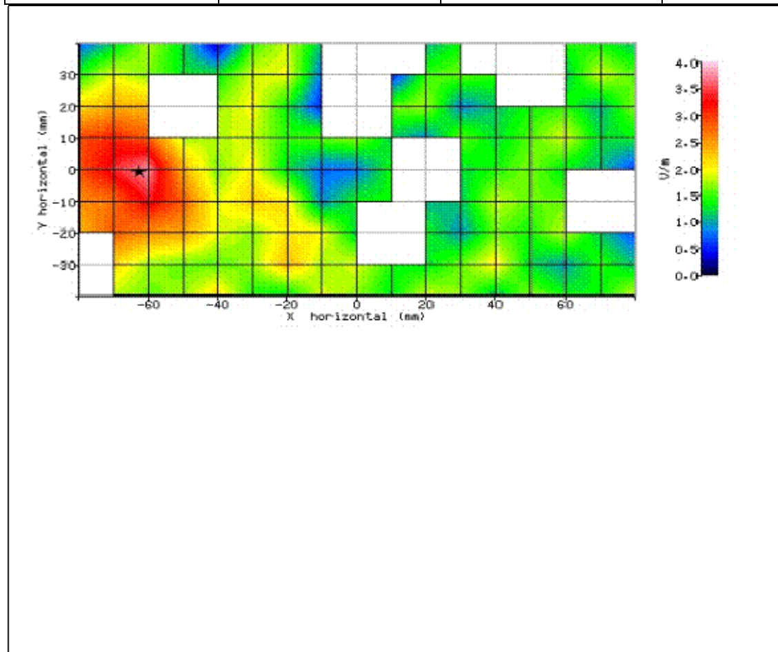
Figure 65: SAR Body Testing Results for the SHL22 Mobile Handset at 5580.0MHz.
