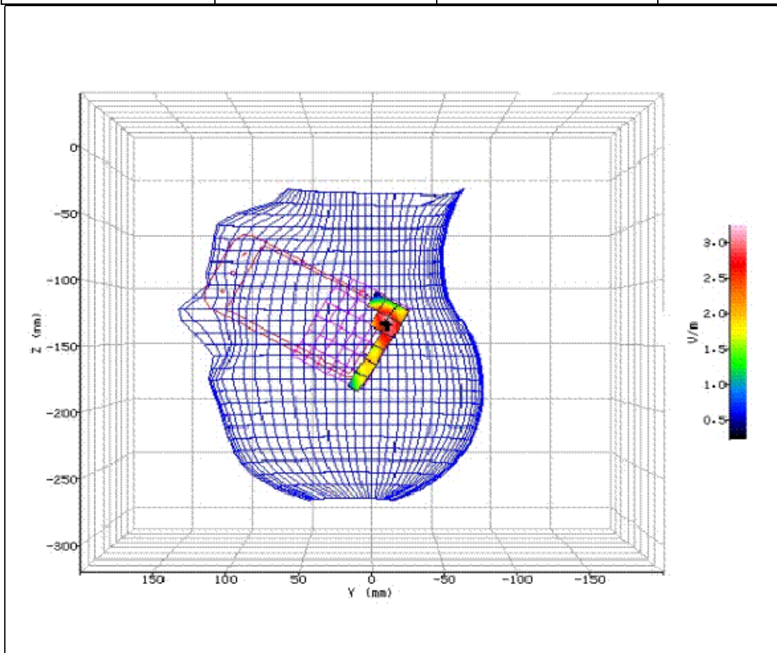
Figure 60: SAR Head Testing Results for the SHL22 Mobile Handset at 5580.0MHz.
