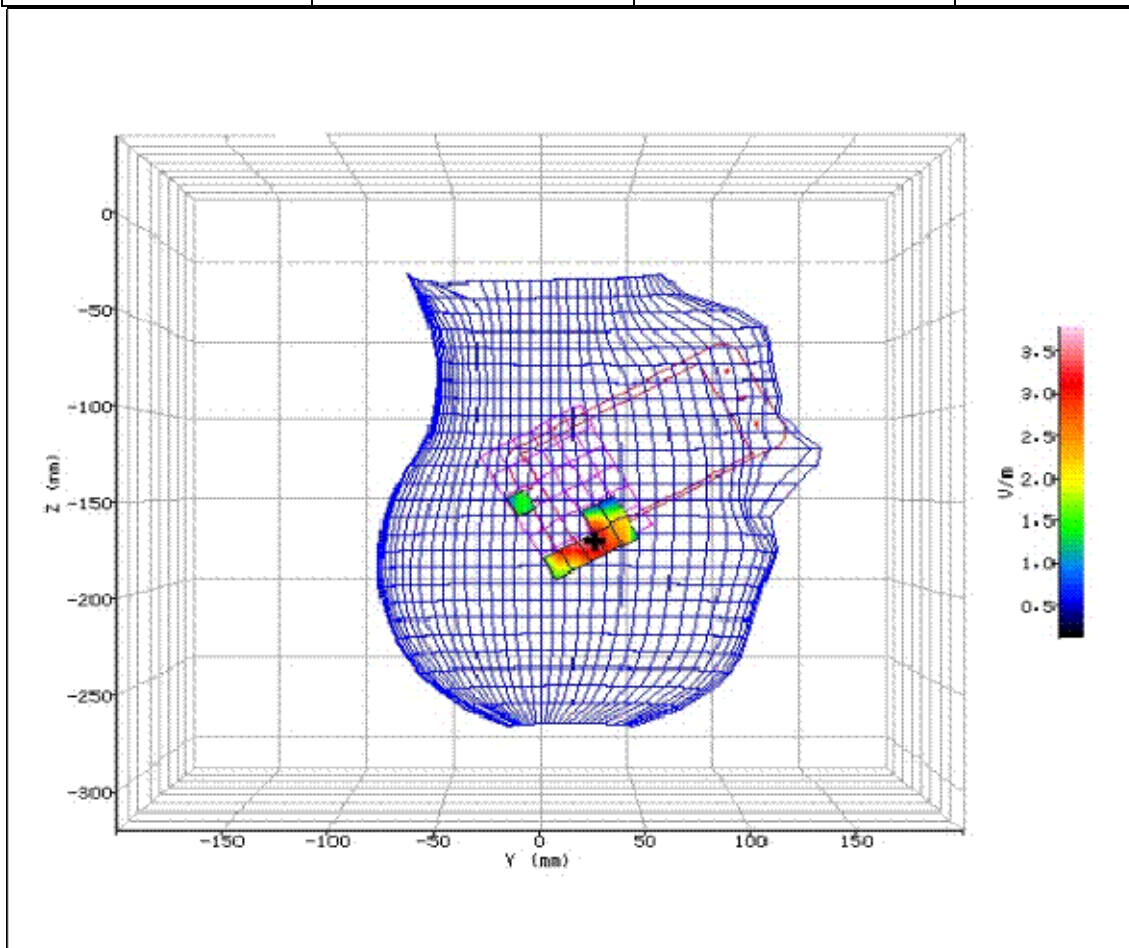
Figure 46: SAR Head Testing Results for the SHL22 Mobile Handset at 5240.0MHz.
