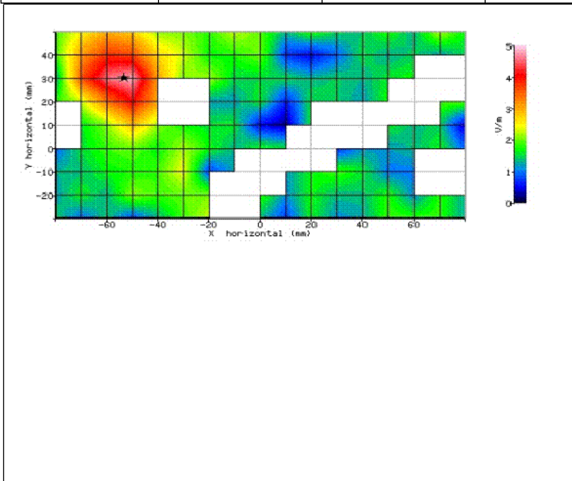
Figure 48: SAR Body Testing Results for the SHL22 Mobile Handset at 5240.0MHz.
