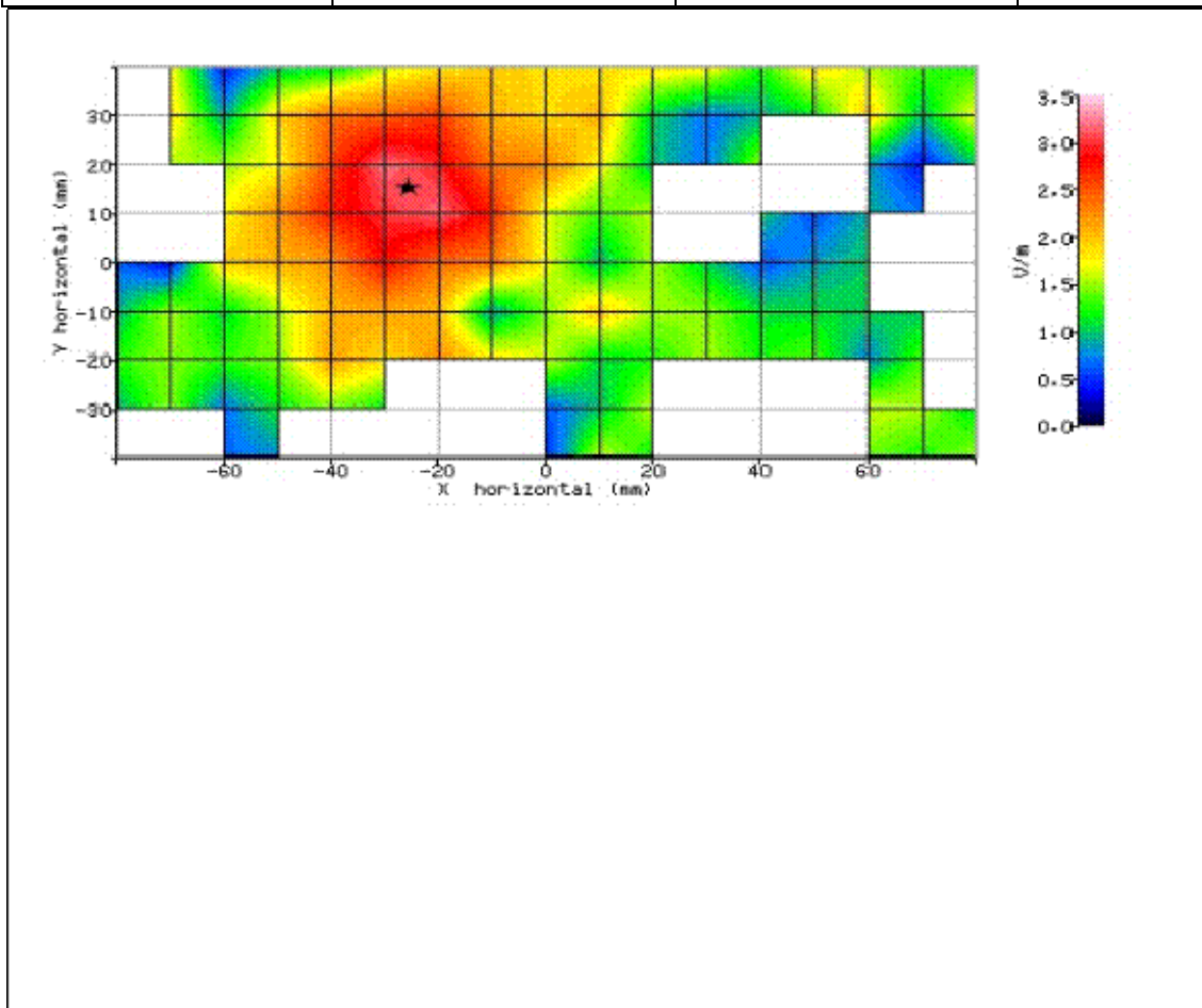
Figure 66: SAR Body Testing Results for the SHL22 Mobile Handset at 5580.0MHz.
