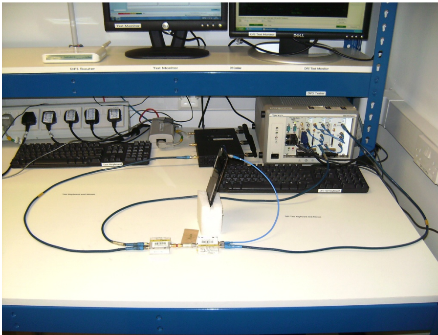
DFS Testing - Testing Set-Up
