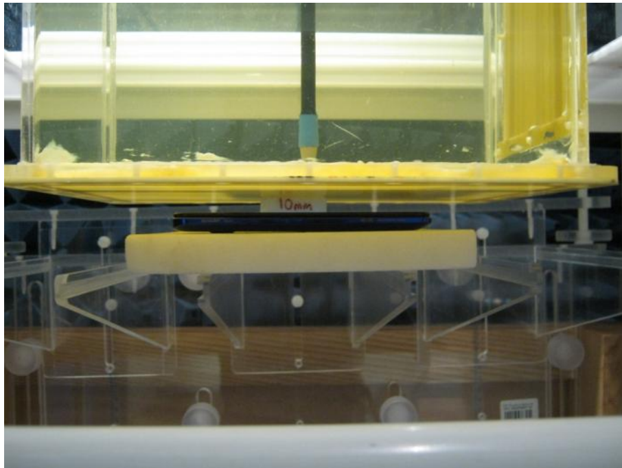
SAR - Front Face
