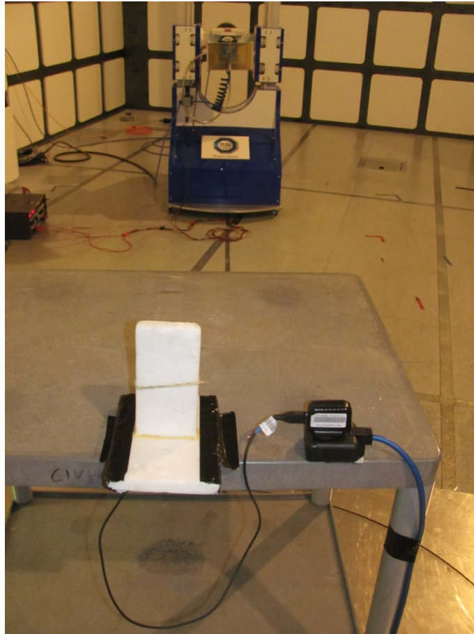
FCC Part 15.247 Radiated Emissions 1GHz-17GHz
