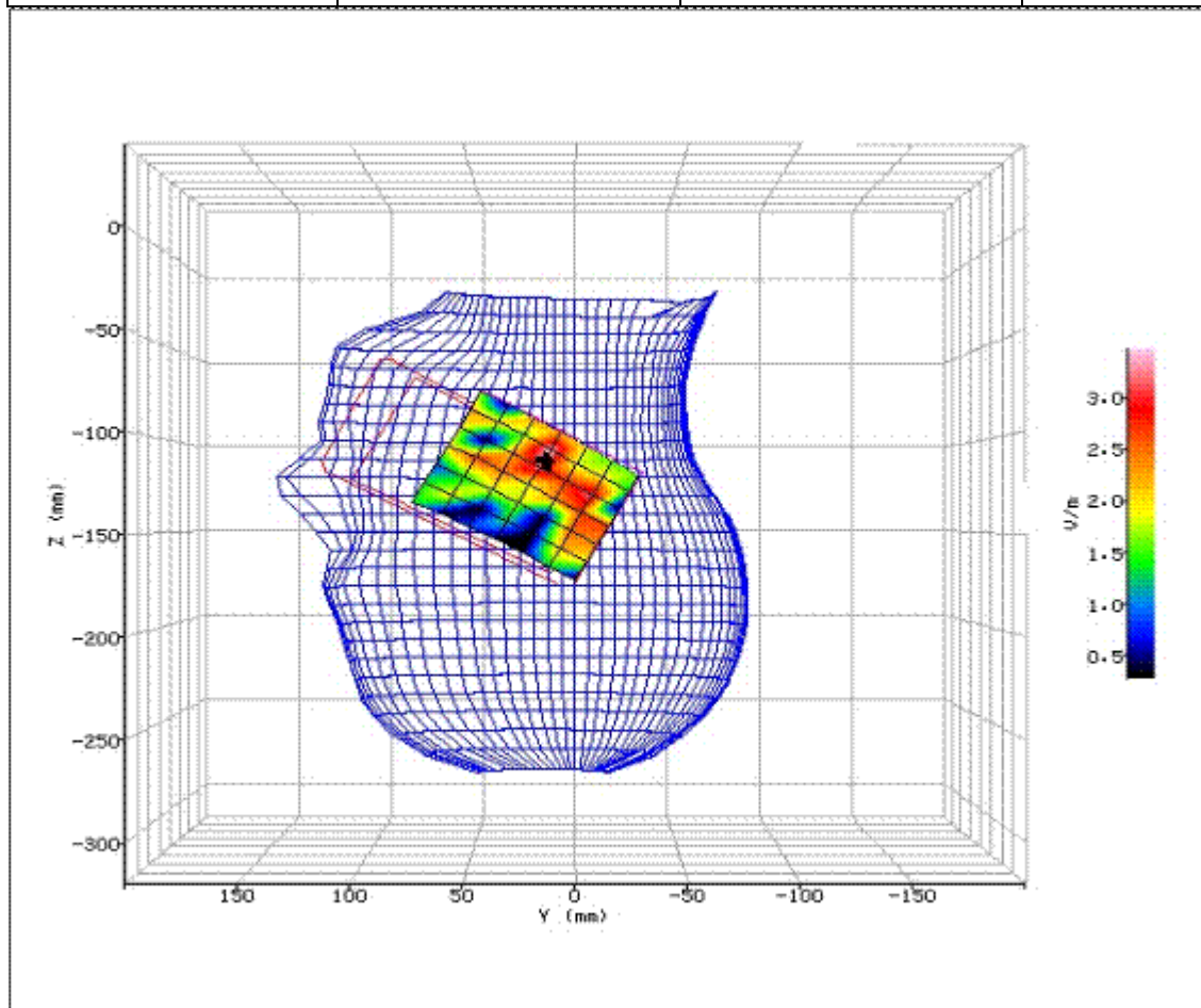
Figure 66: SAR Head Testing Results for the SHL23 Mobile Handset at 5520.0MHz. (NUA)
