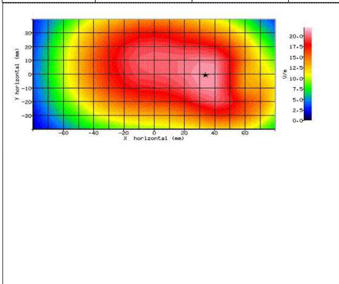
Figure 25: SAR Body Testing Results for the SHL23 Mobile Handset at 826.6MHz.
