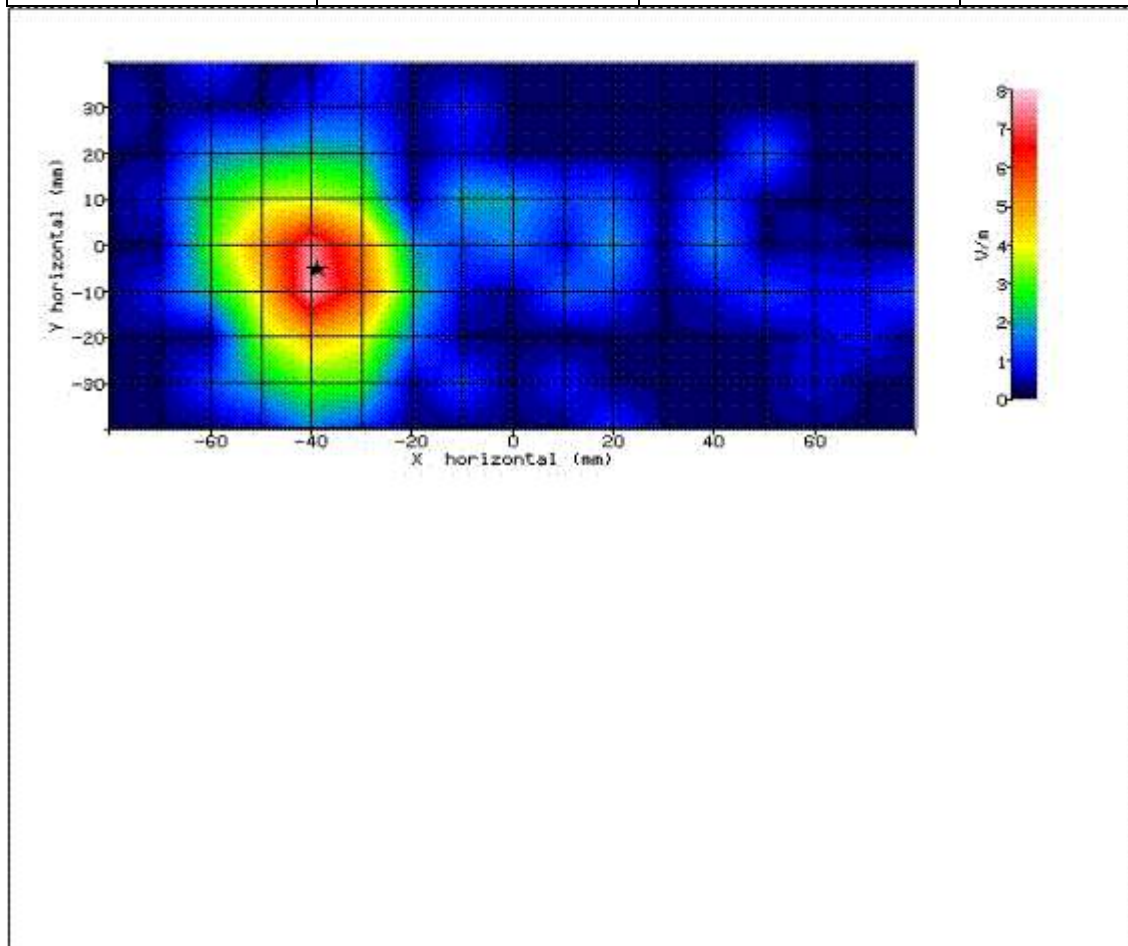
Figure 64: SAR Body Testing Results for the SHL23 Mobile Handset at 5280.0MHz. (NUA)
