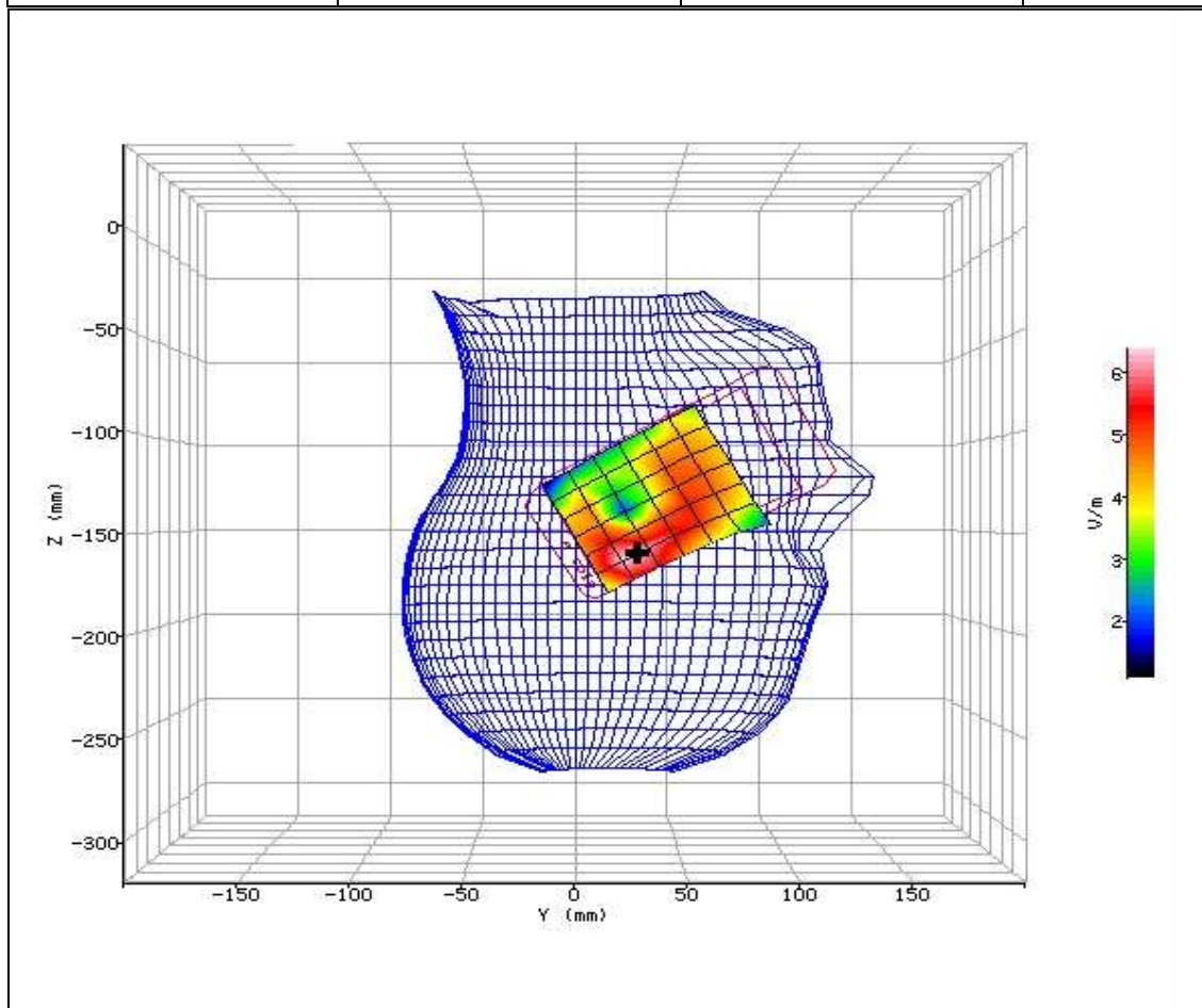
Figure 33: SAR Head Testing Results for the SHL23 Mobile Handset at 1909.8MHz.
