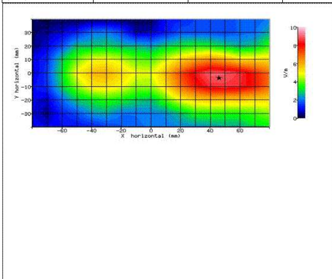
Figure 40: SAR Body Testing Results for the SHL23 Mobile Handset at 1880MHz.
