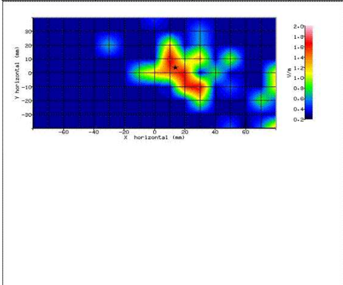
Figure 57: SAR Body Testing Results for the SHL23 Mobile Handset at 5240.0MHz. (NUA)
