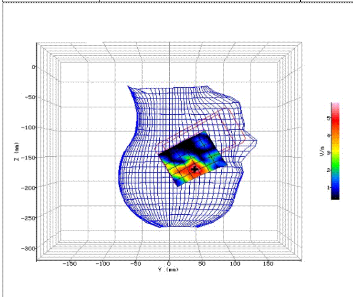
Figure 68: SAR Head Testing Results for the SHL23 Mobile Handset at 5520.0MHz. (NUA)
