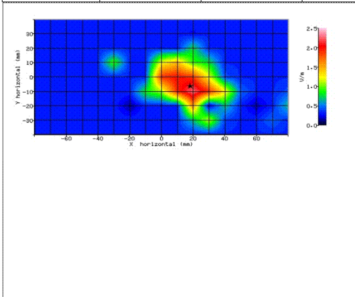
Figure 73: SAR Body Testing Results for the SHL23 Mobile Handset at 5520.0MHz. (NUA)
