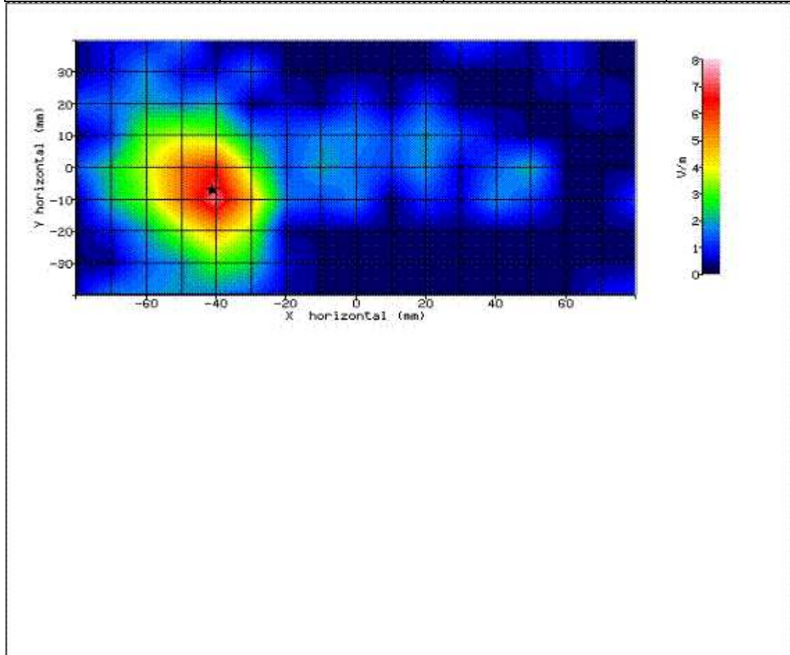
Figure 72: SAR Body Testing Results for the SHL23 Mobile Handset at 5520.0MHz. (NUA)
