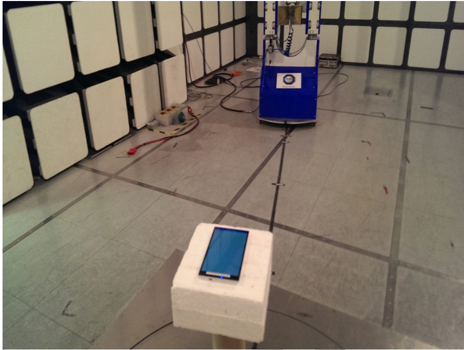
FCC Part 15.247 Radiated Emissions 1 GHz to 18 GHz
