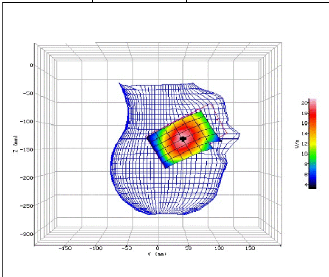
Figure 13: SAR Head Testing Results for the Sharp SHV32 Mobile Handset at 824.2MHz.
