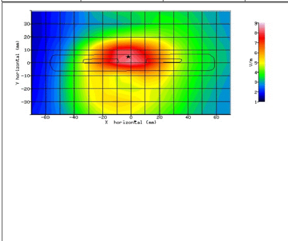
Figure 57: SAR Body Testing Results for the Sharp SHV32 Mobile Handset at 841.5MHz.
