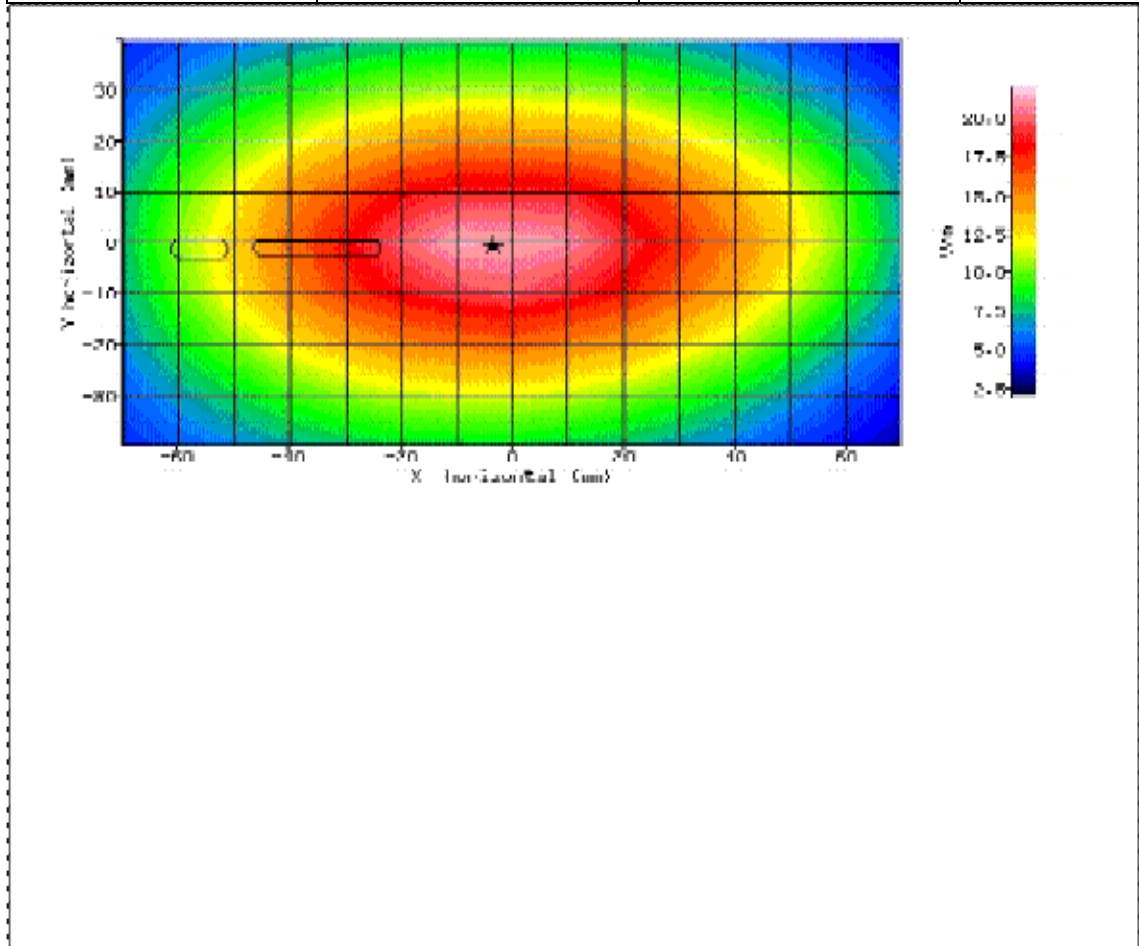
Figure 16: SAR Body Testing Results for the Sharp SHV32 Mobile Handset at 824.2MHz.
