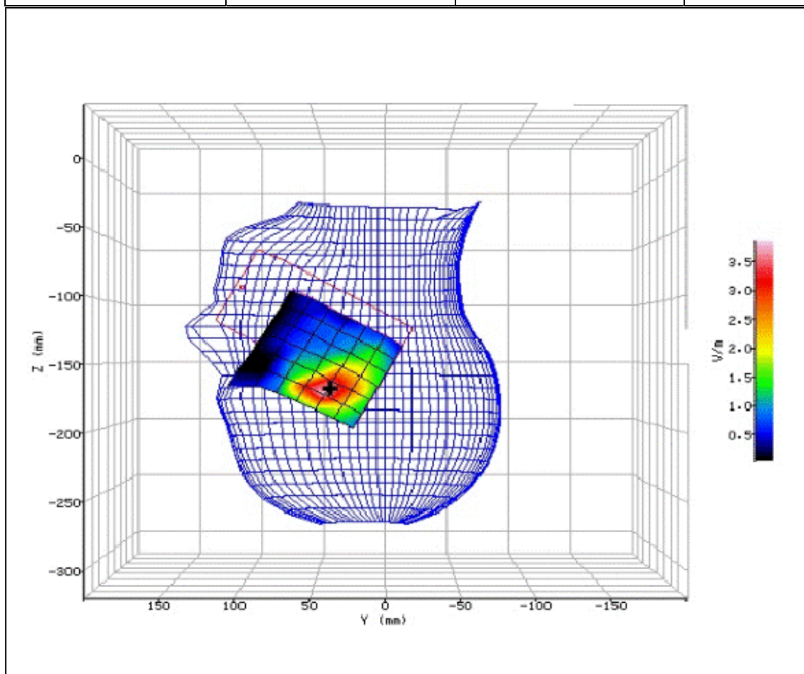
Figure 119: SAR Head Testing Results for the Sharp SHV32 Mobile Handset at 2437.0MHz.
