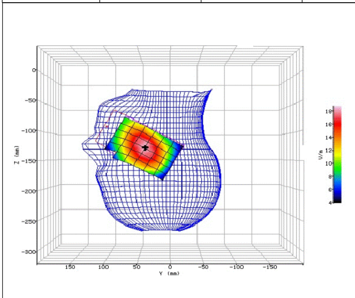
Figure 11: SAR Head Testing Results for the Sharp SHV32 Mobile Handset at 824.2MHz.
