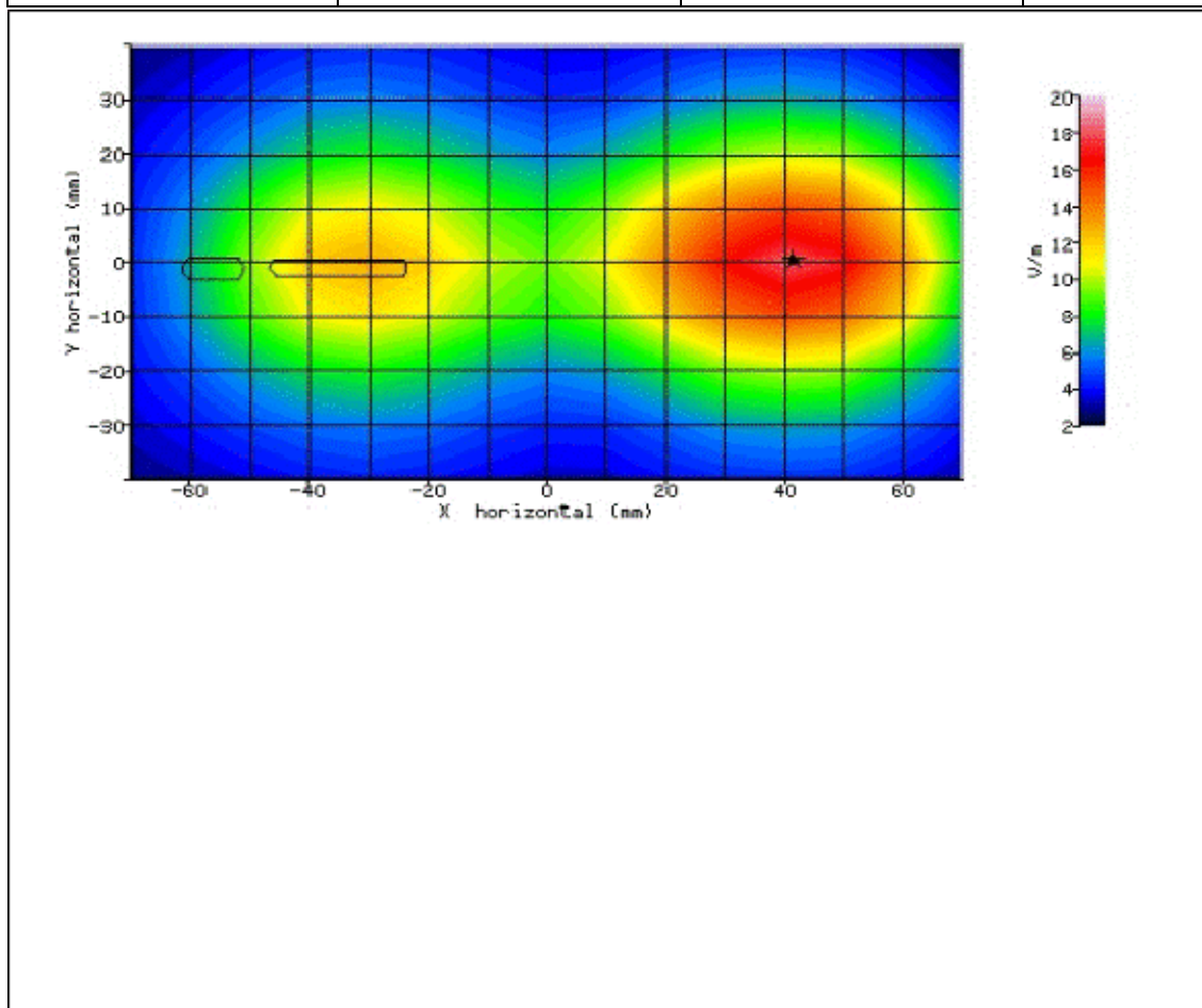
Figure 94: SAR Body Testing Results for the Sharp SHV32 Mobile Handset at 1880.0MHz.
