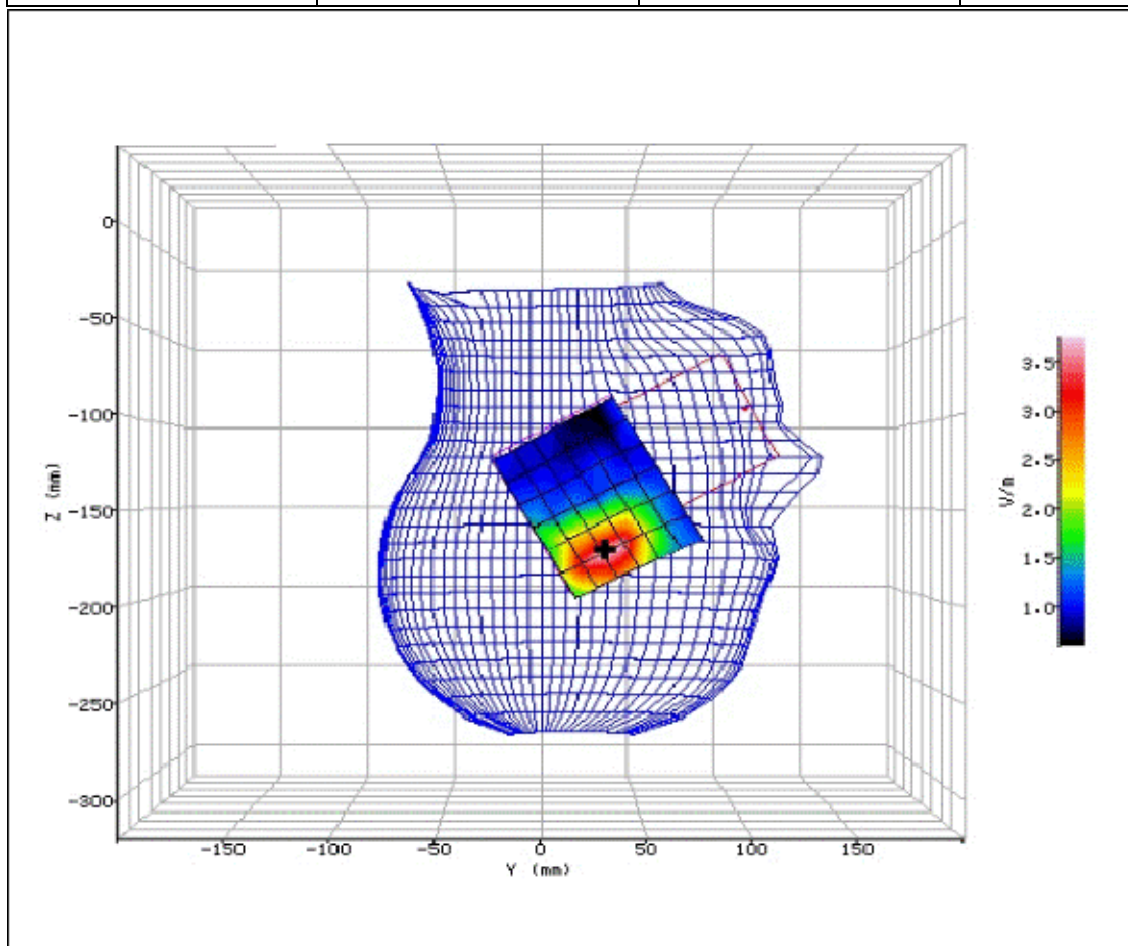
Figure 113: SAR Head Testing Results for the Sharp SHV32 Mobile Handset at 2437.0MHz.
