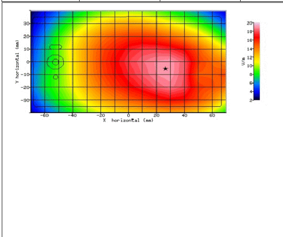
Figure 44: SAR Body Testing Results for the Sharp SHV32 Mobile Handset at 829.0MHz.
