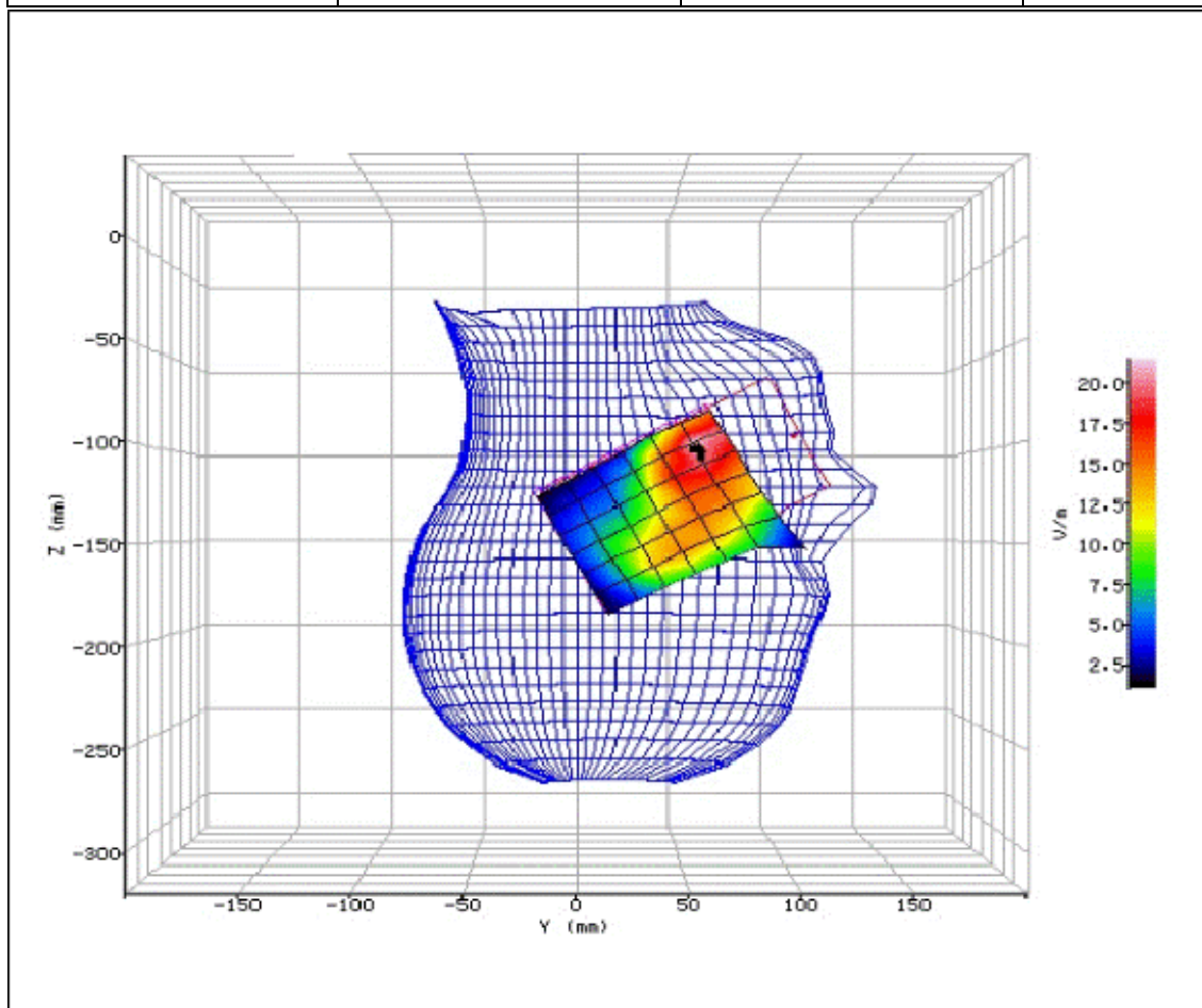
Figure 86: SAR Head Testing Results for the Sharp SHV32 Mobile Handset at 1880.0MHz.
