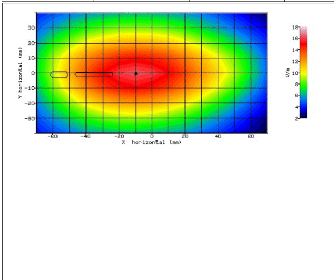
Figure 50: SAR Body Testing Results for the Sharp SHV32 Mobile Handset at 821.5MHz.
