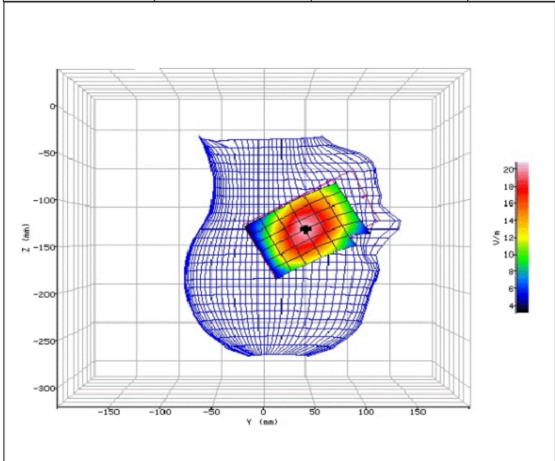
Figure 13: SAR Head Testing Results for the Sharp SHV32 Mobile Handset at 824.2MHz.
