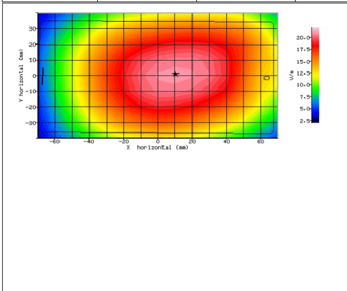
Figure 48: SAR Body Testing Results for the Sharp SHV32 Mobile Handset at 821.5MHz.
