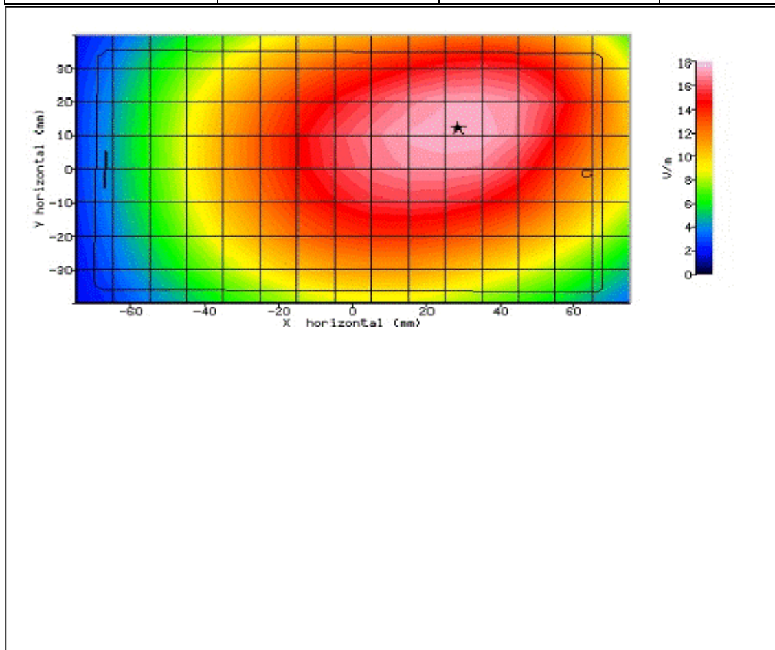
Figure 33: SAR Body Testing Results for the Sharp SHV32 Mobile Handset at 711.0MHz.
