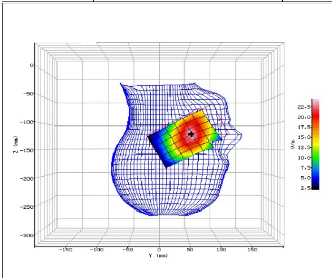
Figure 21: SAR Head Testing Results for the Sharp SHV32 Mobile Handset at 826.4MHz.
