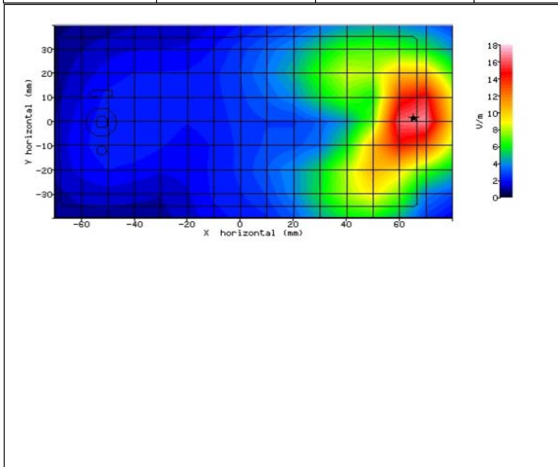
Figure 63: SAR Body Testing Results for the SHV32 Mobile Handset at 2636.5MHz.
