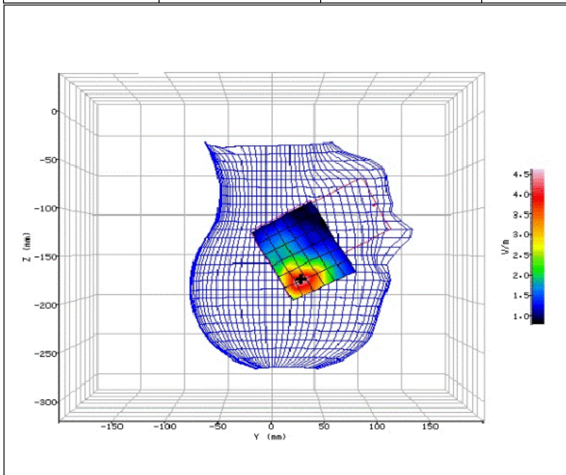
Figure 99: SAR Head Testing Results for the Sharp SHV32 Mobile Handset at 2437.0MHz.
