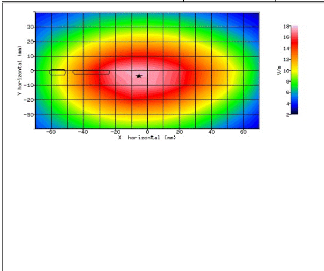
Figure 40: SAR Body Testing Results for the Sharp SHV32 Mobile Handset at 836.5MHz.
