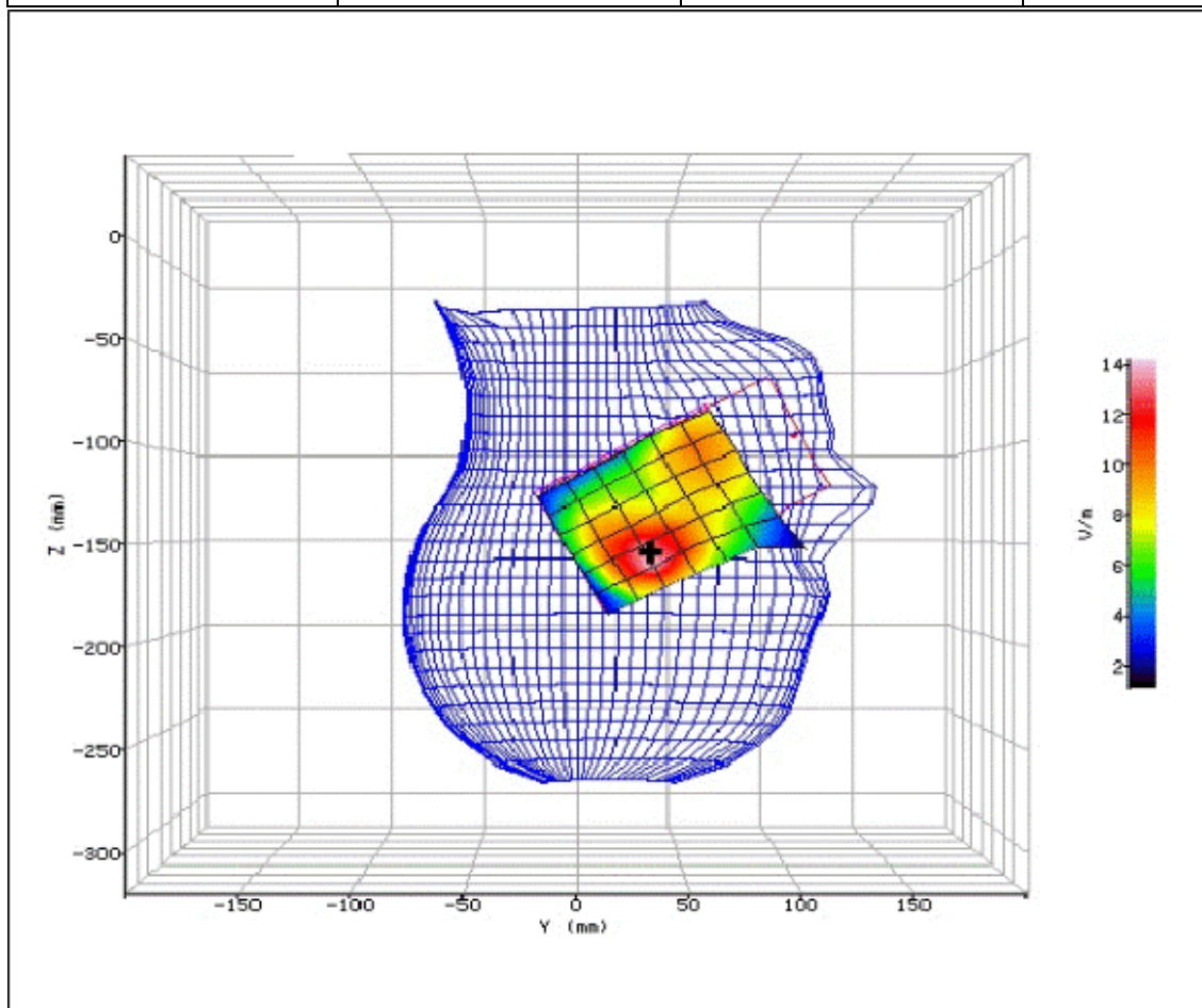
Figure 91: SAR Head Testing Results for the Sharp SHV32 Mobile Handset at 1880.0MHz.
