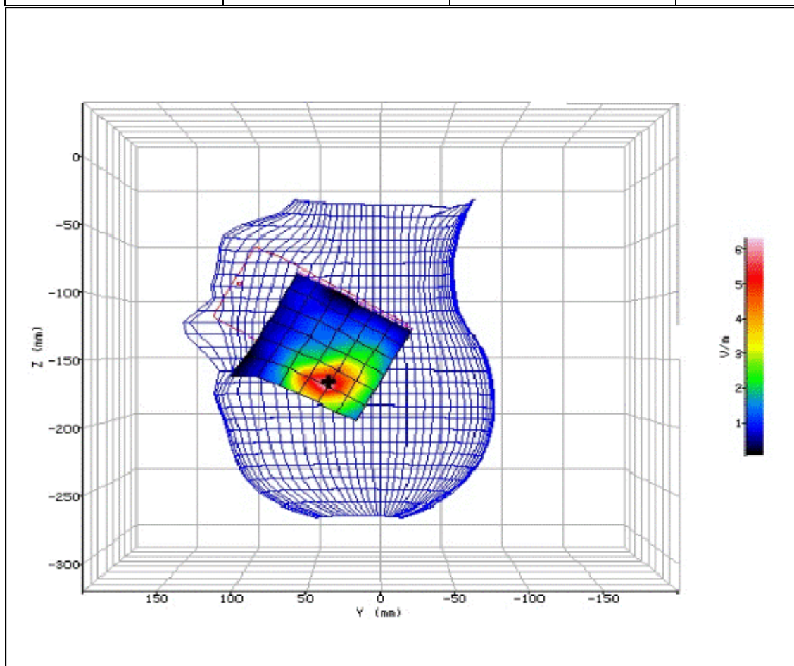
Figure 104: SAR Head Testing Results for the Sharp SHV32 Mobile Handset at 2437.0MHz.
