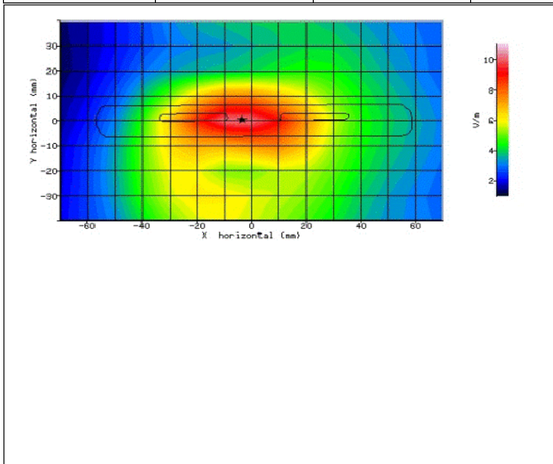
Figure 27: SAR Body Testing Results for the Sharp SHV32 Mobile Handset at 826.4MHz.
