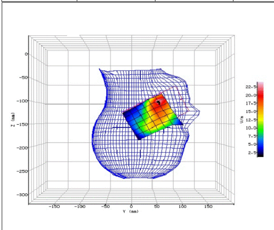
Figure 90: SAR Head Testing Results for the Sharp SHV32 Mobile Handset at 1880.0MHz.
