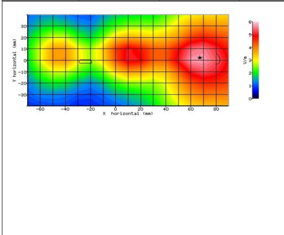
Figure 65: SAR Body Testing Results for the SHV32 Mobile Handset at 2593.0MHz.
