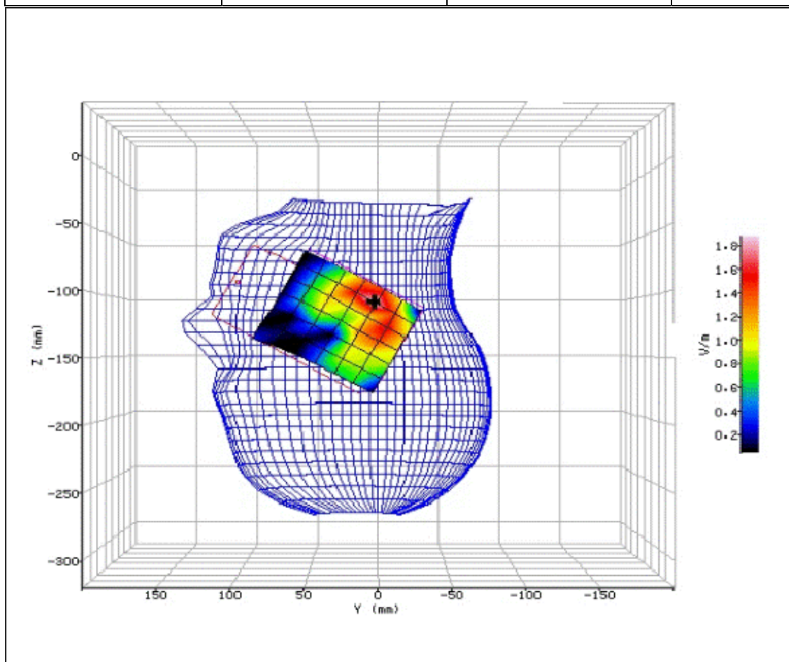
Figure 111: SAR Head Testing Results for the Sharp SHV32 Mobile Handset at 2437.0MHz.
