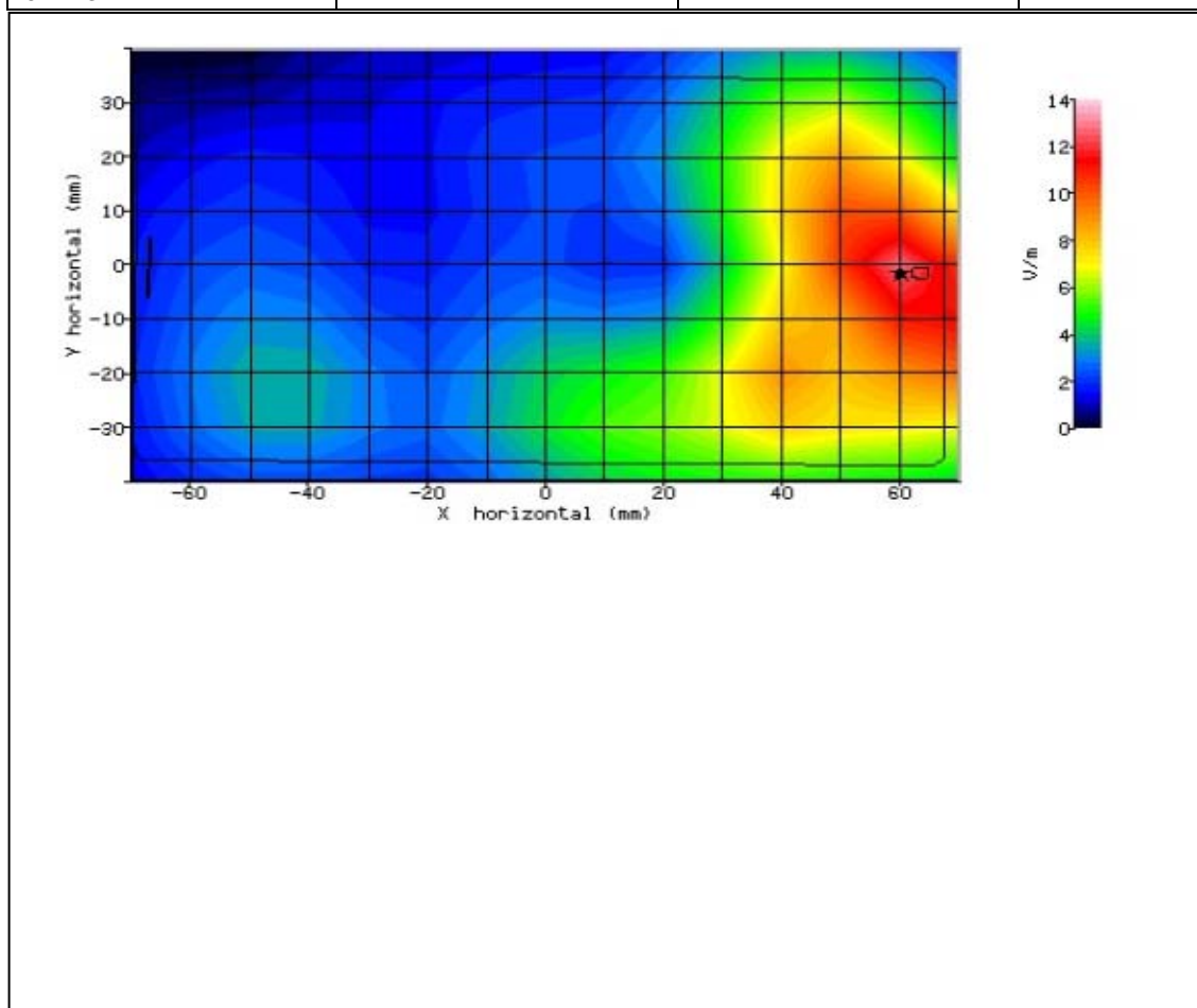
Figure 58: SAR Body Testing Results for the SHV32 Mobile Handset at 2593.0MHz.
