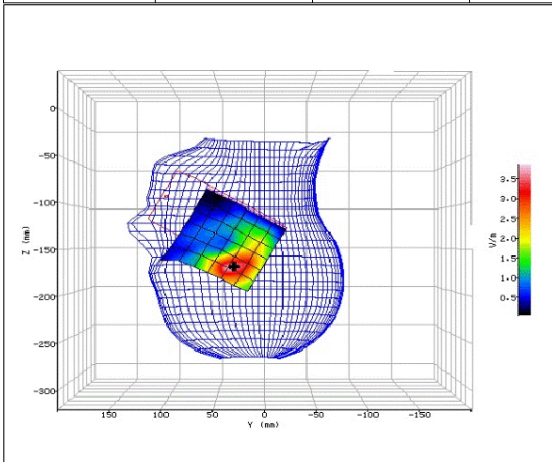
Figure 105: SAR Head Testing Results for the Sharp SHV32 Mobile Handset at 2437.0MHz.
