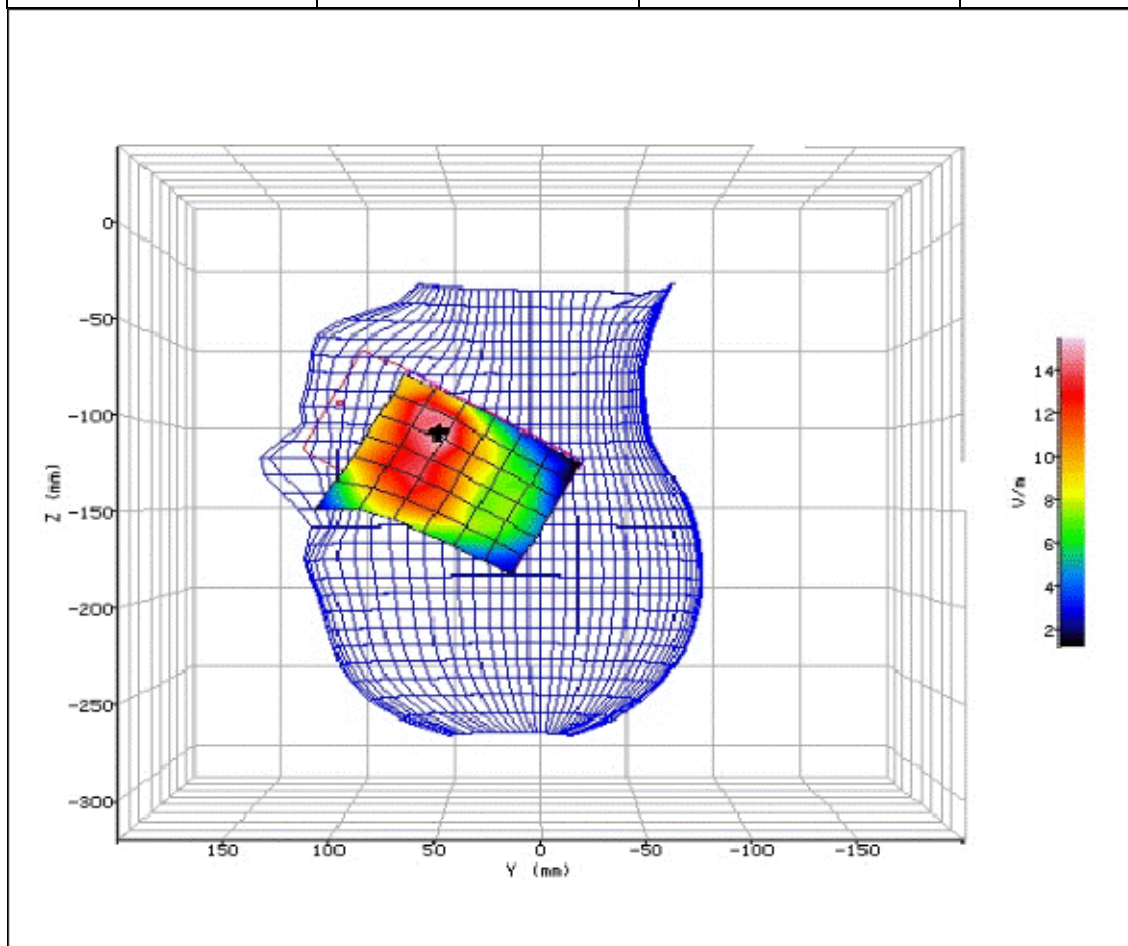
Figure 88: SAR Head Testing Results for the Sharp SHV32 Mobile Handset at 1880.0MHz.
