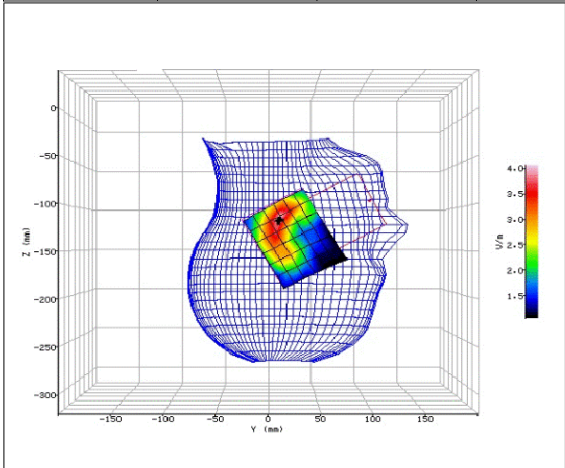
Figure 106: SAR Head Testing Results for the Sharp SHV32 Mobile Handset at 2437.0MHz.
