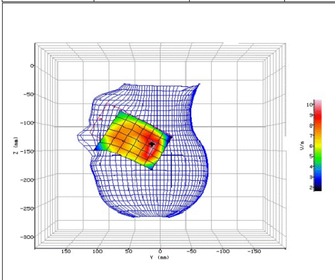
Figure 89: SAR Head Testing Results for the Sharp SHV32 Mobile Handset at 1880.0MHz.
