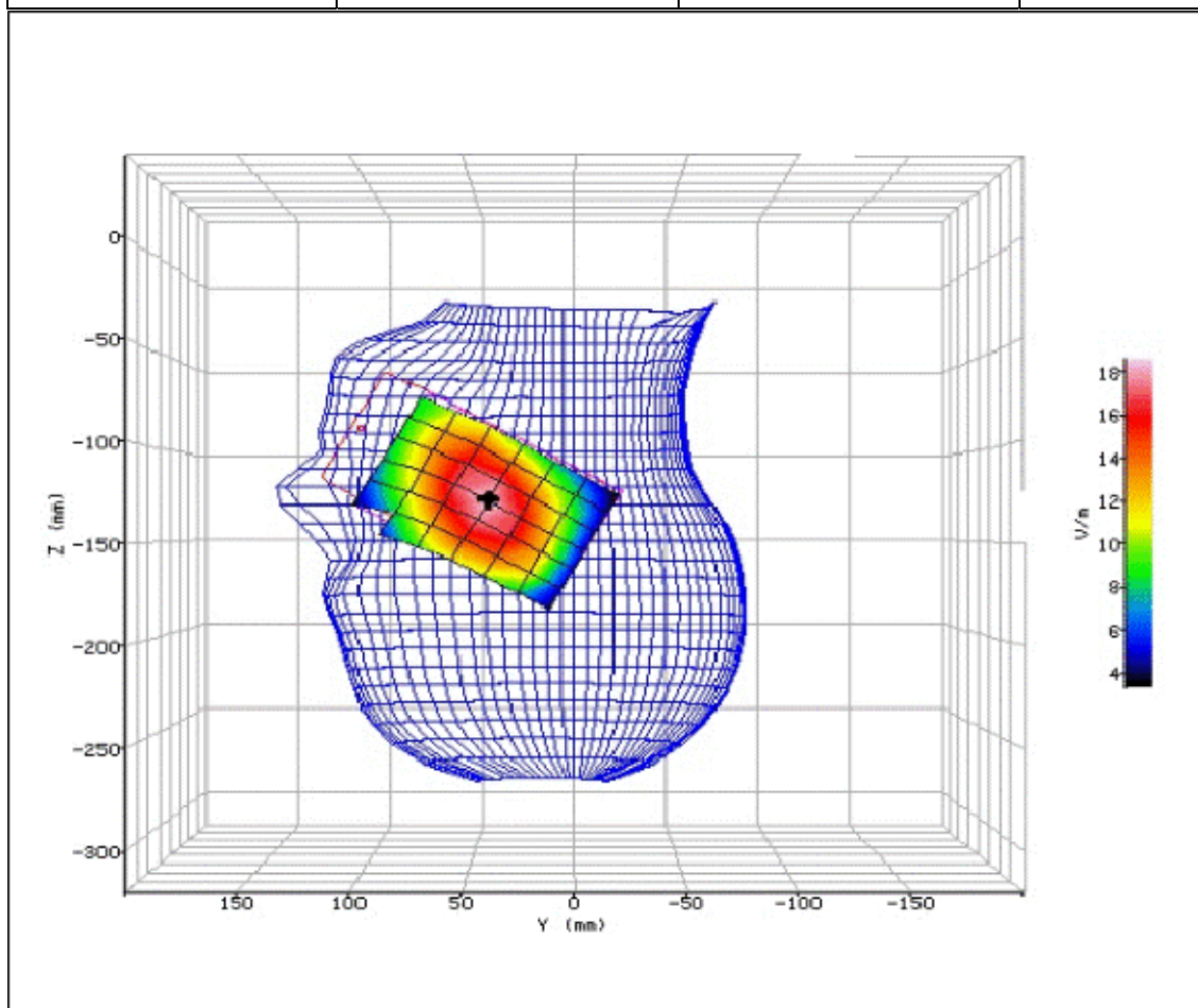
Figure 20: SAR Head Testing Results for the Sharp SHV32 Mobile Handset at 826.4MHz.
