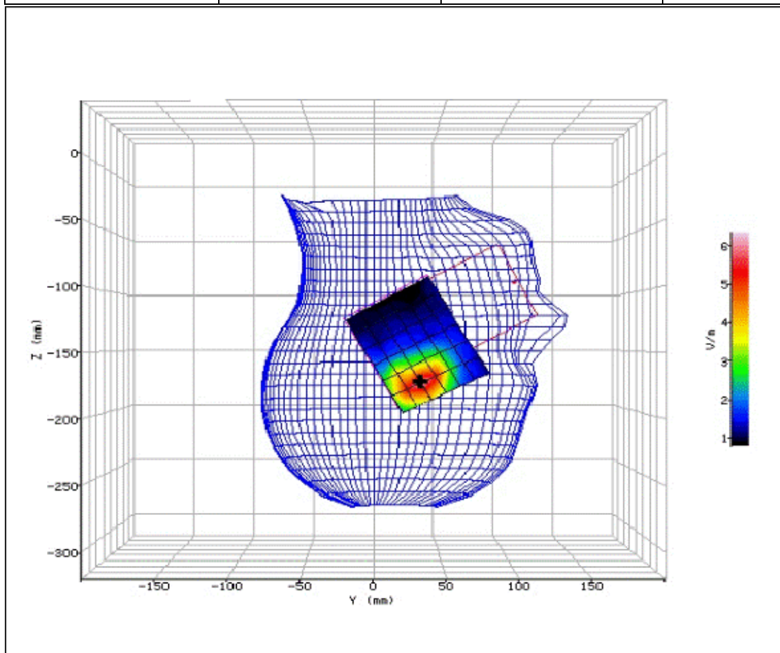
Figure 98: SAR Head Testing Results for the Sharp SHV32 Mobile Handset at 2437.0MHz.
