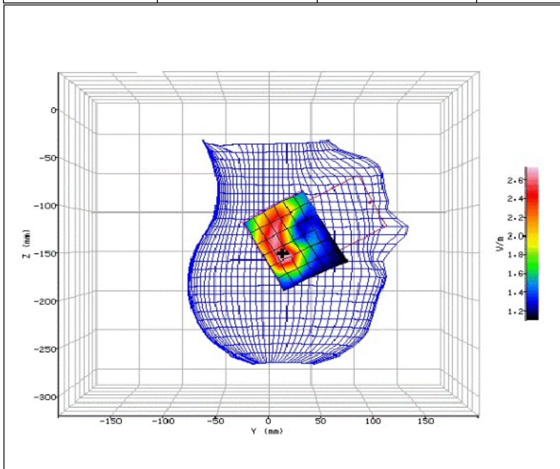
Figure 107: SAR Head Testing Results for the Sharp SHV32 Mobile Handset at 2437.0MHz.
