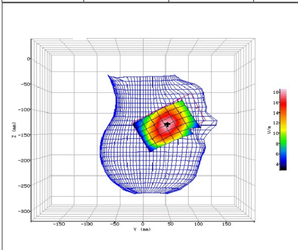
Figure 9: SAR Head Testing Results for the Sharp SHV32 Mobile Handset at 824.2MHz.
