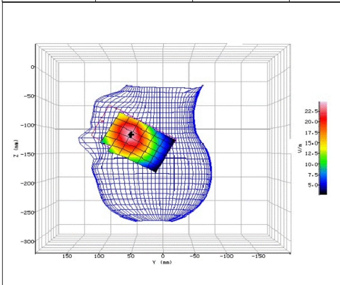
Figure 10: SAR Head Testing Results for the Sharp SHV32 Mobile Handset at 824.2MHz.
