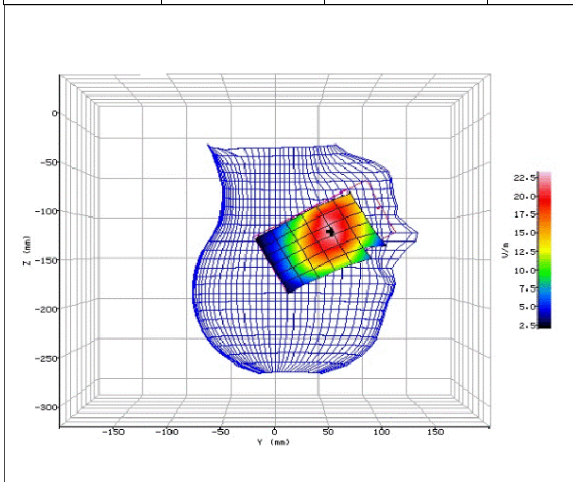
Figure 8: SAR Head Testing Results for the Sharp SHV32 Mobile Handset at 824.2MHz.
