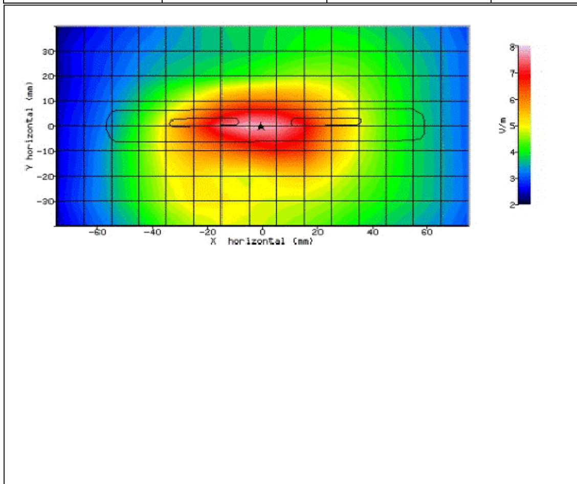
Figure 32: SAR Body Testing Results for the Sharp SHV32 Mobile Handset at 709.0MHz.
