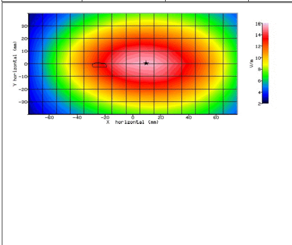
Figure 31: SAR Body Testing Results for the Sharp SHV32 Mobile Handset at 709.0MHz.
