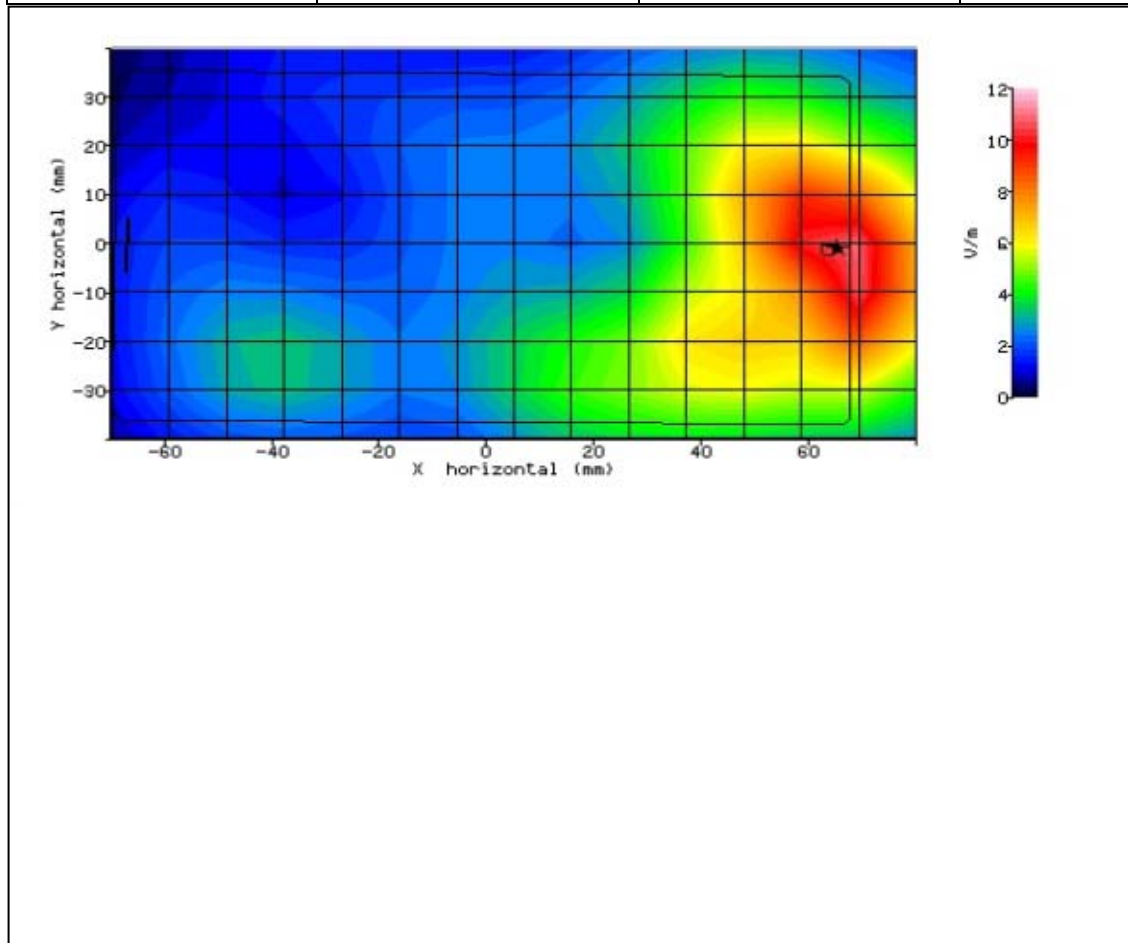
Figure 71: SAR Body Testing Results for the SHV32 Mobile Handset at 2506.0MHz.
