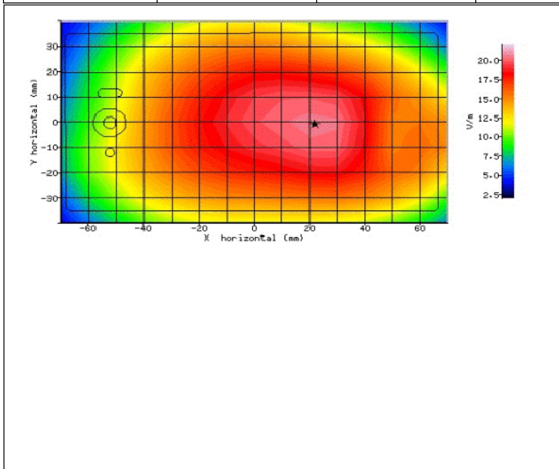
Figure 49: SAR Body Testing Results for the Sharp SHV32 Mobile Handset at 821.5MHz.
