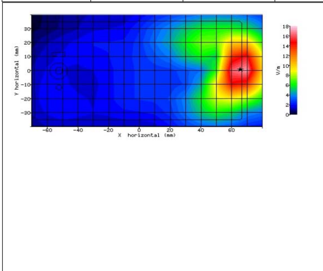
Figure 62: SAR Body Testing Results for the SHV32 Mobile Handset at 2549.5MHz.
