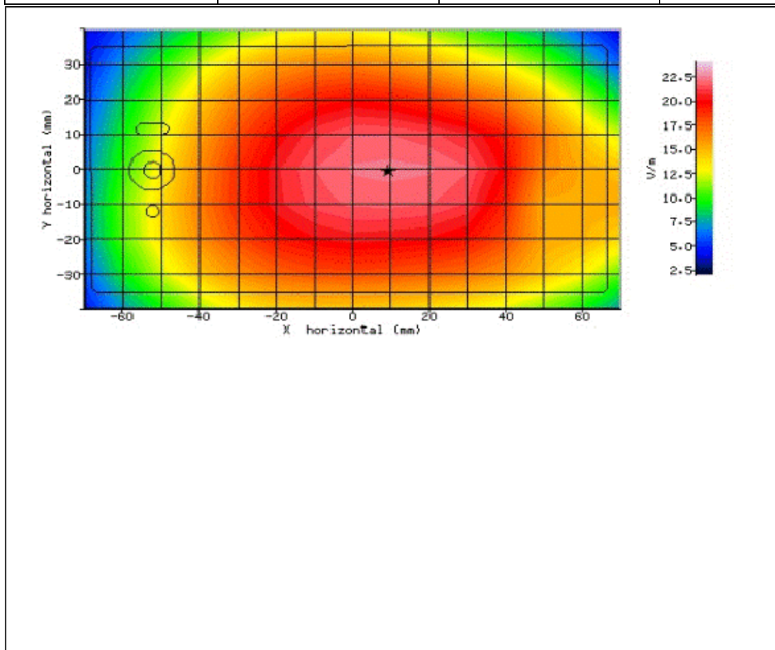
Figure 24: SAR Body Testing Results for the Sharp SHV32 Mobile Handset at 826.4MHz.
