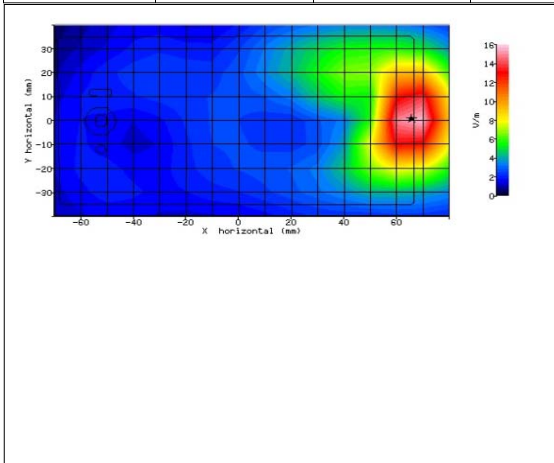
Figure 61: SAR Body Testing Results for the SHV32 Mobile Handset at 2506.0MHz.
