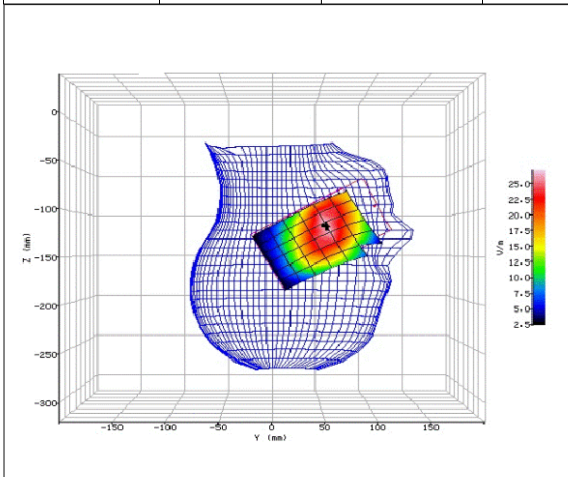
Figure 12: SAR Head Testing Results for the Sharp SHV32 Mobile Handset at 824.2MHz.
