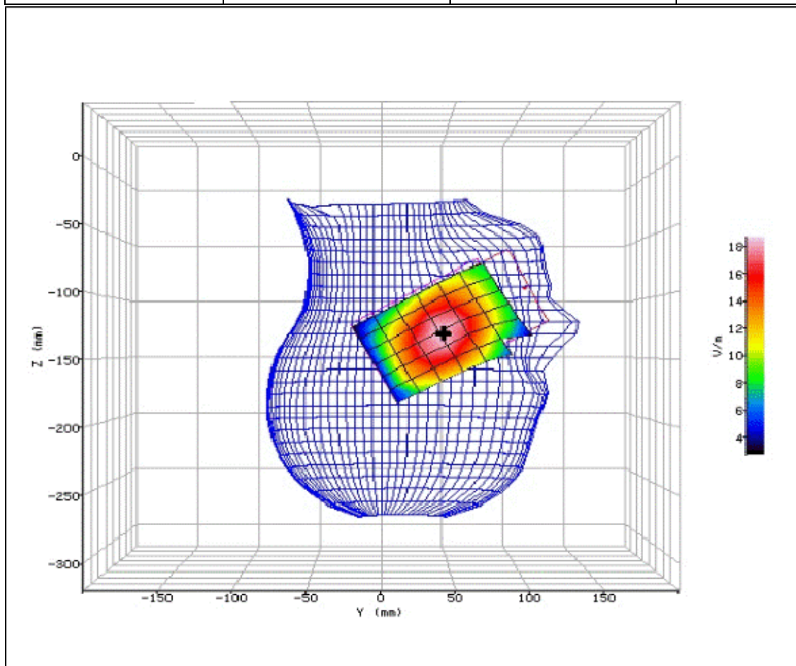
Figure 22: SAR Head Testing Results for the Sharp SHV32 Mobile Handset at 826.4MHz.
