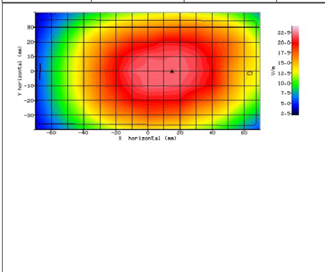
Figure 38: SAR Body Testing Results for the Sharp SHV32 Mobile Handset at 836.5MHz.
