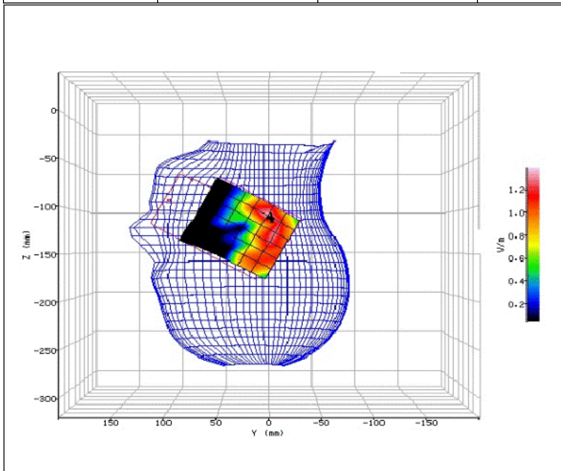
Figure 112: SAR Head Testing Results for the Sharp SHV32 Mobile Handset at 2437.0MHz.
