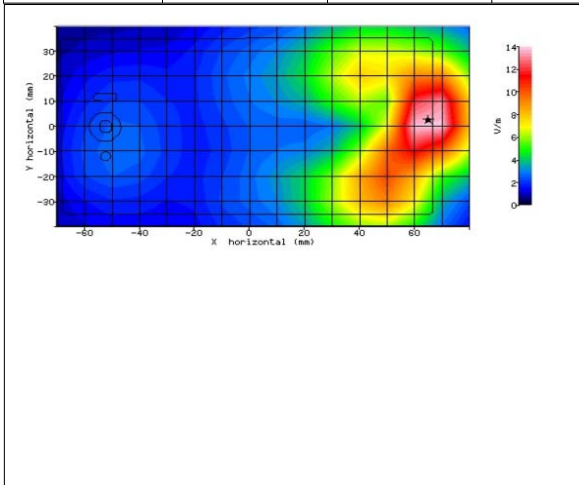
Figure 73: SAR Body Testing Results for the SHV32 Mobile Handset at 2680.0MHz.
