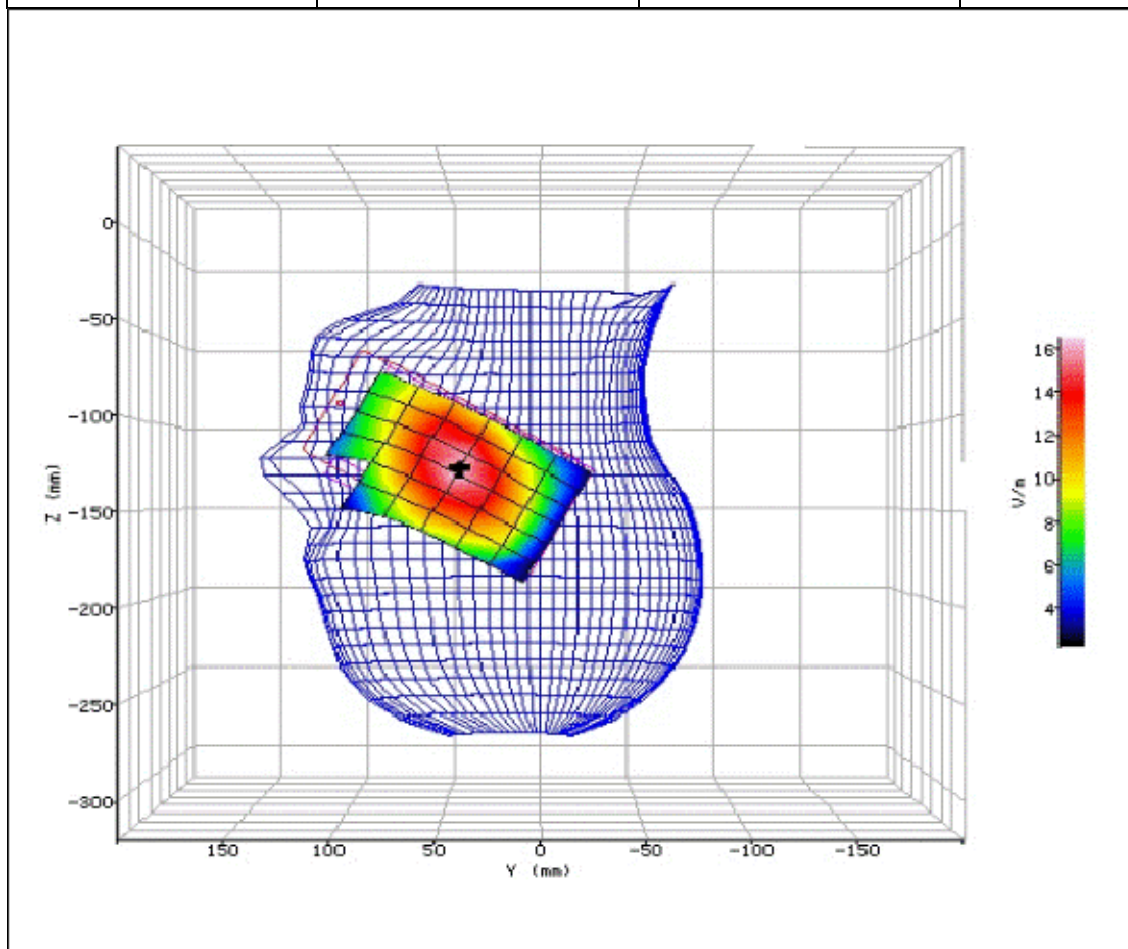
Figure 7: SAR Head Testing Results for the Sharp SHV32 Mobile Handset at 824.2MHz.
