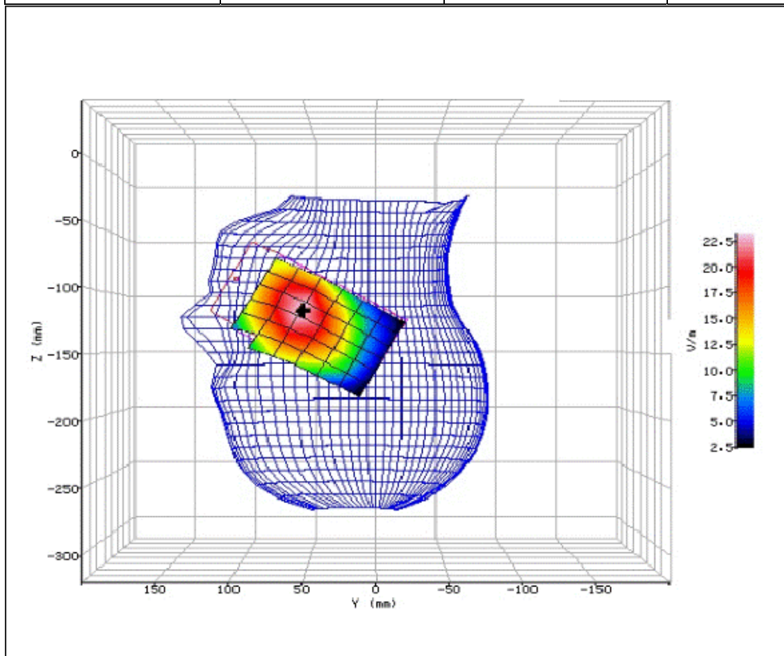
Figure 19: SAR Head Testing Results for the Sharp SHV32 Mobile Handset at 826.4MHz.
