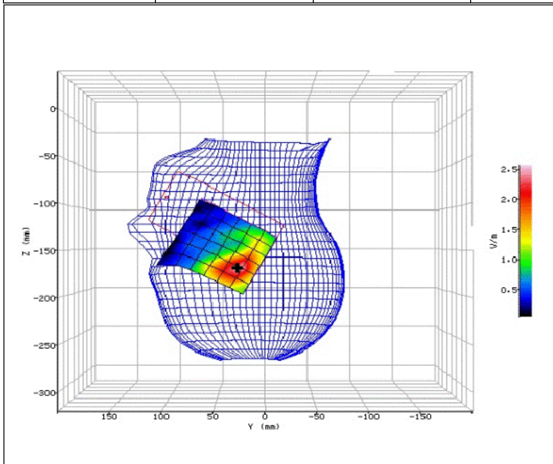
Figure 120: SAR Head Testing Results for the Sharp SHV32 Mobile Handset at 2437.0MHz.
