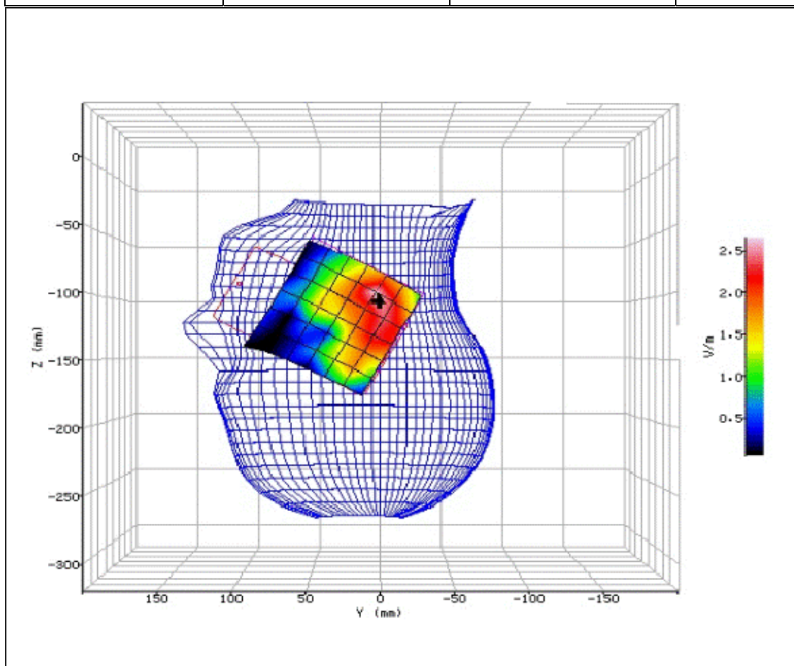
Figure 96: SAR Head Testing Results for the Sharp SHV32 Mobile Handset at 2437.0MHz.
