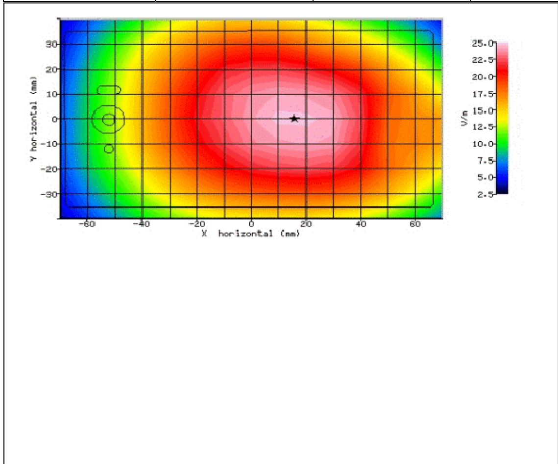
Figure 15: SAR Body Testing Results for the Sharp SHV32 Mobile Handset at 824.2MHz.
