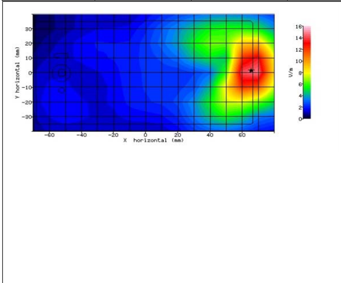
Figure 75: SAR Body Testing Results for the SHV32 Mobile Handset at 2549.5MHz.
