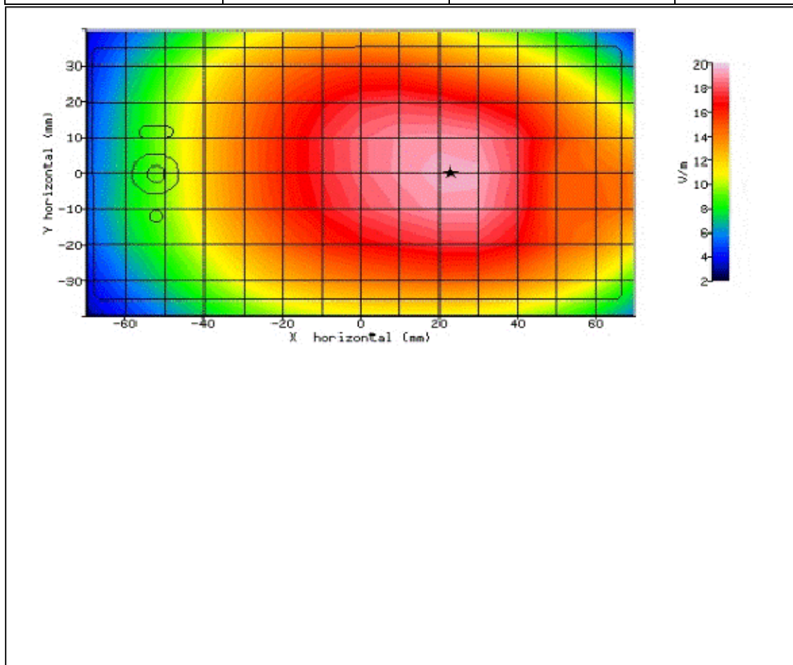
Figure 54: SAR Body Testing Results for the Sharp SHV32 Mobile Handset at 841.5MHz.
