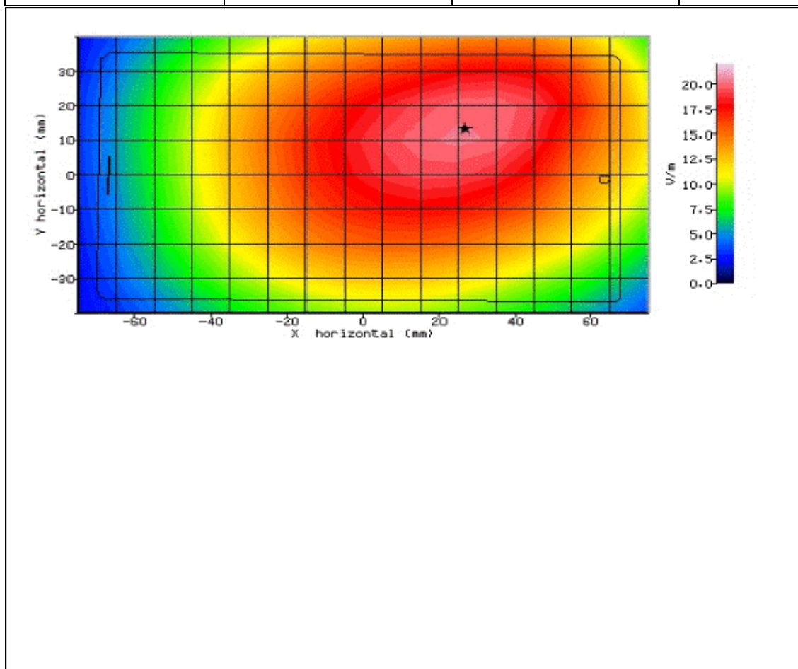
Figure 28: SAR Body Testing Results for the Sharp SHV32 Mobile Handset at 709.0MHz.
