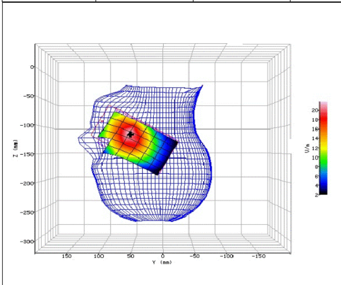
Figure 6: SAR Head Testing Results for the Sharp SHV32 Mobile Handset at 824.2MHz.
