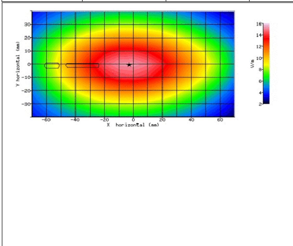
Figure 55: SAR Body Testing Results for the Sharp SHV32 Mobile Handset at 841.5MHz.
