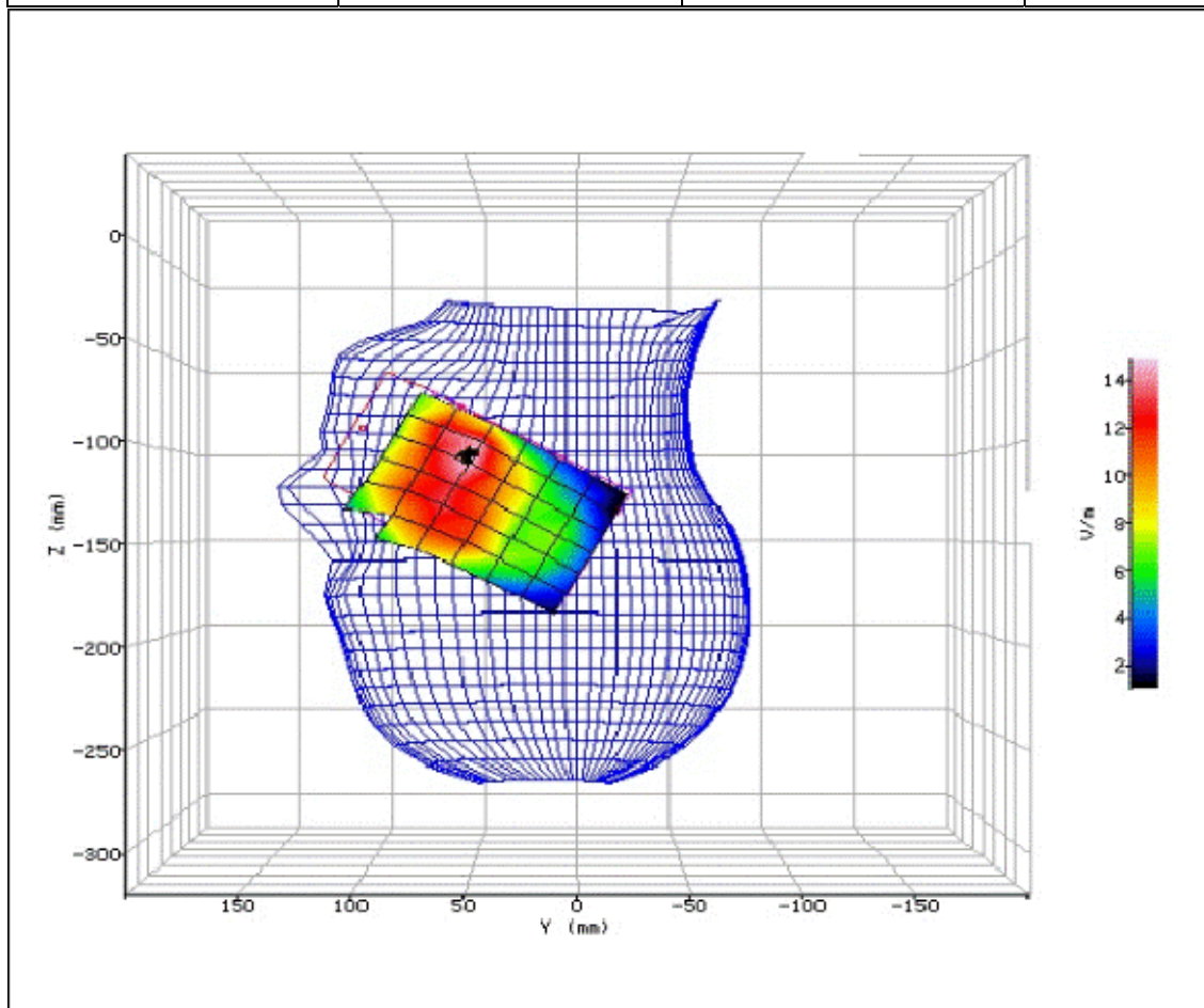
Figure 84: SAR Head Testing Results for the Sharp SHV32 Mobile Handset at 1880.0MHz.
