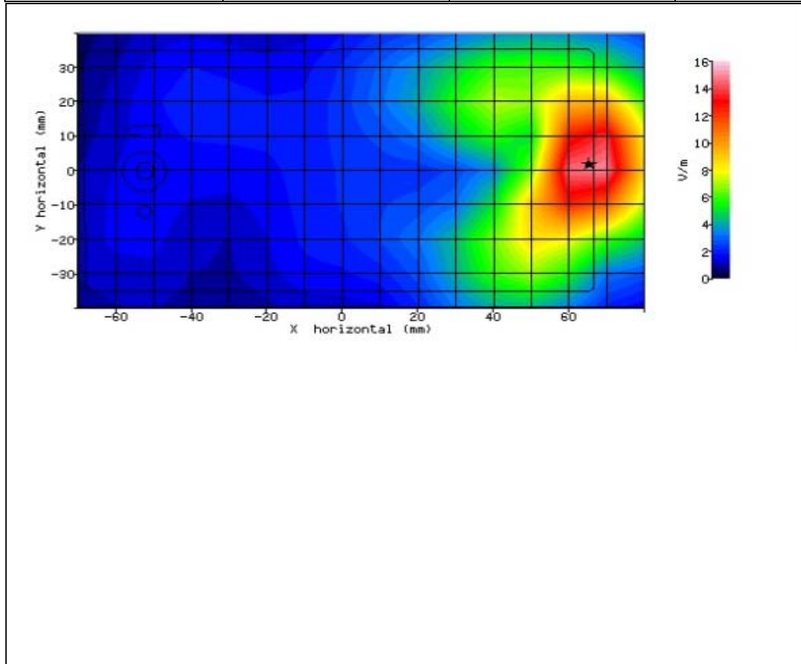
Figure 74: SAR Body Testing Results for the SHV32 Mobile Handset at 2593.0MHz.
