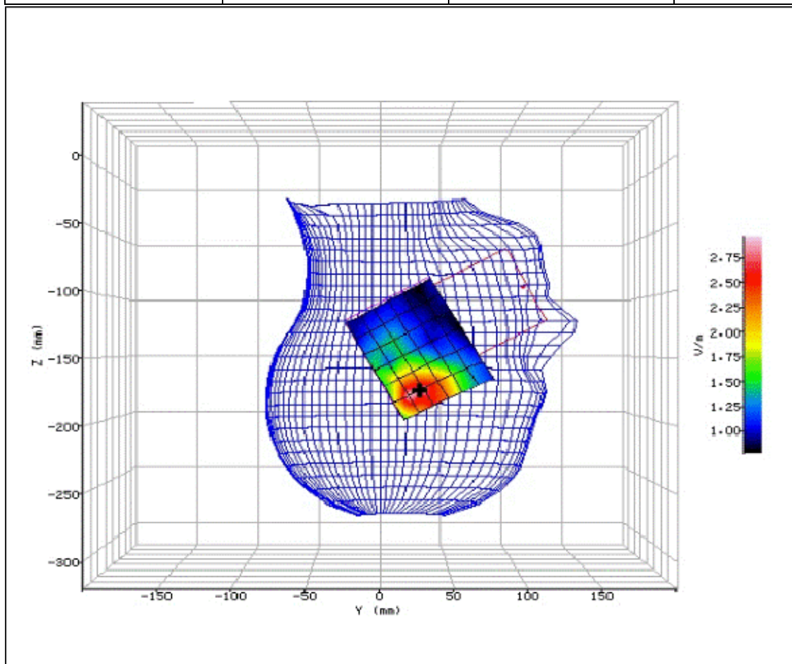
Figure 114: SAR Head Testing Results for the Sharp SHV32 Mobile Handset at 2437.0MHz.
