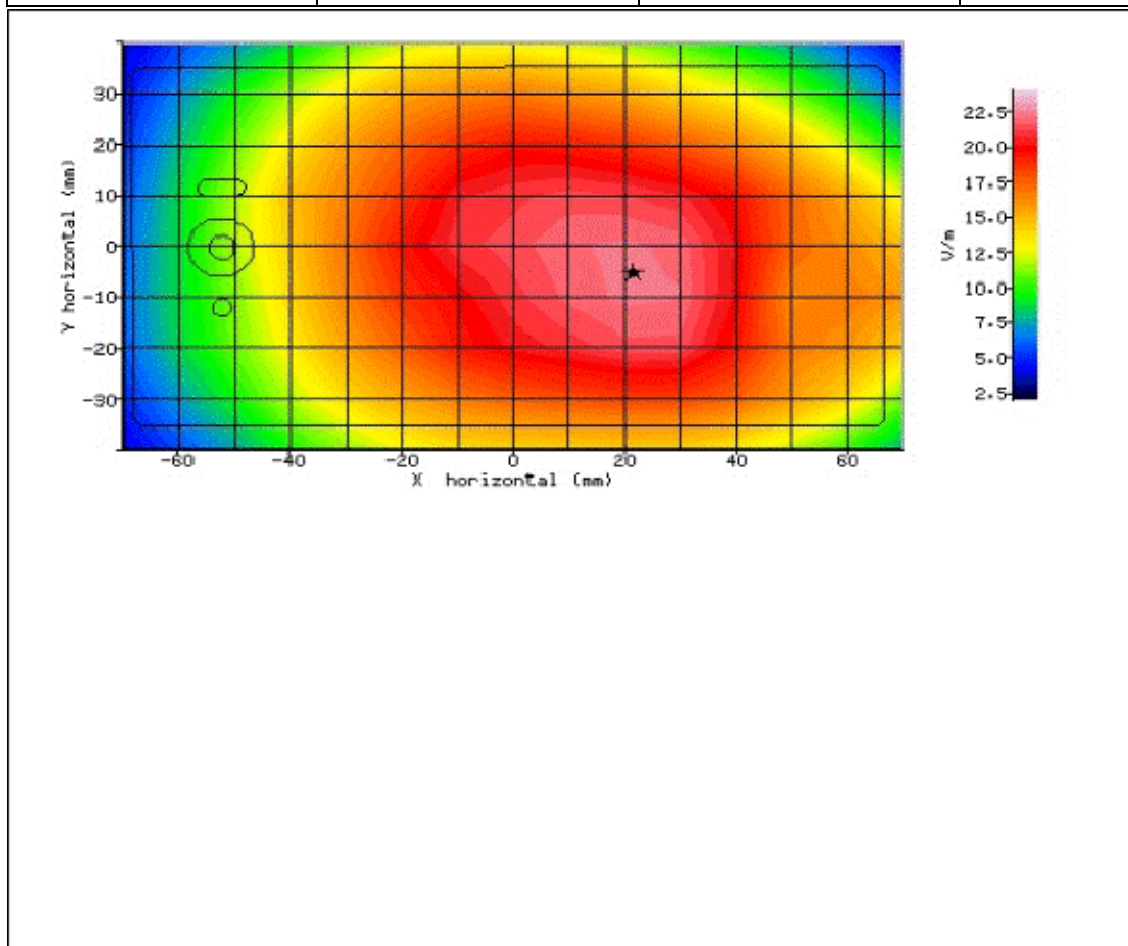
Figure 39: SAR Body Testing Results for the Sharp SHV32 Mobile Handset at 836.5MHz.
