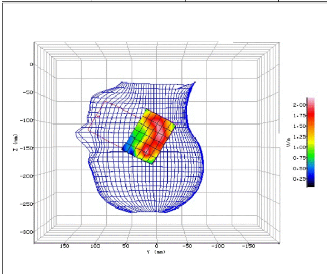
Figure 97: SAR Head Testing Results for the Sharp SHV32 Mobile Handset at 2437.0MHz.
