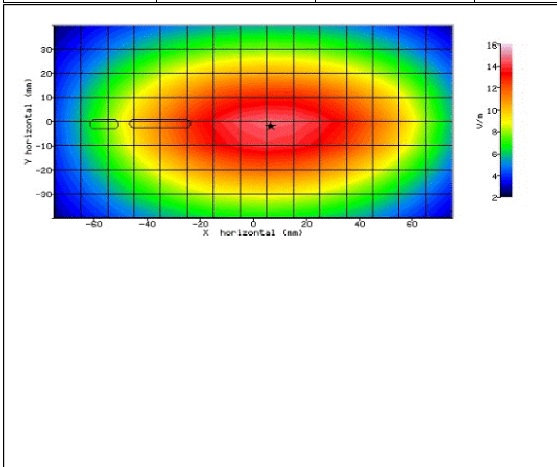
Figure 35: SAR Body Testing Results for the Sharp SHV32 Mobile Handset at 711.0MHz.
