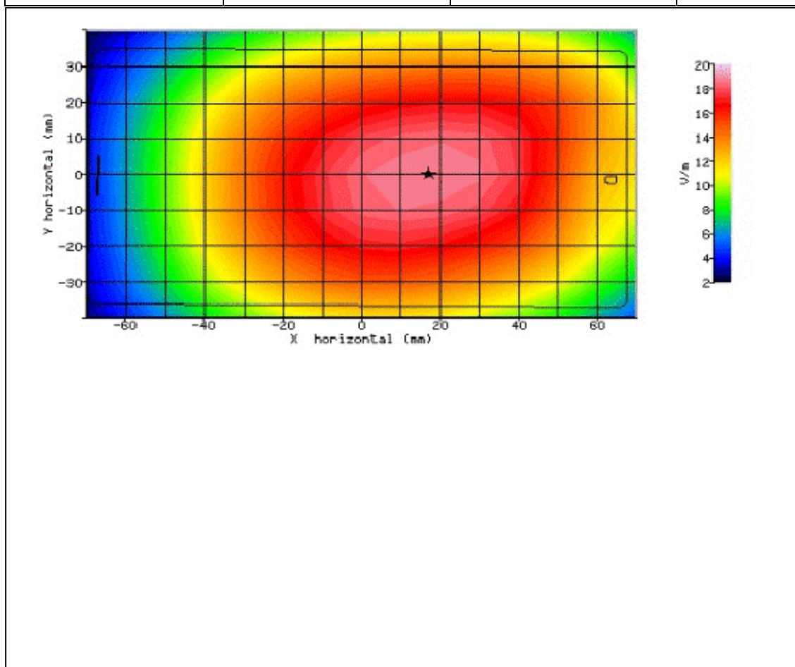
Figure 43: SAR Body Testing Results for the Sharp SHV32 Mobile Handset at 829.0MHz.
