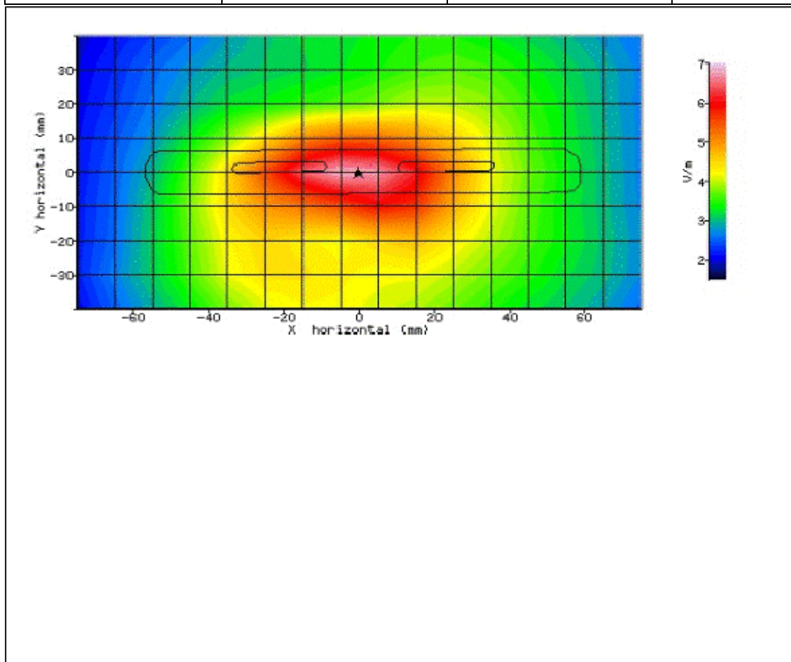
Figure 37: SAR Body Testing Results for the Sharp SHV32 Mobile Handset at 711.0MHz.
