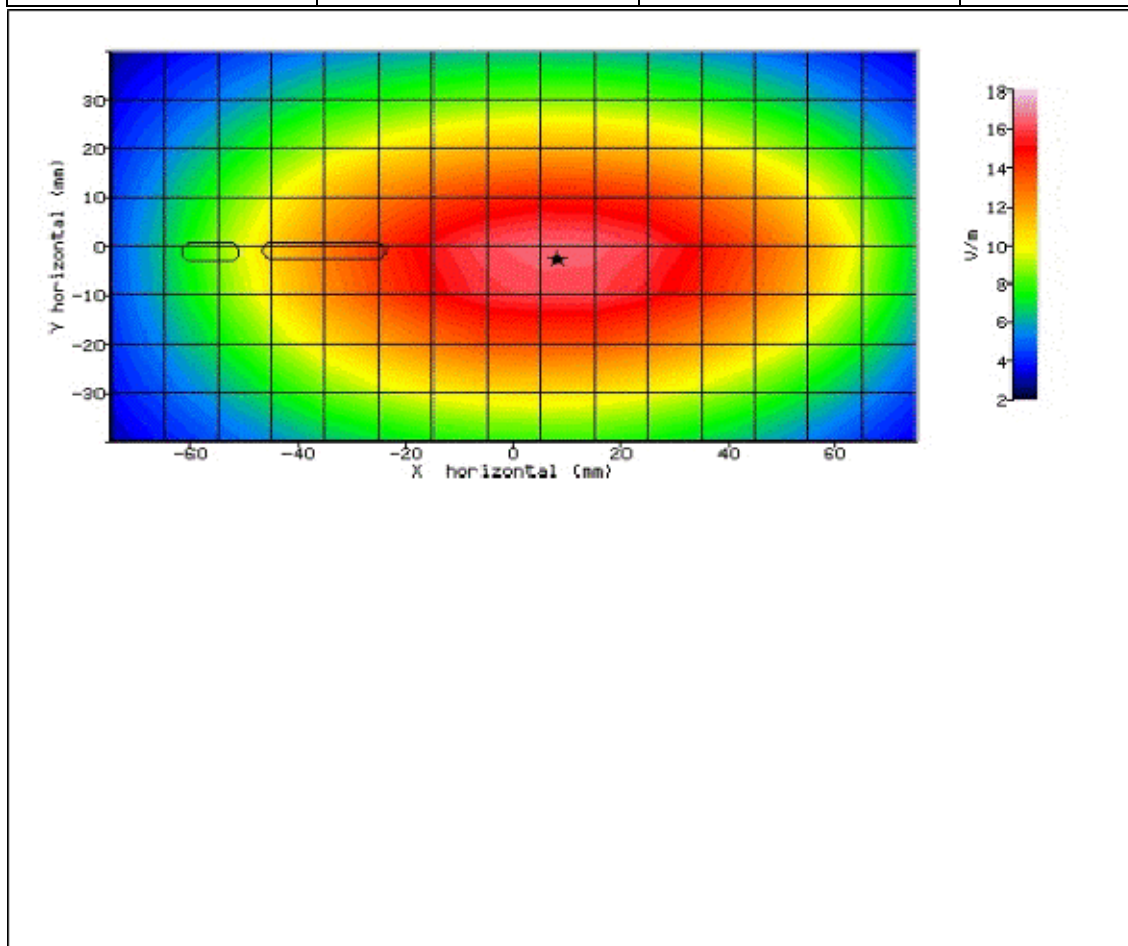
Figure 30: SAR Body Testing Results for the Sharp SHV32 Mobile Handset at 709.0MHz.
