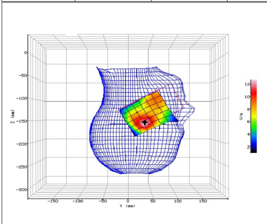
Figure 87: SAR Head Testing Results for the Sharp SHV32 Mobile Handset at 1880.0MHz.
