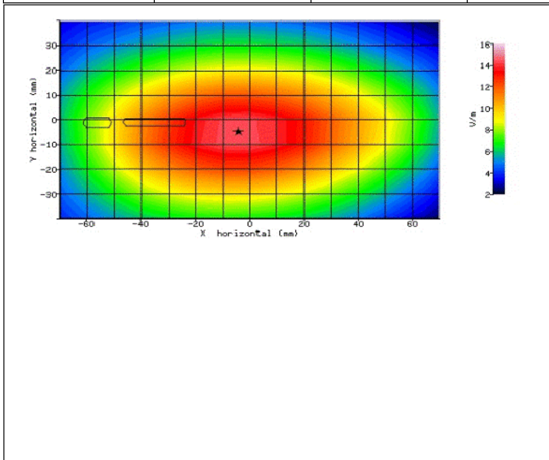
Figure 45: SAR Body Testing Results for the Sharp SHV32 Mobile Handset at 829.0MHz.
