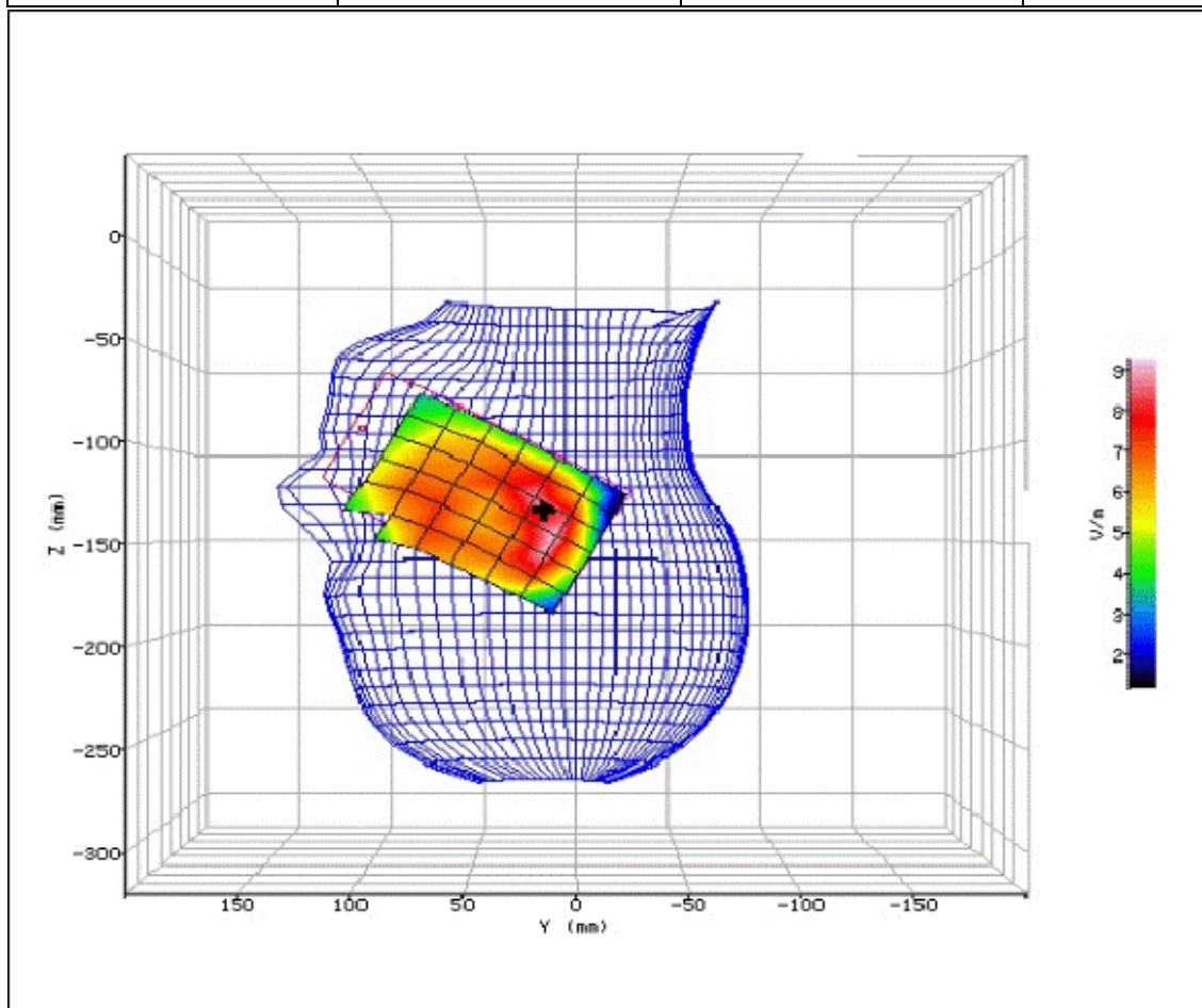
Figure 85: SAR Head Testing Results for the Sharp SHV32 Mobile Handset at 1880.0MHz.
