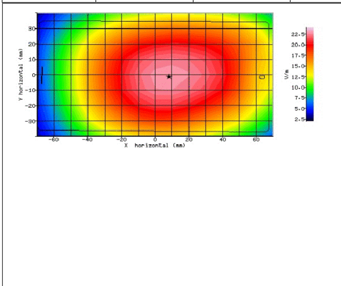
Figure 23: SAR Body Testing Results for the Sharp SHV32 Mobile Handset at 826.4MHz.
