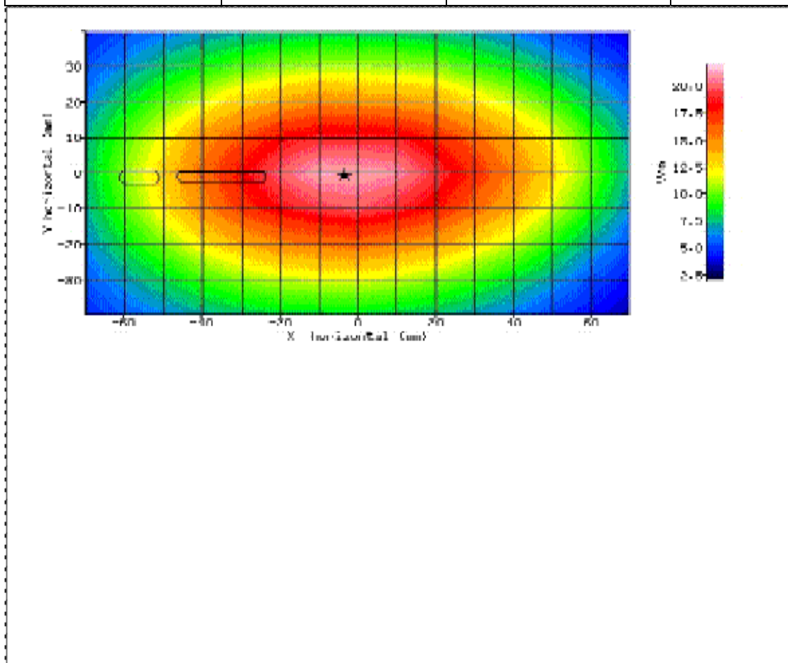
Figure 16: SAR Body Testing Results for the Sharp SHV32 Mobile Handset at 824.2MHz.
