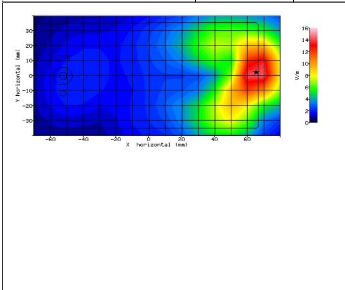
Figure 76: SAR Body Testing Results for the SHV32 Mobile Handset at 2636.5MHz.
