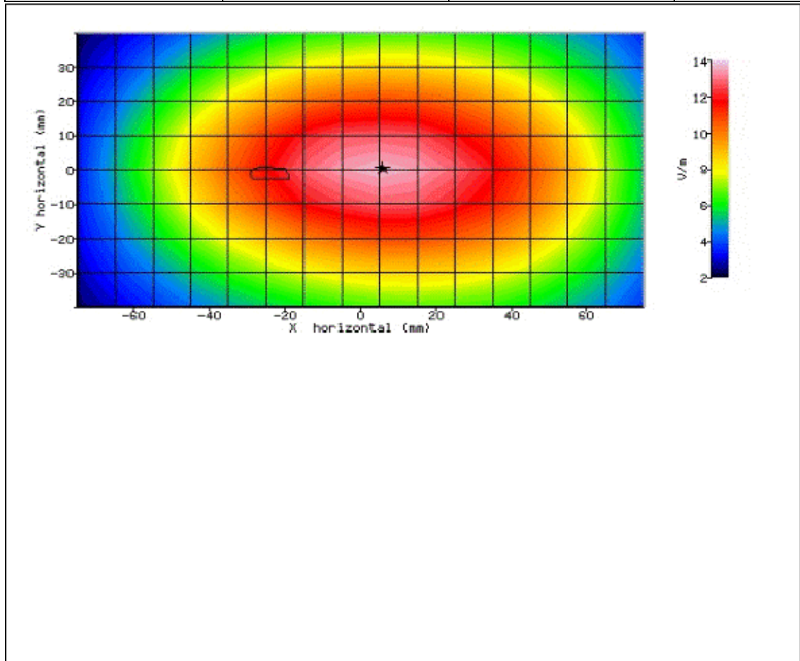
Figure 36: SAR Body Testing Results for the Sharp SHV32 Mobile Handset at 711.0MHz.
