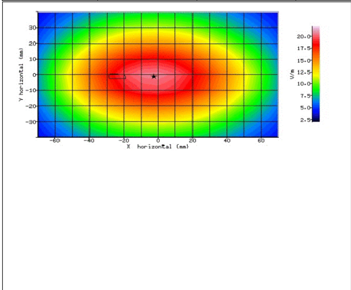
Figure 26: SAR Body Testing Results for the Sharp SHV32 Mobile Handset at 826.4MHz.
