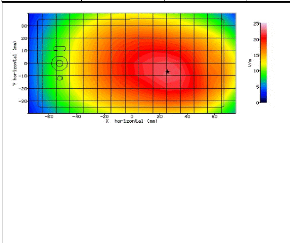
Figure 29: SAR Body Testing Results for the Sharp SHV32 Mobile Handset at 709.0MHz.
