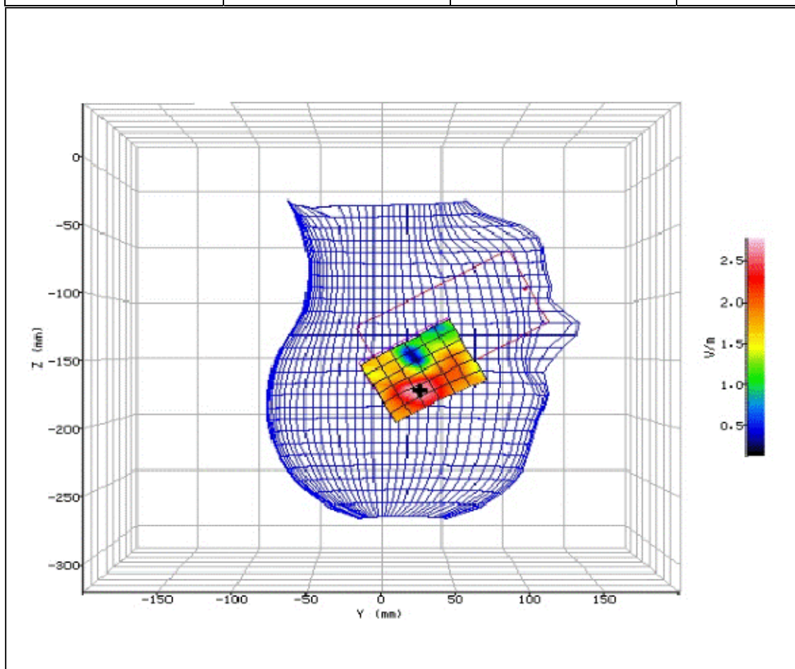
Figure 217: SAR Head Testing Results for the Sharp SHV32 Mobile Handset at 5280.0MHz. (NUA)
