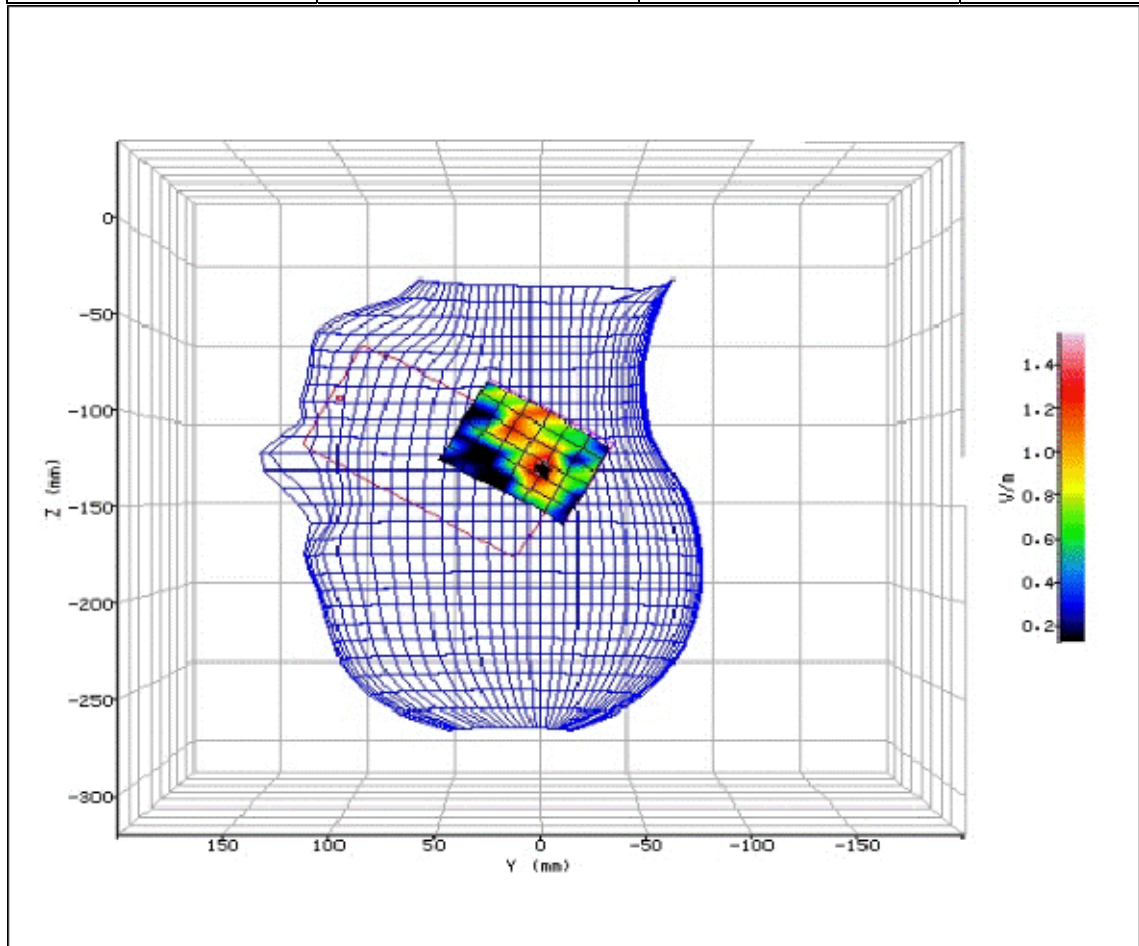
Figure 218: SAR Head Testing Results for the Sharp SHV32 Mobile Handset at 5600.0MHz. (NUA)
