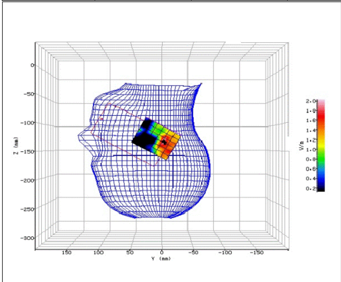
Figure 157: SAR Head Testing Results for the Sharp SHV32 Mobile Handset at 5600.0MHz. (NUA)
