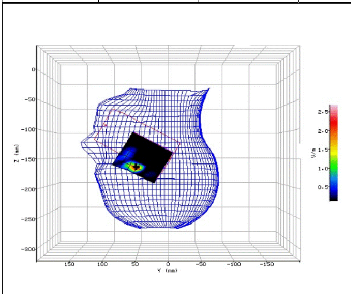
Figure 134: SAR Head Testing Results for the Sharp SHV32 Mobile Handset at 5180.0MHz. (NUA)
