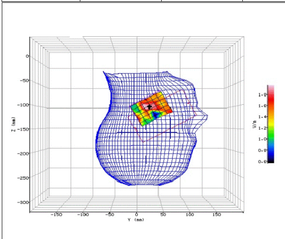
Figure 196: SAR Head Testing Results for the Sharp SHV32 Mobile Handset at 5270.0MHz. (NUA)
