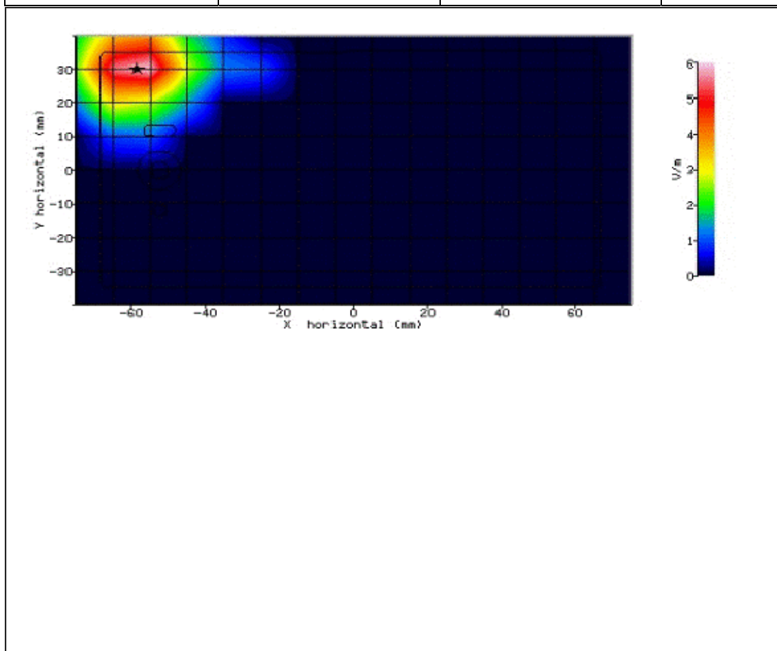
Figure 219: SAR Body Testing Results for the Sharp SHV32 Mobile Handset at 5180.0MHz. (NUA)
