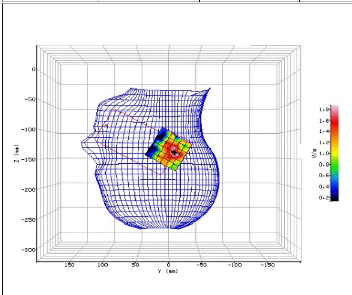
Figure 172: SAR Head Testing Results for the Sharp SHV32 Mobile Handset at 5190.0MHz. (NUA)
