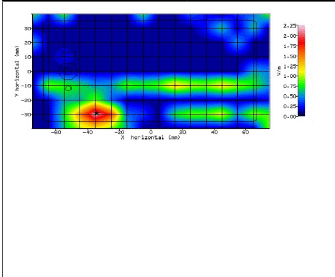
Figure 214: SAR Body Testing Results for the Sharp SHV32 Mobile Handset at 5590.0MHz. (NUA)
