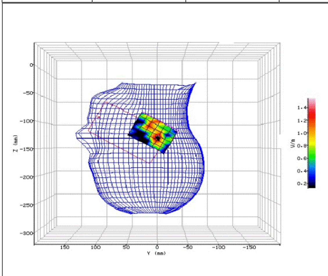
Figure 218: SAR Head Testing Results for the Sharp SHV32 Mobile Handset at 5600.0MHz. (NUA)
