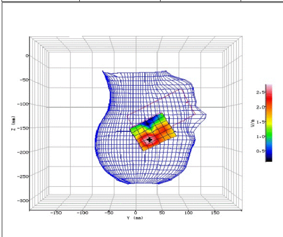
Figure 143: SAR Head Testing Results for the Sharp SHV32 Mobile Handset at 5280.0MHz. (NUA)
