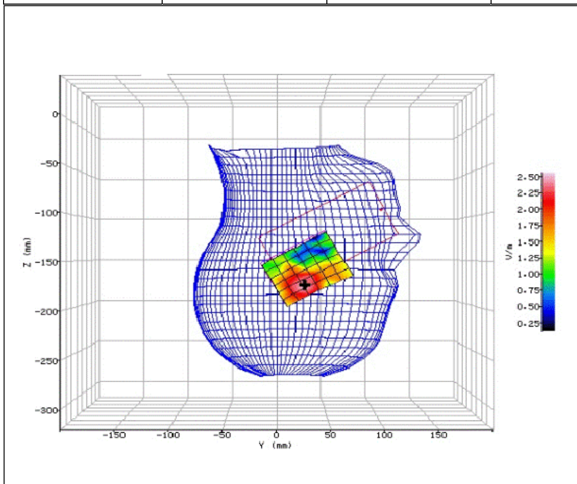
Figure 216: SAR Head Testing Results for the Sharp SHV32 Mobile Handset at 5180.0MHz. (NUA)
