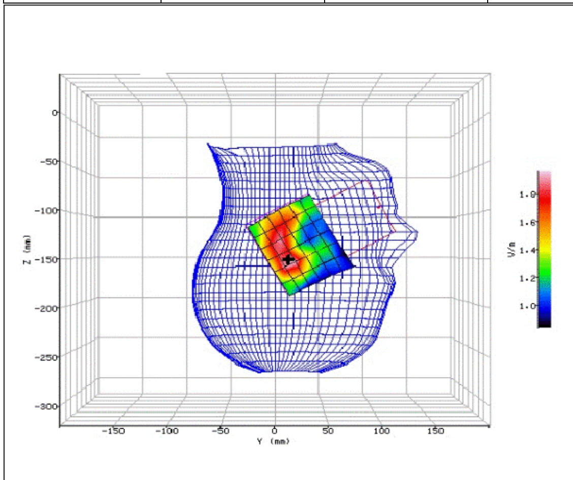
Figure 122: SAR Head Testing Results for the Sharp SHV32 Mobile Handset at 2437.0MHz.
