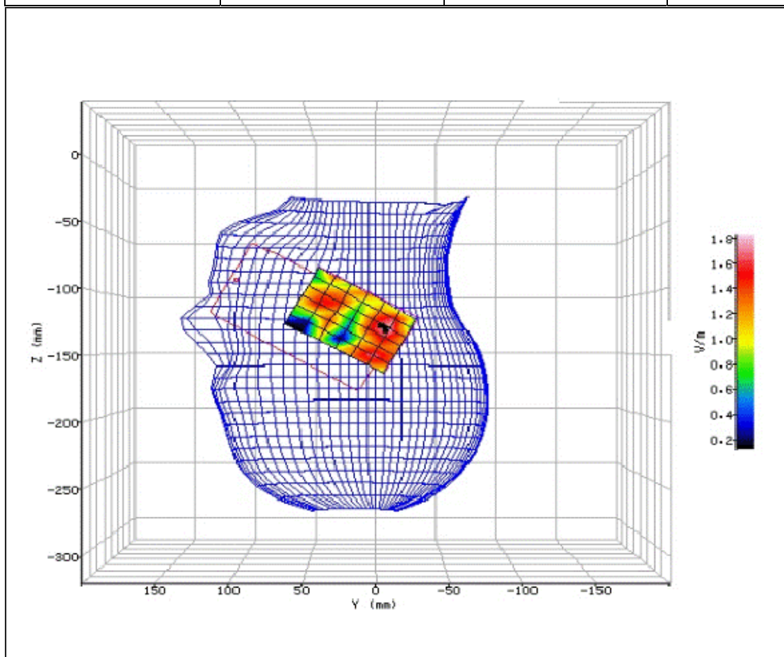
Figure 156: SAR Head Testing Results for the Sharp SHV32 Mobile Handset at 5600.0MHz. (NUA)
