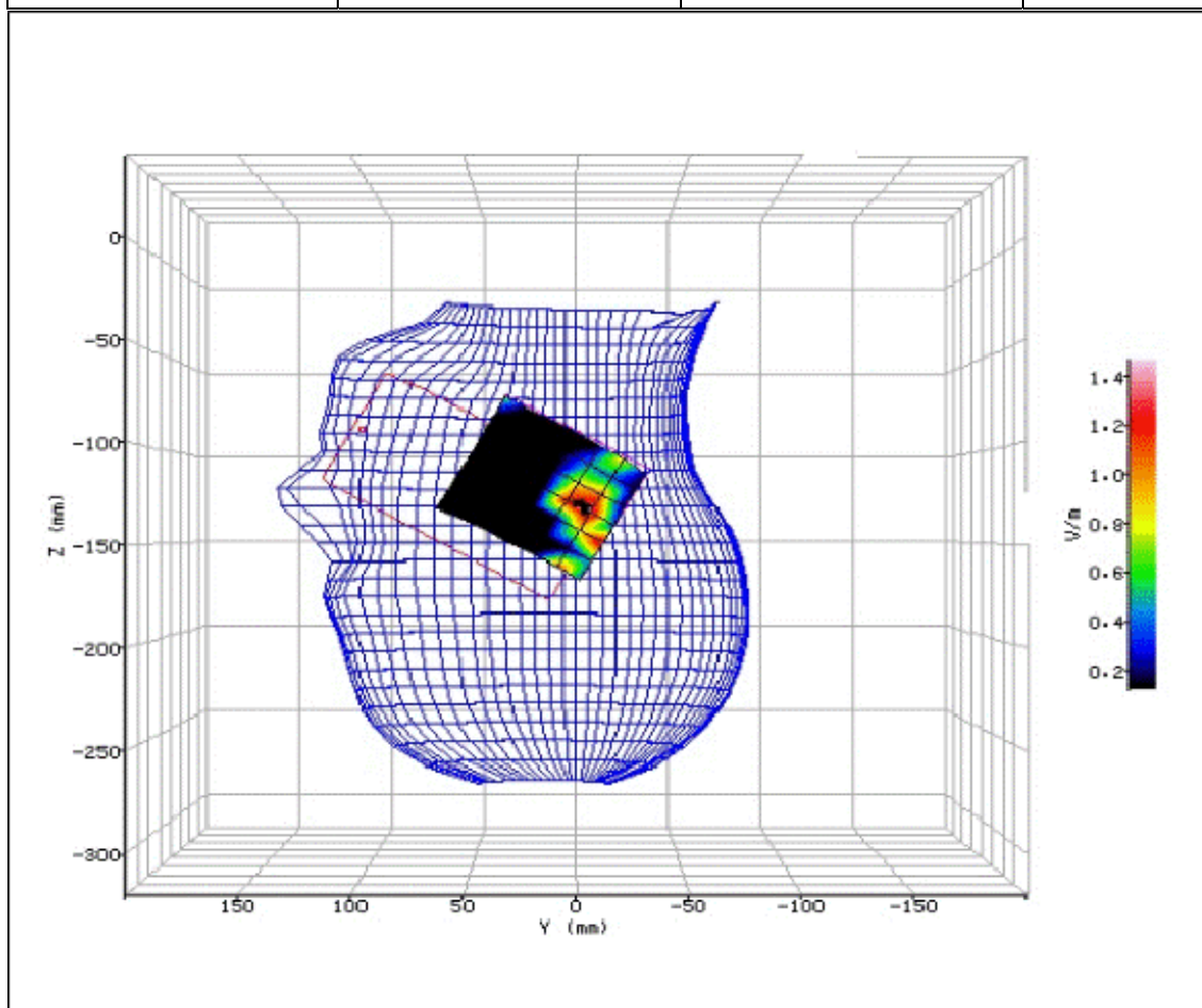
Figure 141: SAR Head Testing Results for the Sharp SHV32 Mobile Handset at 5280.0MHz. (NUA)
