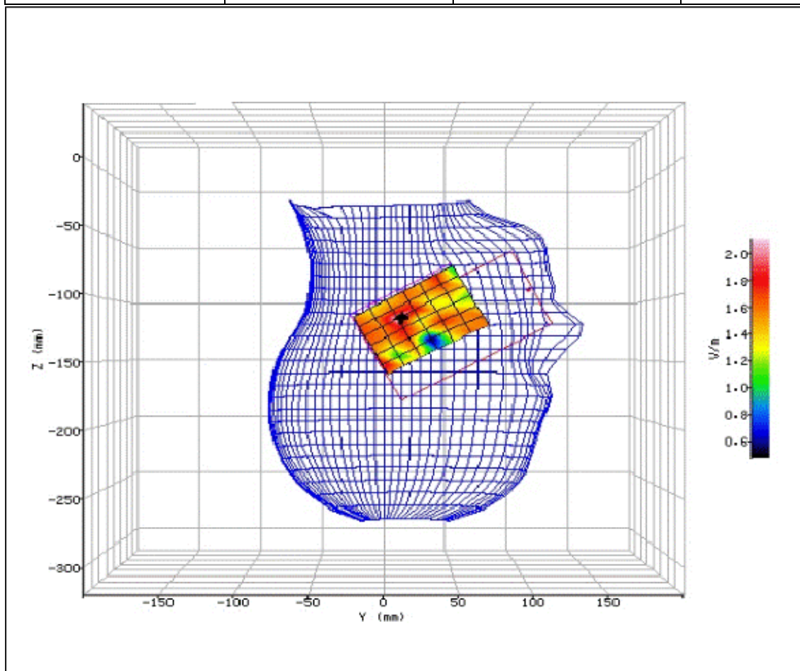
Figure 211: SAR Head Testing Results for the Sharp SHV32 Mobile Handset at 5590.0MHz. (NUA)
