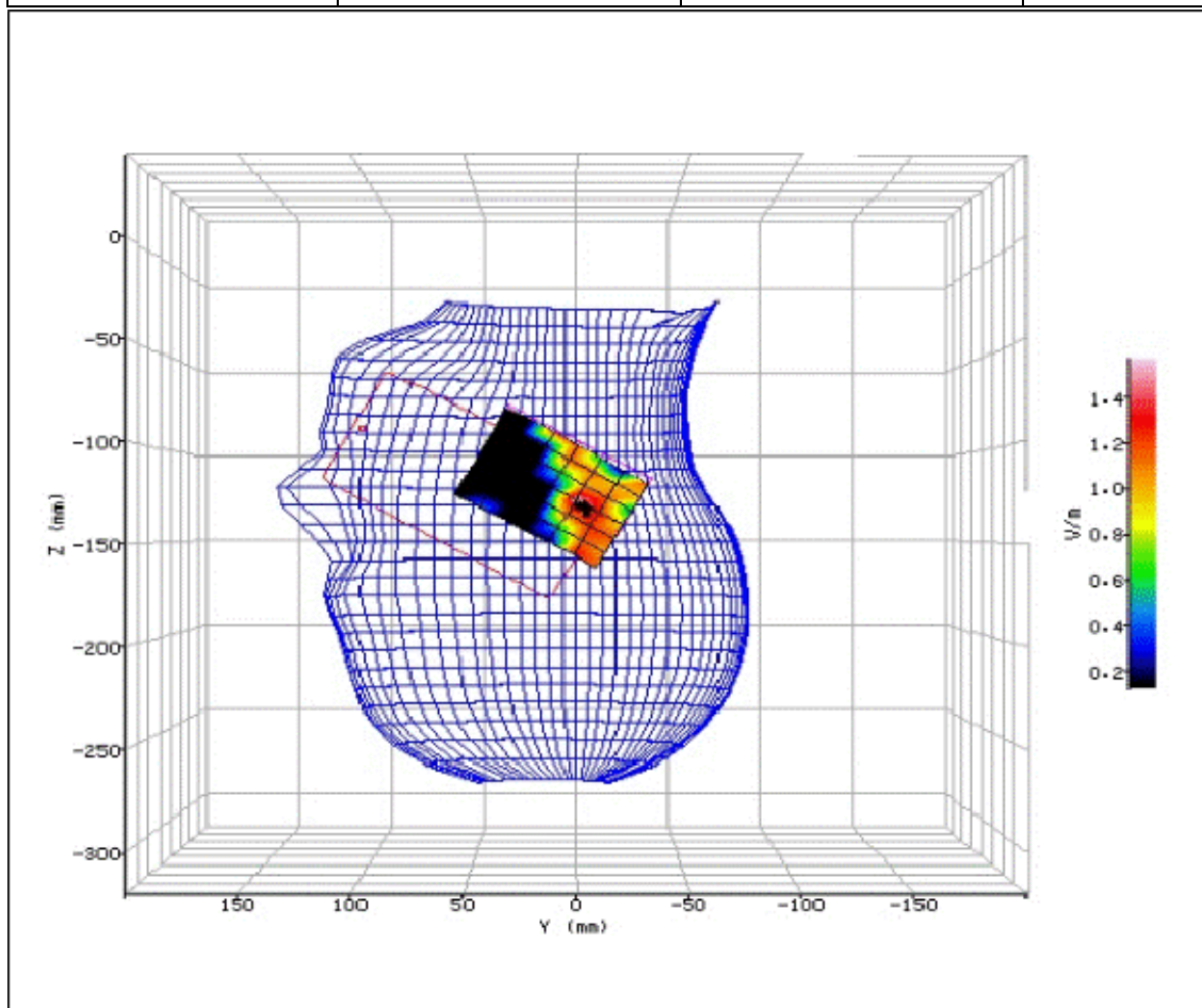
Figure 202: SAR Head Testing Results for the Sharp SHV32 Mobile Handset at 5590.0MHz. (NUA)
