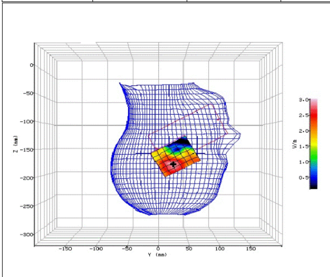
Figure 189: SAR Head Testing Results for the Sharp SHV32 Mobile Handset at 5270.0MHz. (NUA)
