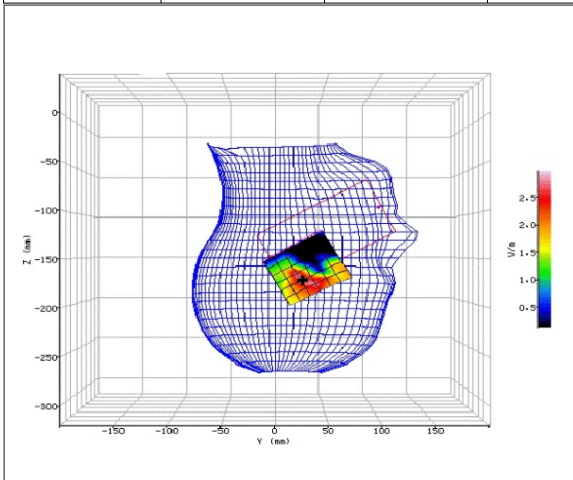
Figure 159: SAR Head Testing Results for the Sharp SHV32 Mobile Handset at 5600.0MHz. (NUA)
