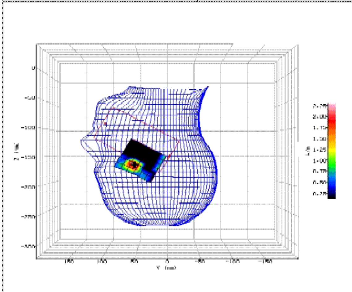
Figure 179: SAR Head Testing Results for the Sharp SHV32 Mobile Handset at 5190.0MHz. (NUA)
