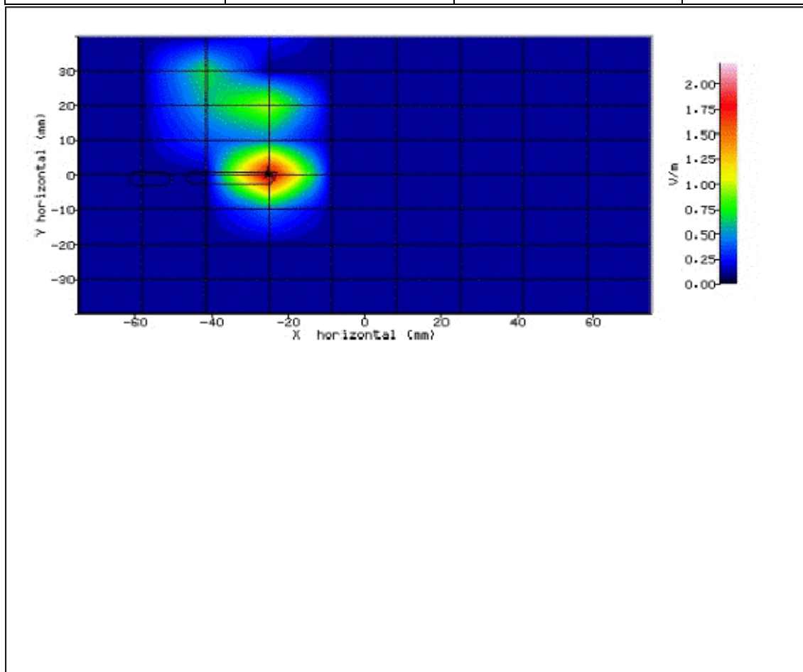
Figure 185: SAR Body Testing Results for the Sharp SHV32 Mobile Handset at 5190.0MHz. (NUA)
