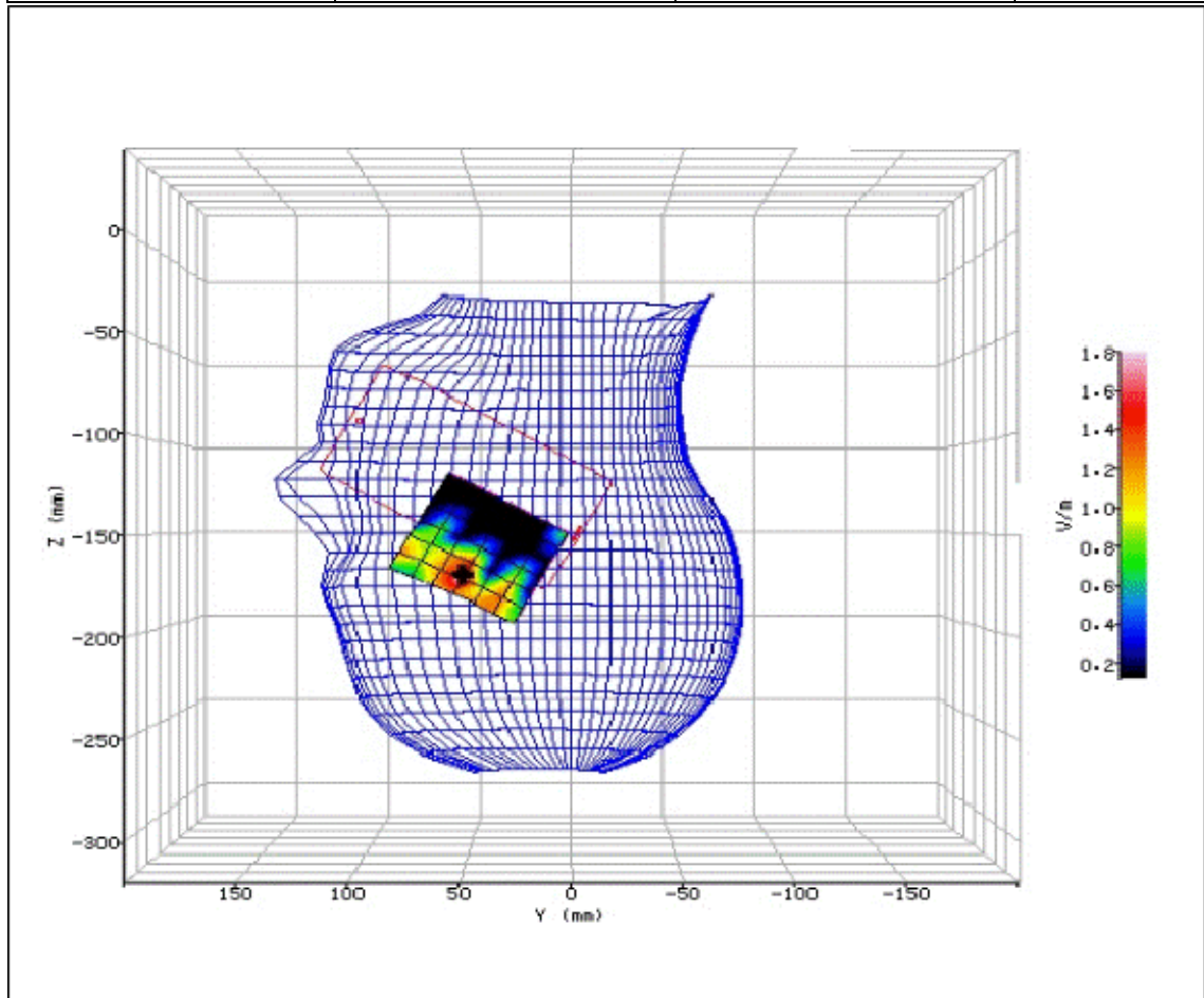
Figure 180: SAR Head Testing Results for the Sharp SHV32 Mobile Handset at 5190.0MHz. (NUA)
