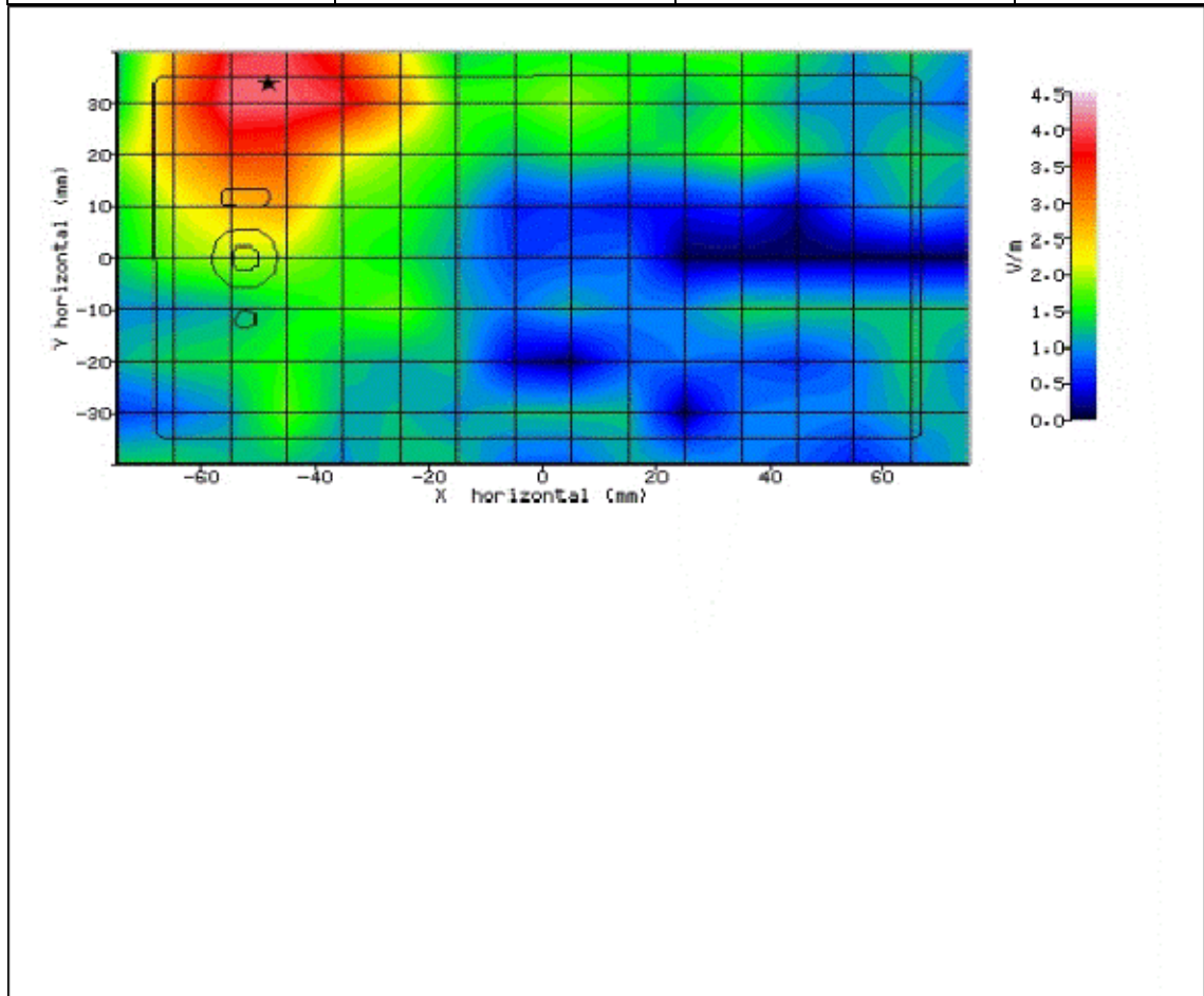
Figure 221: SAR Body Testing Results for the Sharp SHV32 Mobile Handset at 5600.0MHz. (NUA)
