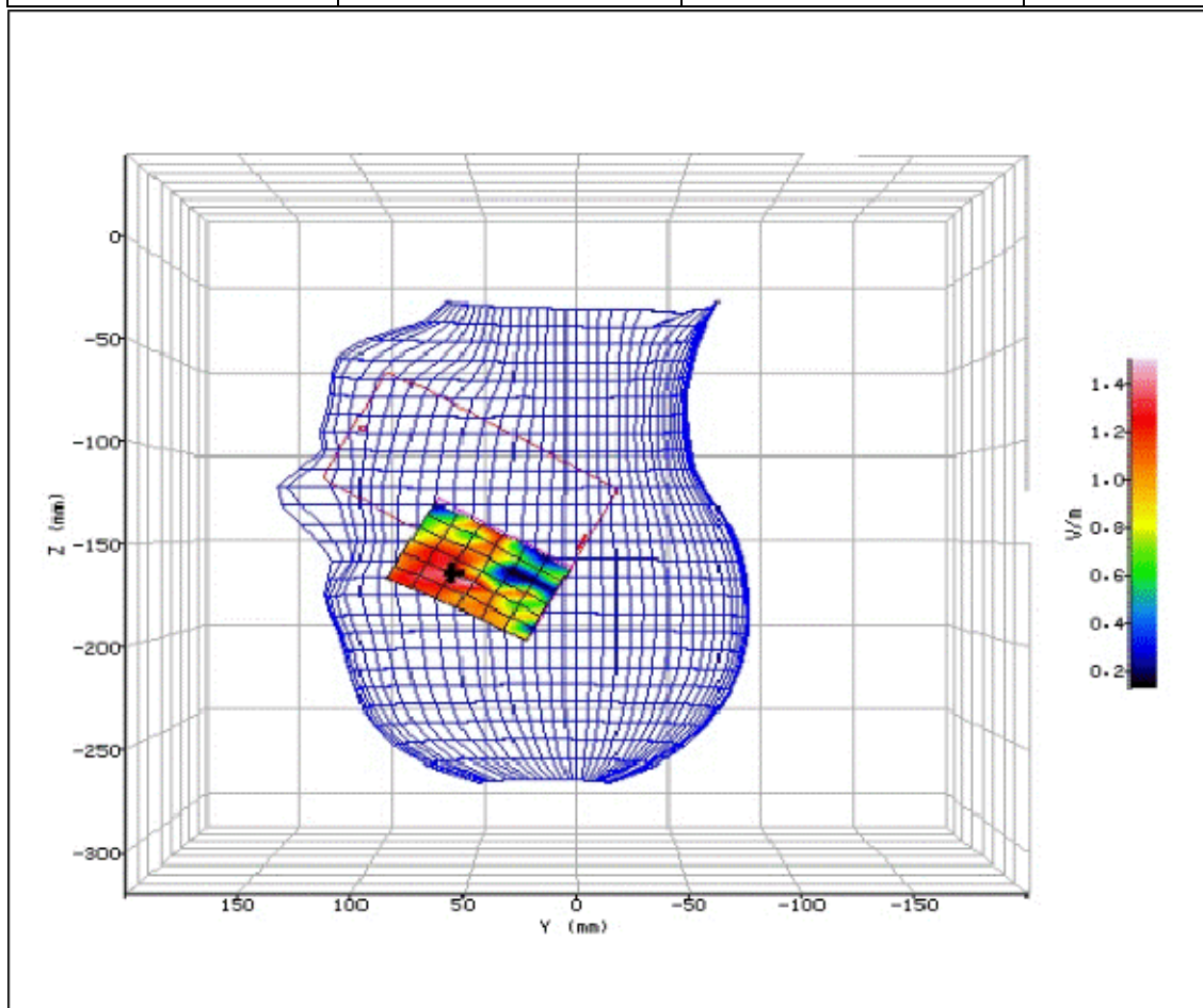
Figure 165: SAR Head Testing Results for the Sharp SHV32 Mobile Handset at 5600.0MHz. (NUA)
