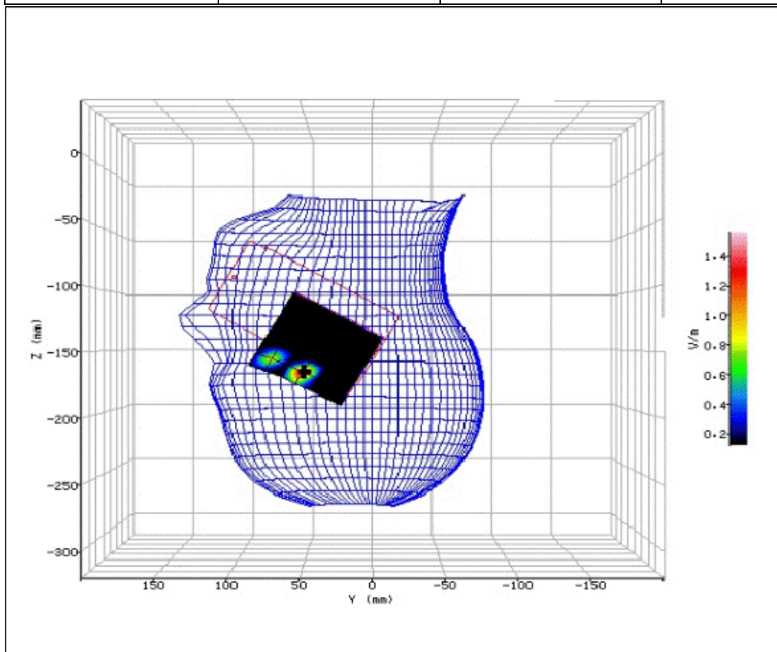
Figure 135: SAR Head Testing Results for the Sharp SHV32 Mobile Handset at 5180.0MHz. (NUA)
