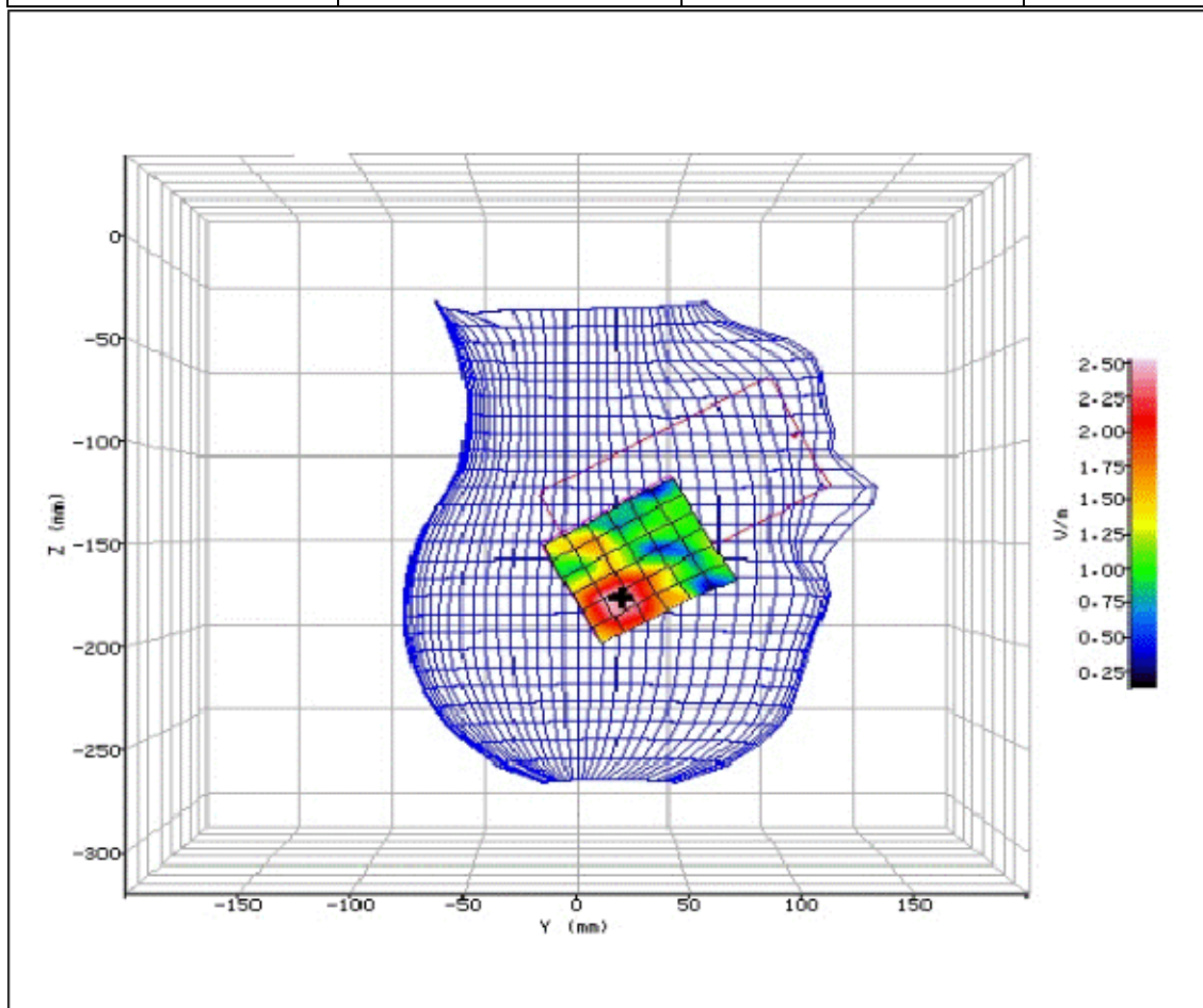
Figure 174: SAR Head Testing Results for the Sharp SHV32 Mobile Handset at 5190.0MHz. (NUA)
