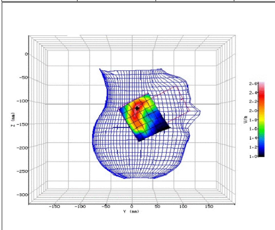
Figure 121: SAR Head Testing Results for the Sharp SHV32 Mobile Handset at 2437.0MHz.
