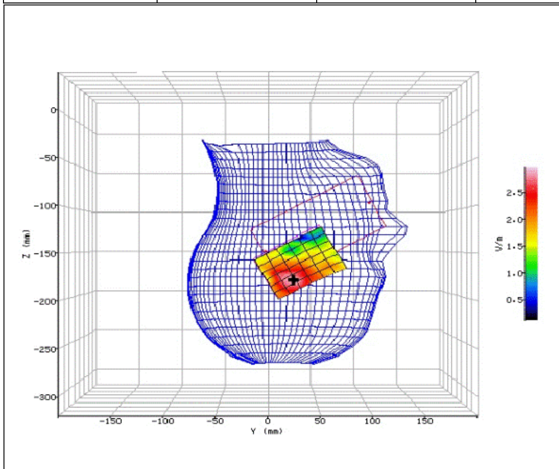
Figure 129: SAR Head Testing Results for the Sharp SHV32 Mobile Handset at 5180.0MHz. (NUA)
