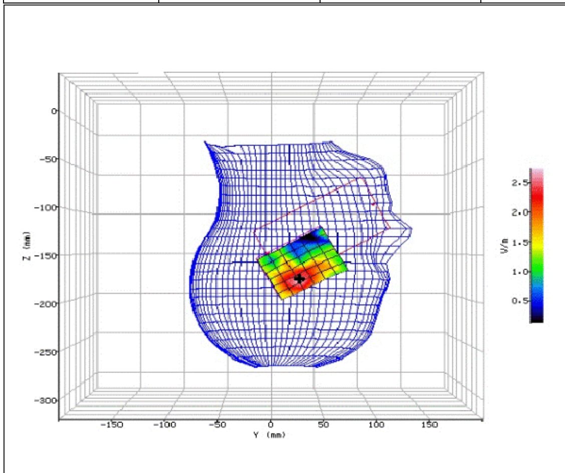
Figure 173: SAR Head Testing Results for the Sharp SHV32 Mobile Handset at 5190.0MHz. (NUA)
