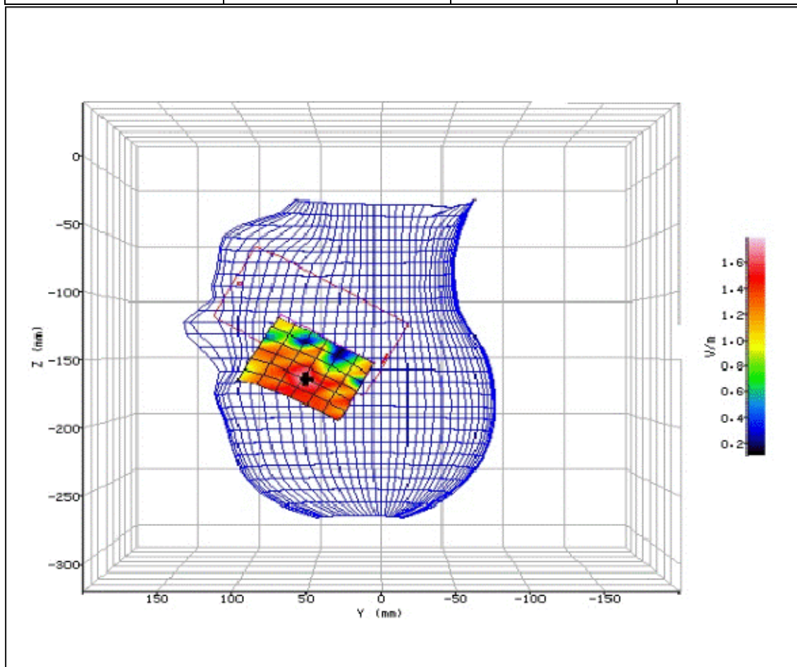
Figure 195: SAR Head Testing Results for the Sharp SHV32 Mobile Handset at 5270.0MHz. (NUA)
