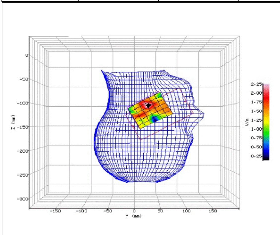
Figure 136: SAR Head Testing Results for the Sharp SHV32 Mobile Handset at 5180.0MHz. (NUA)
