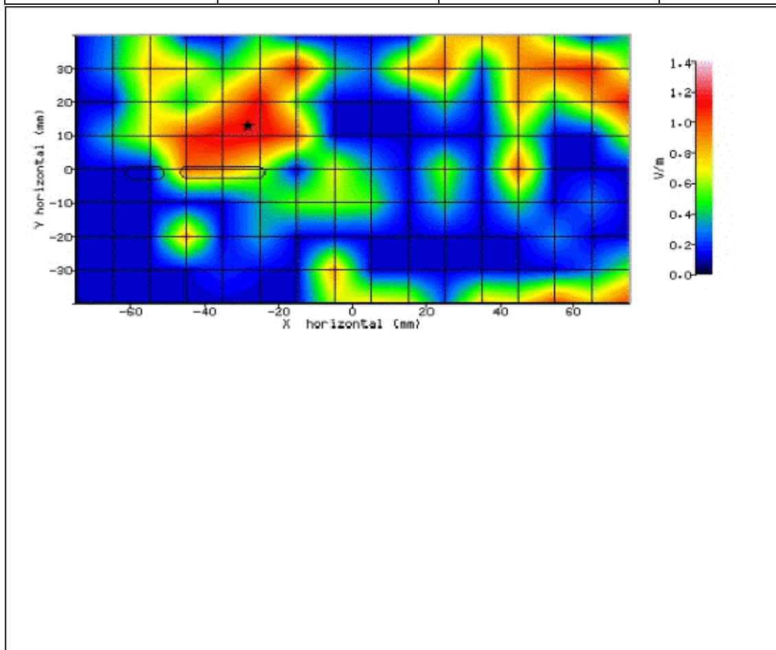
Figure 215: SAR Body Testing Results for the Sharp SHV32 Mobile Handset at 5590.0MHz. (NUA)
