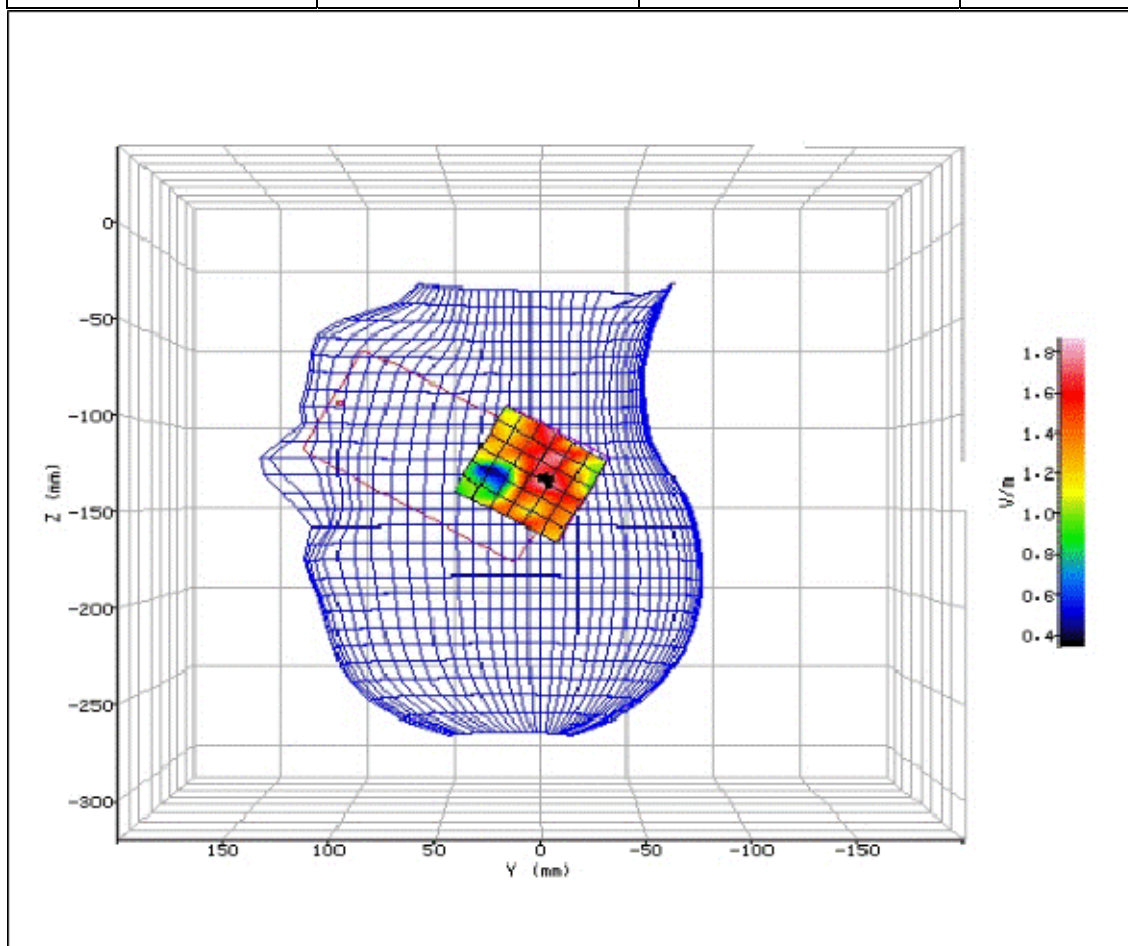
Figure 186: SAR Head Testing Results for the Sharp SHV32 Mobile Handset at 5270.0MHz. (NUA)
