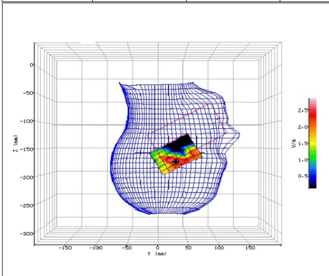
Figure 203: SAR Head Testing Results for the Sharp SHV32 Mobile Handset at 5590.0MHz. (NUA)
