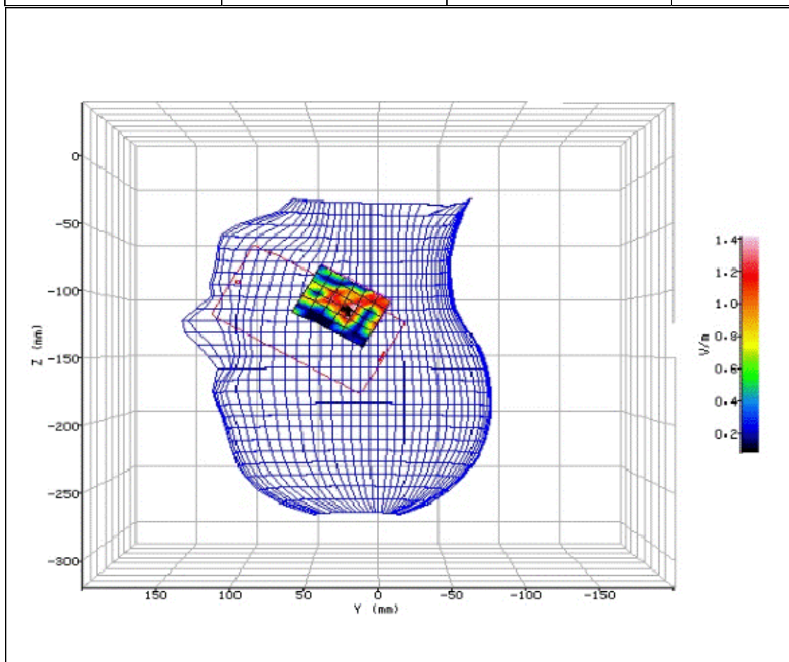
Figure 126: SAR Head Testing Results for the Sharp SHV32 Mobile Handset at 5180.0MHz. (NUA)
