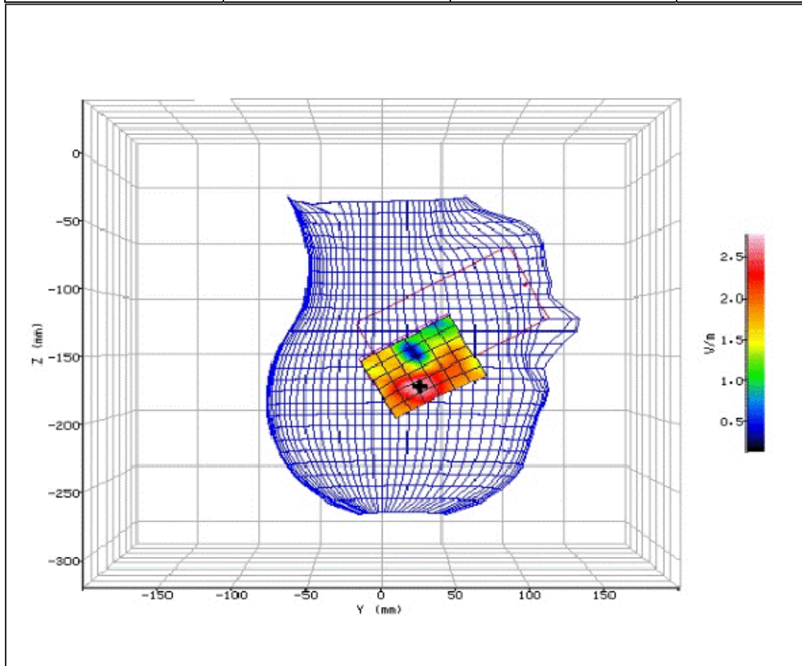
Figure 217: SAR Head Testing Results for the Sharp SHV32 Mobile Handset at 5280.0MHz. (NUA)
