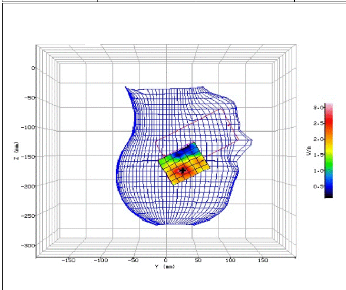
Figure 188: SAR Head Testing Results for the Sharp SHV32 Mobile Handset at 5270.0MHz. (NUA)
