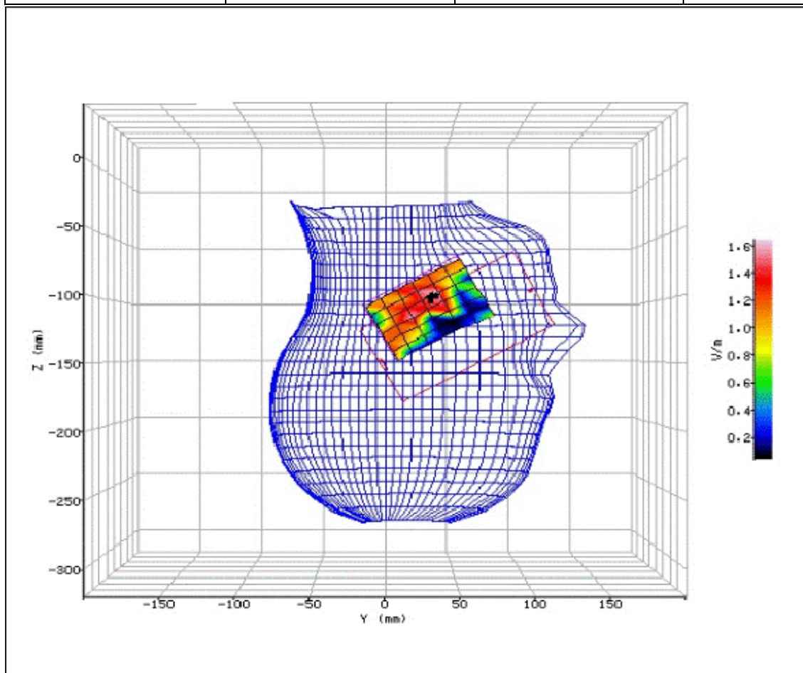
Figure 151: SAR Head Testing Results for the Sharp SHV32 Mobile Handset at 5280.0MHz. (NUA)
