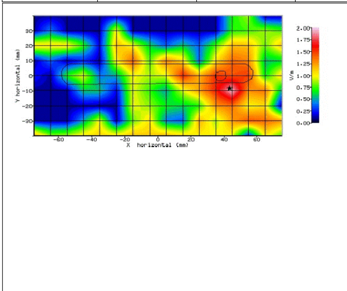
Figure 208: SAR Body Testing Results for the Sharp SHV32 Mobile Handset at 5590.0MHz. (NUA)
