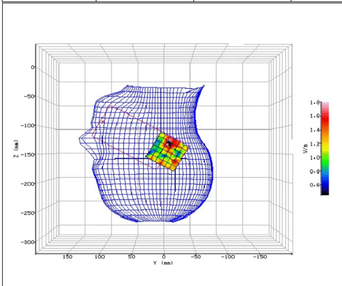
Figure 187: SAR Head Testing Results for the Sharp SHV32 Mobile Handset at 5270.0MHz. (NUA)
