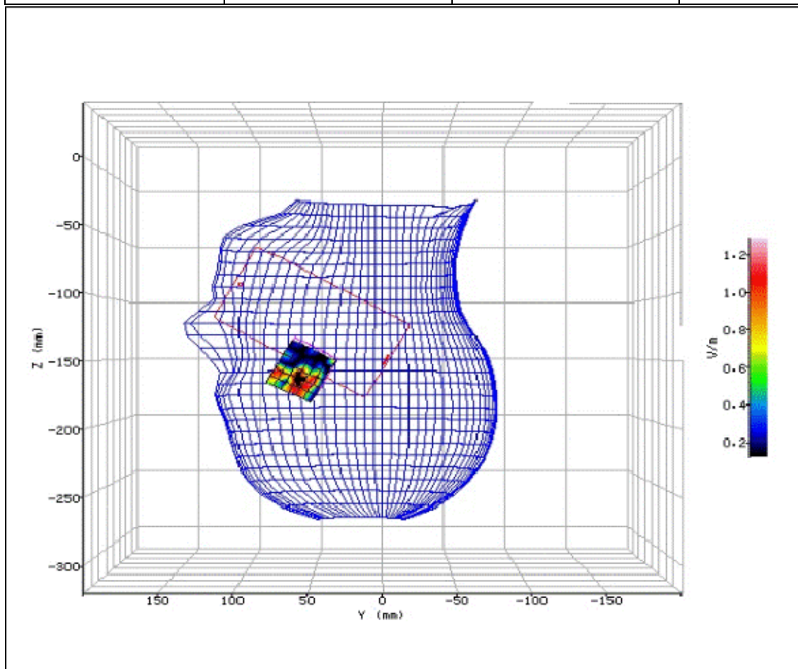
Figure 150: SAR Head Testing Results for the Sharp SHV32 Mobile Handset at 5280.0MHz. (NUA)
