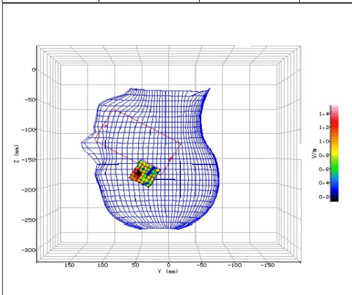
Figure 164: SAR Head Testing Results for the Sharp SHV32 Mobile Handset at 5600.0MHz. (NUA)
