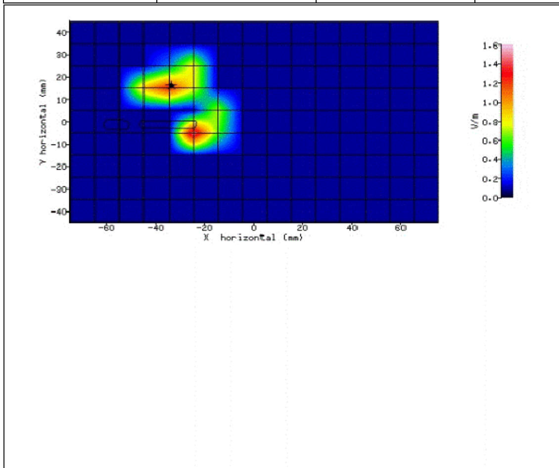
Figure 140: SAR Body Testing Results for the Sharp SHV32 Mobile Handset at 5180.0MHz. (NUA)
