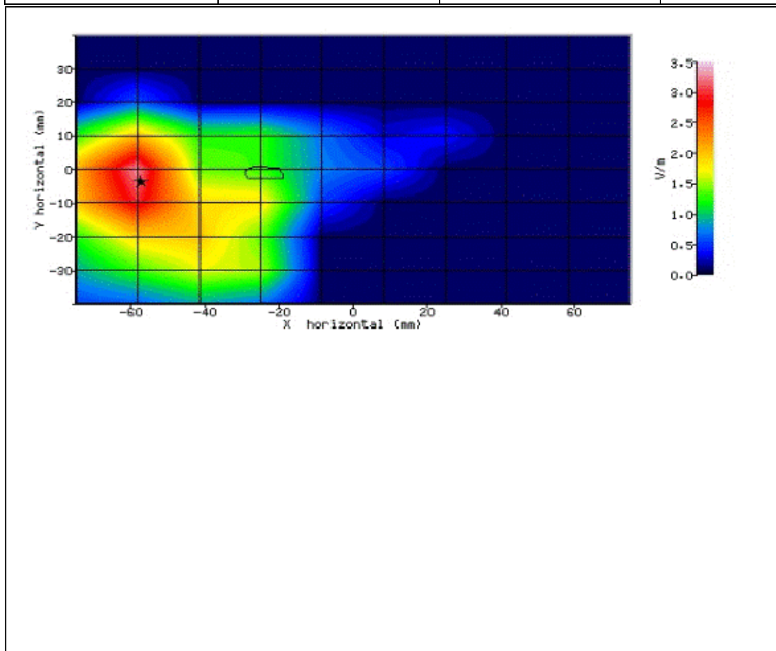
Figure 192: SAR Body Testing Results for the Sharp SHV32 Mobile Handset at 5270.0MHz. (NUA)
