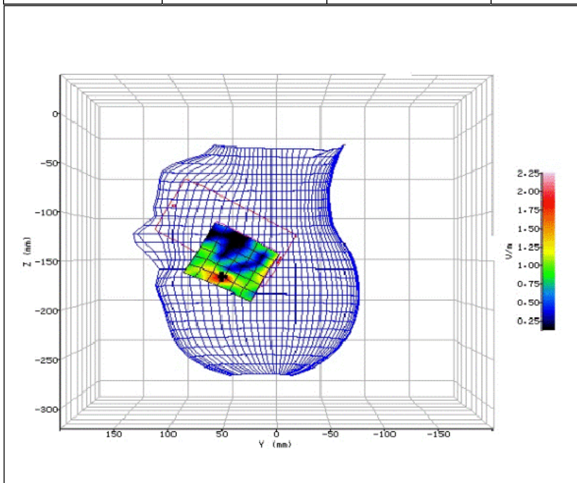
Figure 149: SAR Head Testing Results for the Sharp SHV32 Mobile Handset at 5280.0MHz. (NUA)
