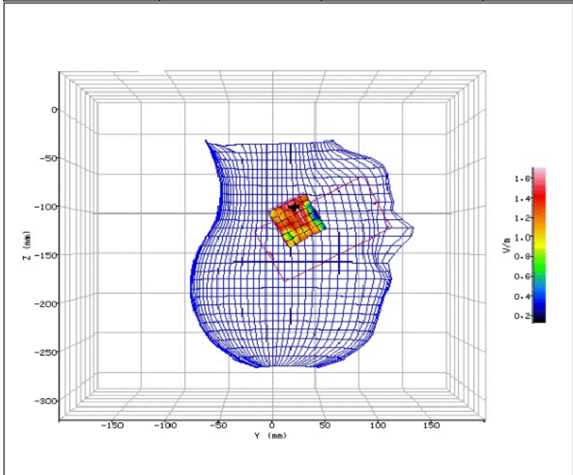
Figure 137: SAR Head Testing Results for the Sharp SHV32 Mobile Handset at 5180.0MHz. (NUA)
