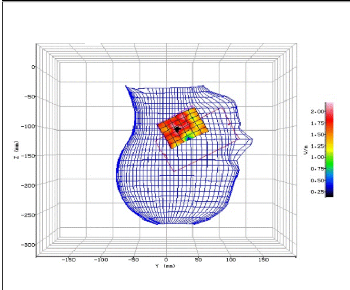
Figure 181: SAR Head Testing Results for the Sharp SHV32 Mobile Handset at 5190.0MHz. (NUA)
