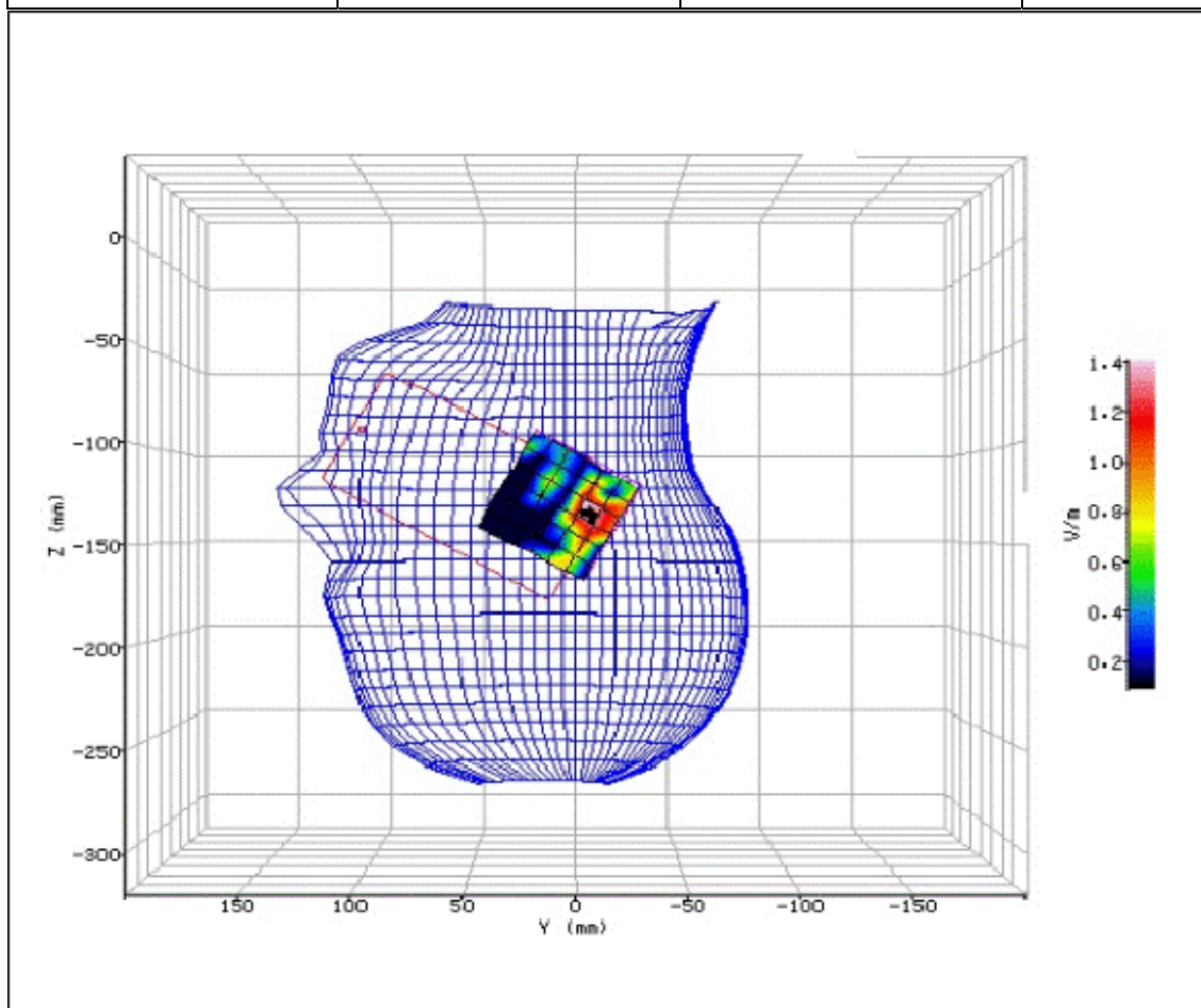
Figure 171: SAR Head Testing Results for the Sharp SHV32 Mobile Handset at 5190.0MHz. (NUA)
