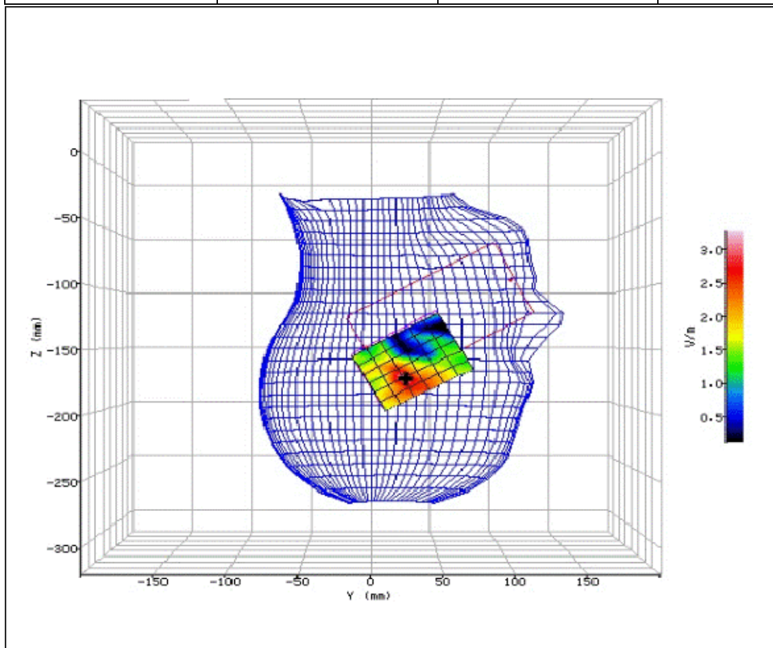
Figure 204: SAR Head Testing Results for the Sharp SHV32 Mobile Handset at 5590.0MHz. (NUA)
