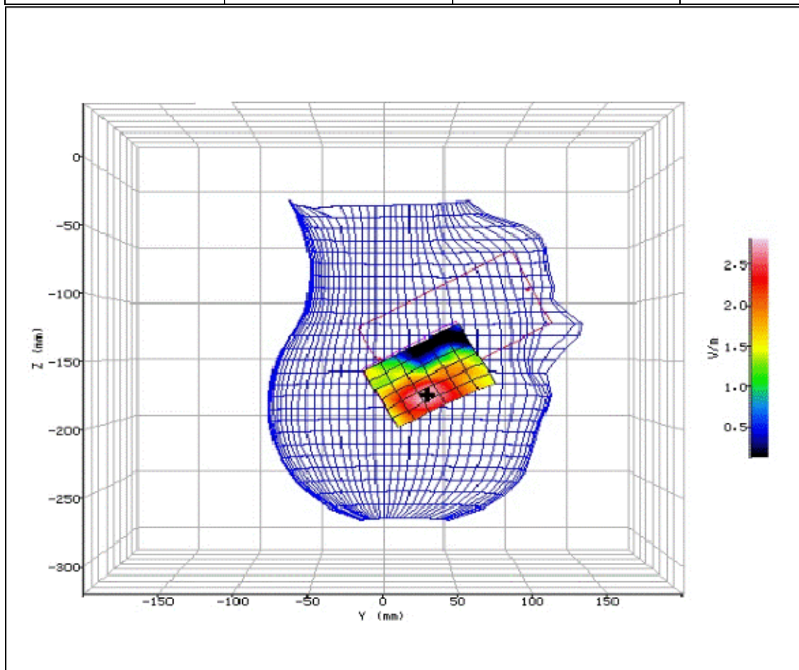
Figure 128: SAR Head Testing Results for the Sharp SHV32 Mobile Handset at 5180.0MHz. (NUA)
