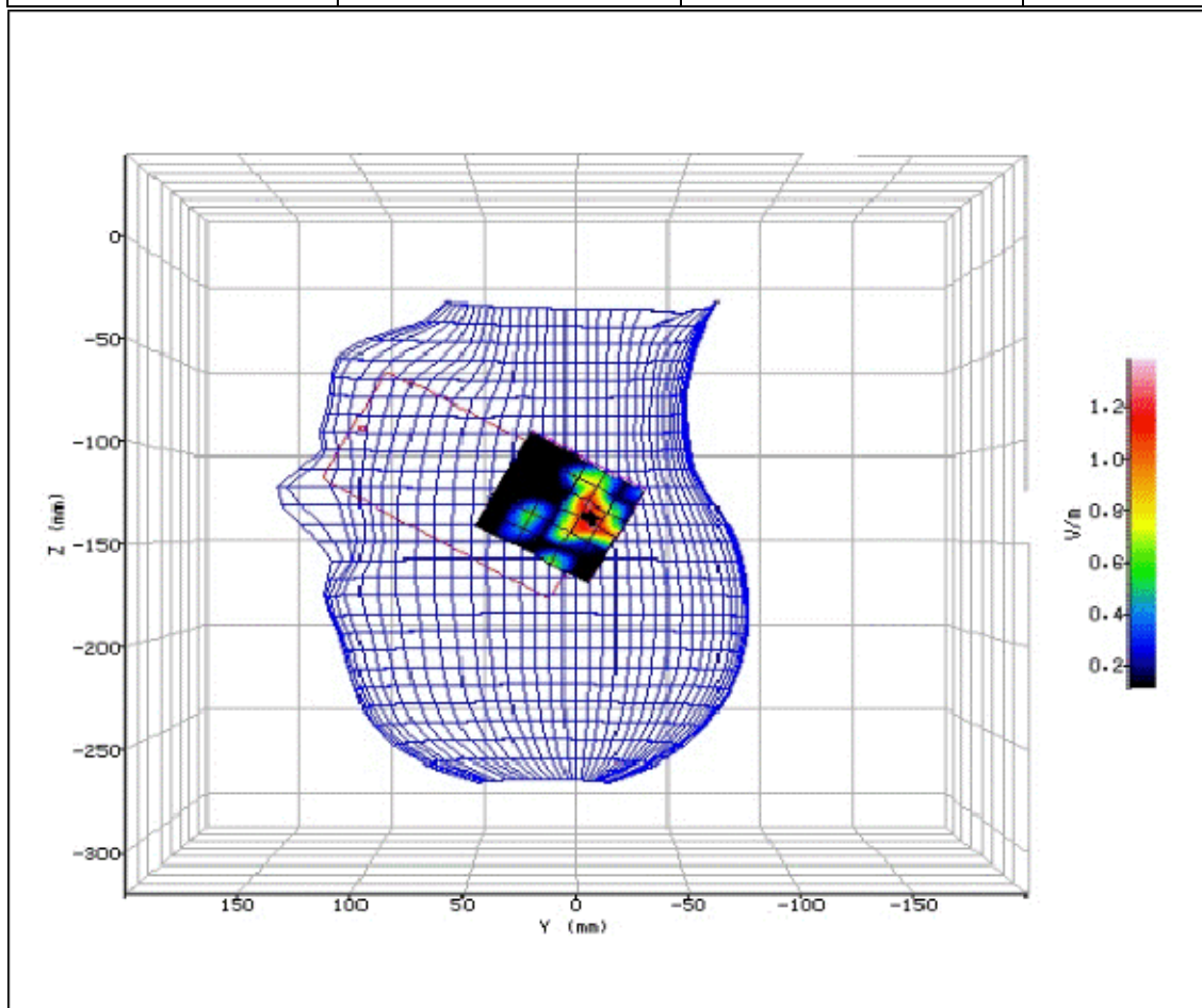
Figure 142: SAR Head Testing Results for the Sharp SHV32 Mobile Handset at 5280.0MHz. (NUA)
