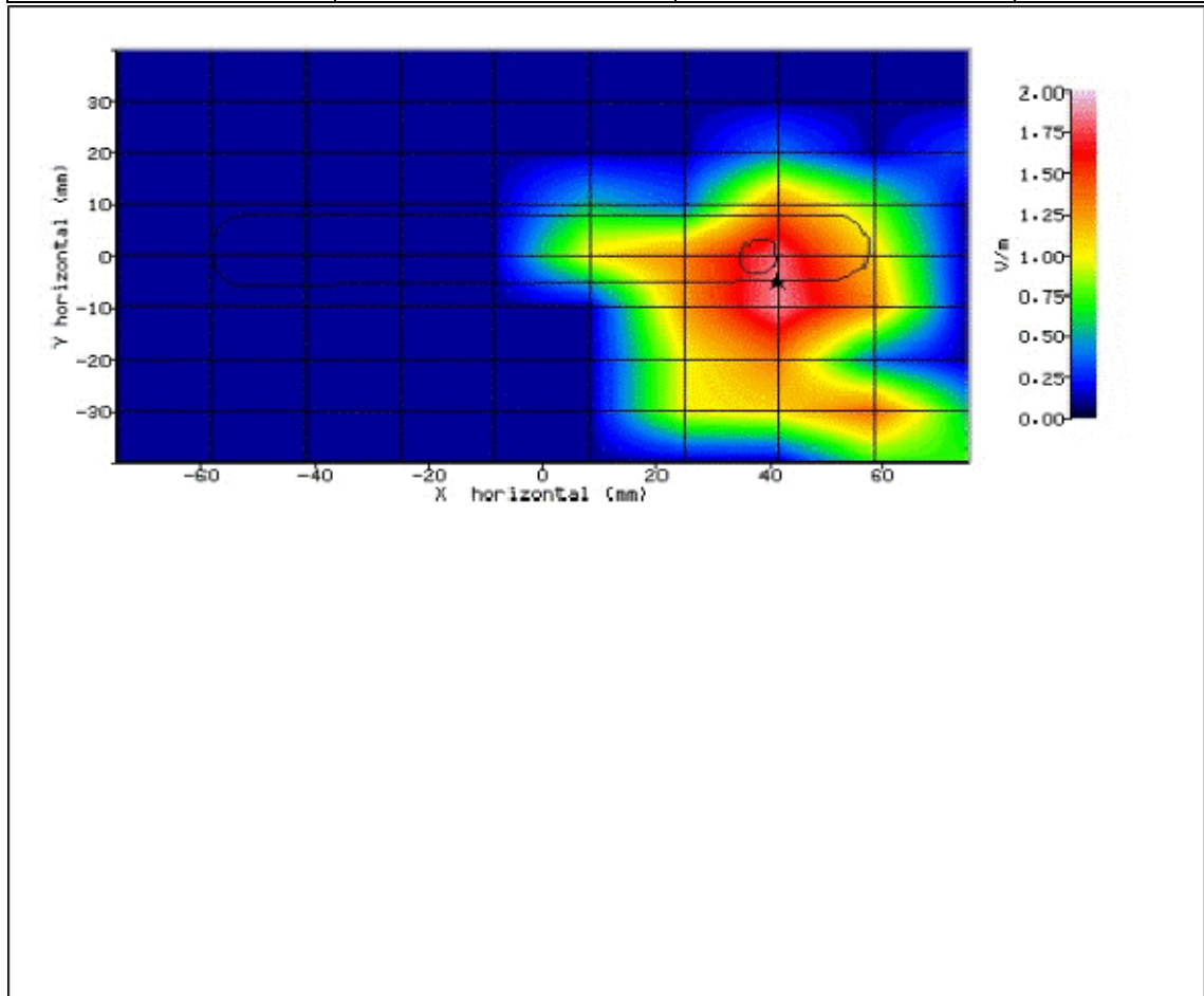
Figure 193: SAR Body Testing Results for the Sharp SHV32 Mobile Handset at 5270.0MHz. (NUA)
