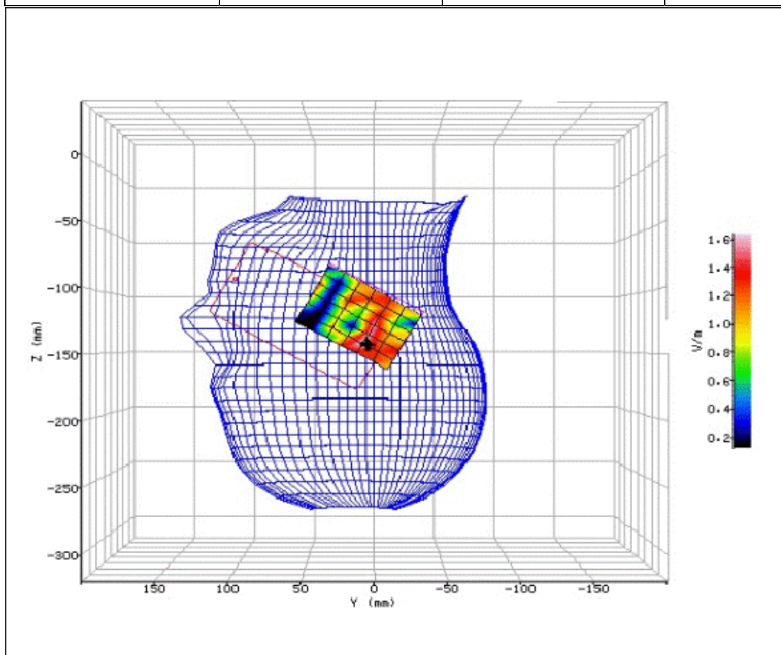
Figure 201: SAR Head Testing Results for the Sharp SHV32 Mobile Handset at 5590.0MHz. (NUA)
