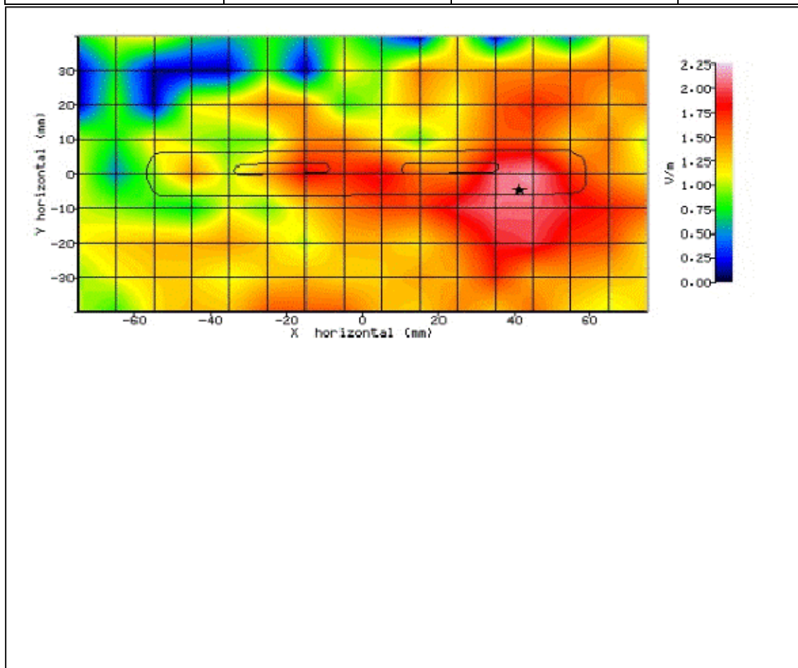
Figure 163: SAR Body Testing Results for the Sharp SHV32 Mobile Handset at 5600.0MHz. (NUA)
