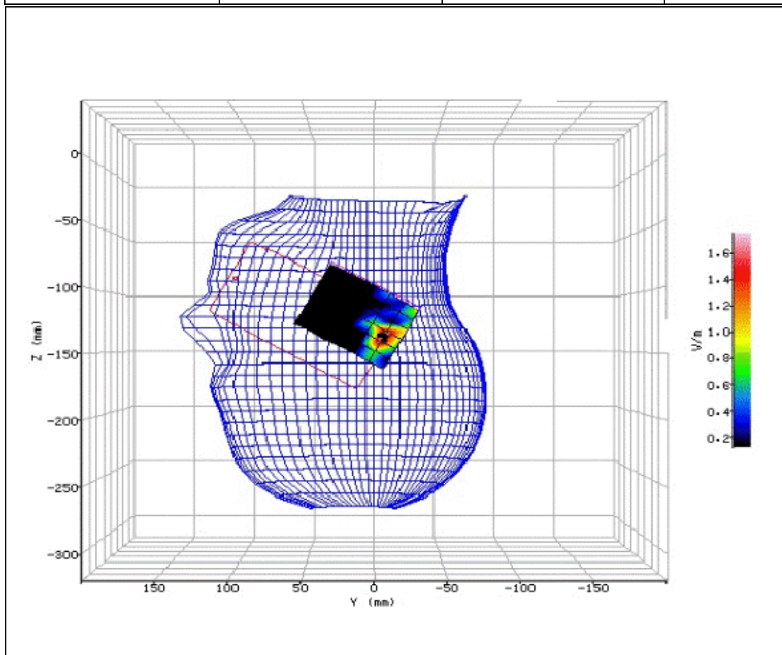
Figure 127: SAR Head Testing Results for the Sharp SHV32 Mobile Handset at 5180.0MHz. (NUA)
