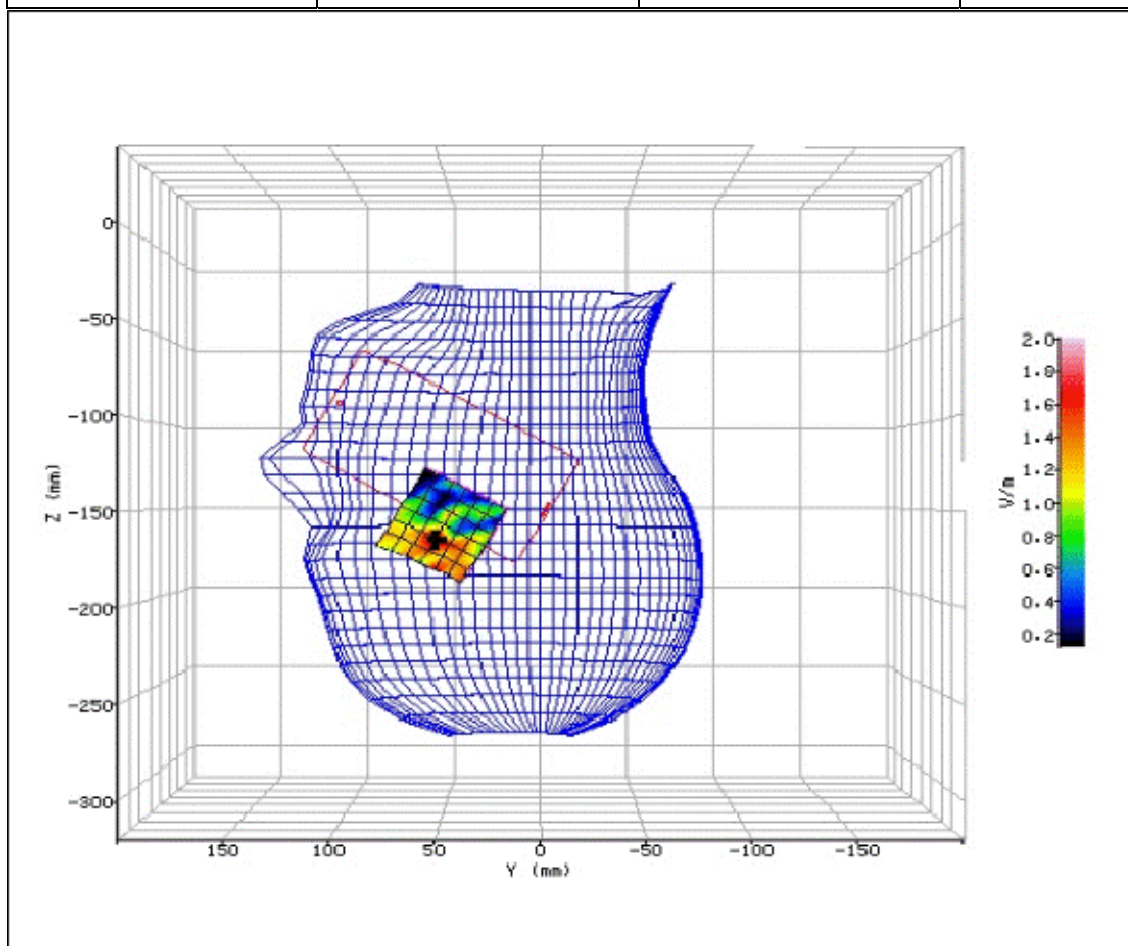
Figure 194: SAR Head Testing Results for the Sharp SHV32 Mobile Handset at 5270.0MHz. (NUA)
