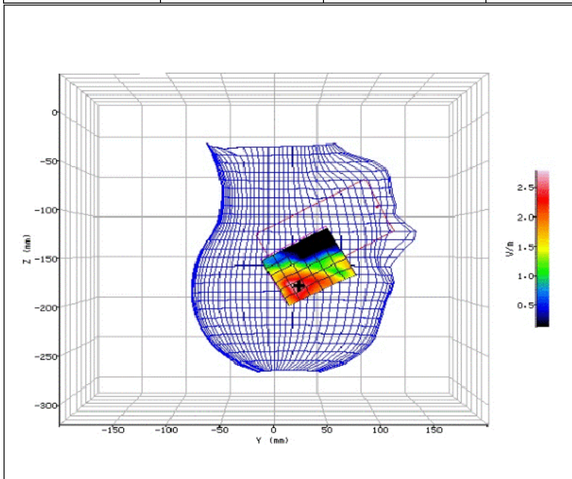
Figure 144: SAR Head Testing Results for the Sharp SHV32 Mobile Handset at 5280.0MHz. (NUA)
