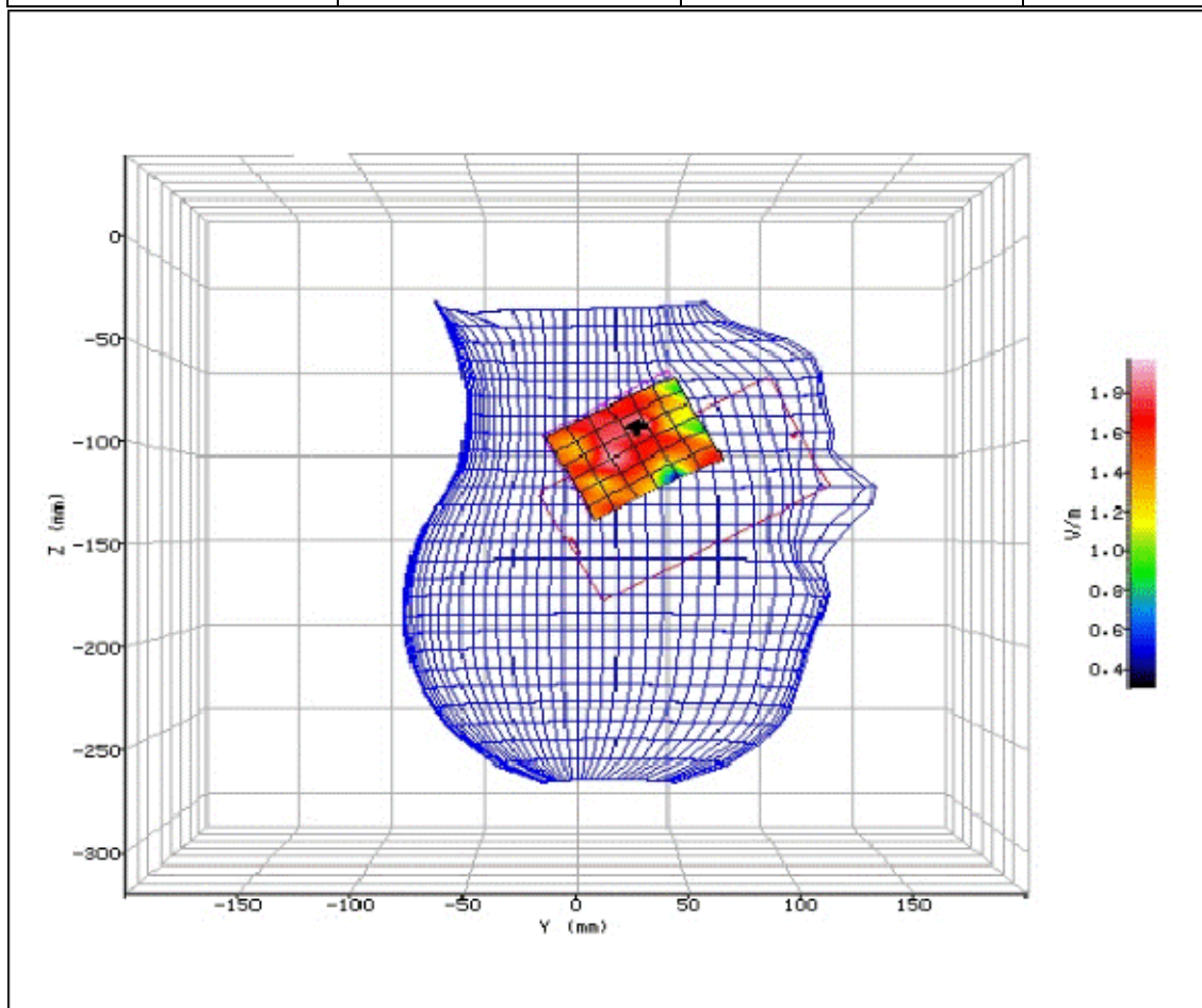
Figure 182: SAR Head Testing Results for the Sharp SHV32 Mobile Handset at 5190.0MHz. (NUA)
