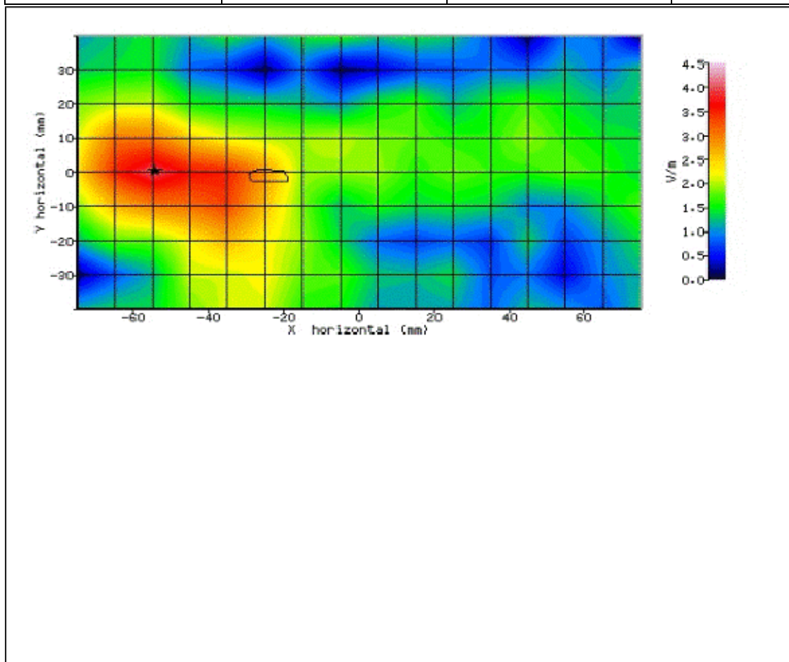
Figure 162: SAR Body Testing Results for the Sharp SHV32 Mobile Handset at 5600.0MHz. (NUA)
