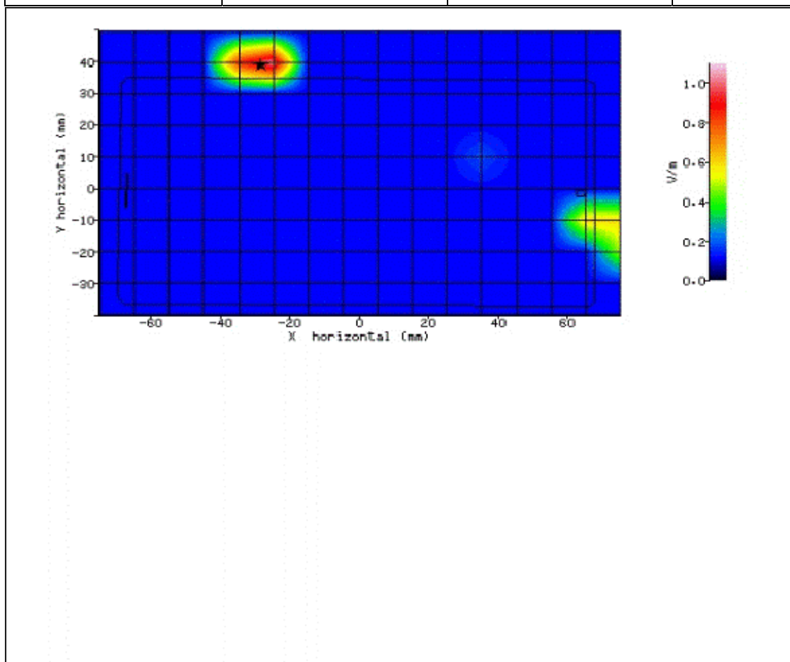
Figure 138: SAR Body Testing Results for the Sharp SHV32 Mobile Handset at 5180.0MHz. (NUA)
