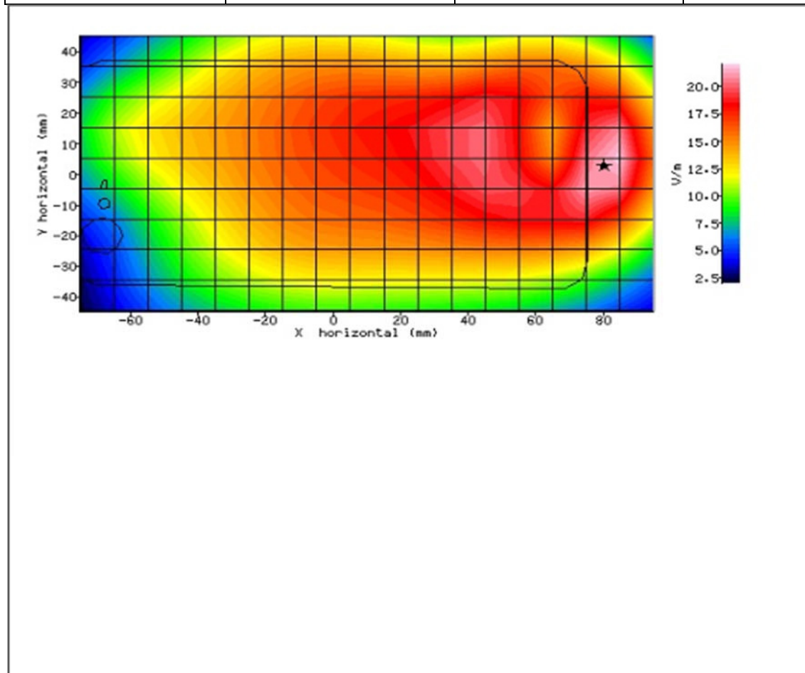
Figure 23: SAR Body Testing Results for the Sharp Smart phone at 826.4MHz.
