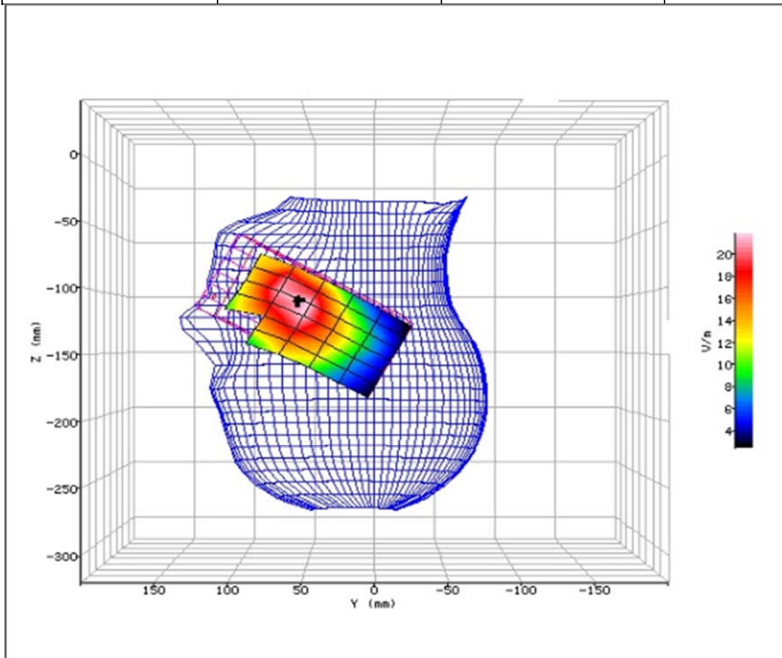
Figure 10: SAR Head Testing Results for the Sharp Smart phone at 824.2MHz.
