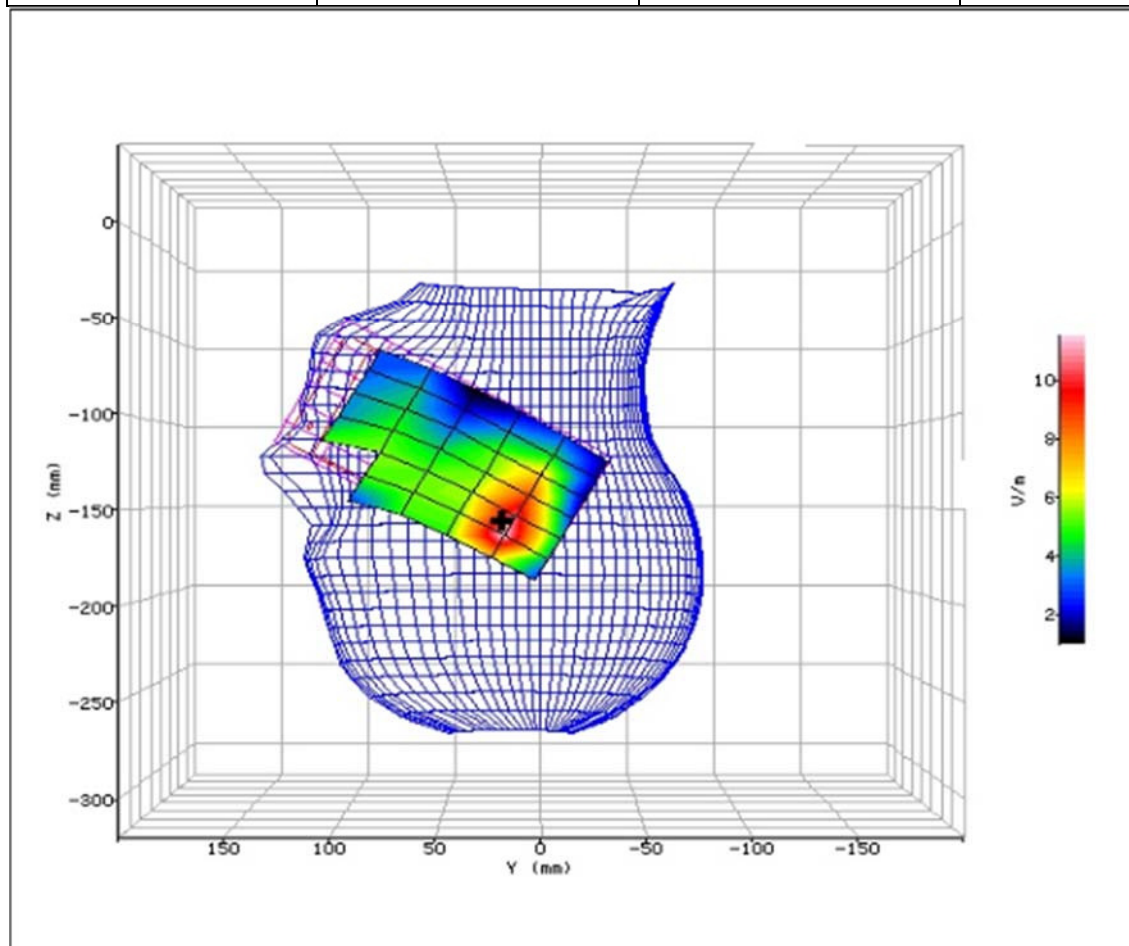
Figure 79: SAR Head Testing Results for the Sharp Smart phone at 1909.8MHz.
