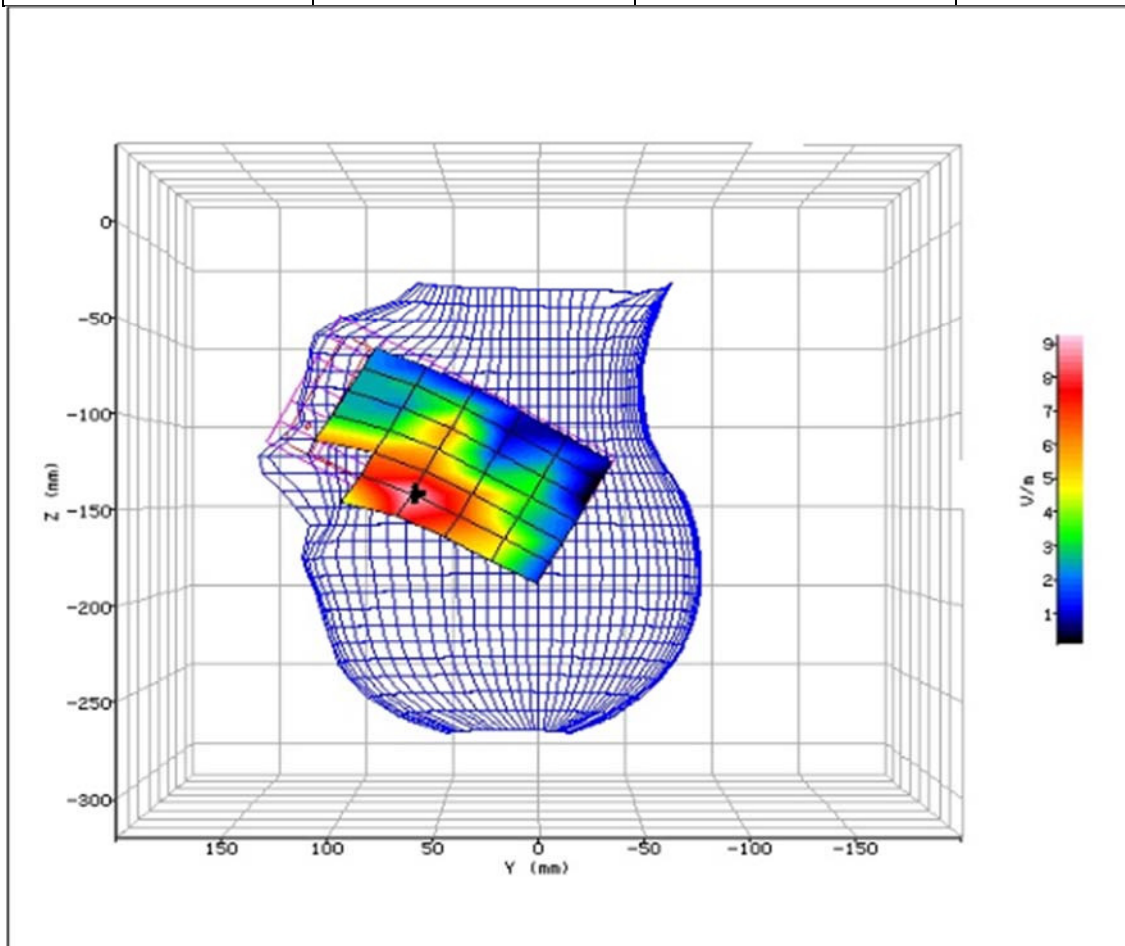
Figure 94: SAR Head Testing Results for the Sharp Smart phone at 2595.0MHz.
