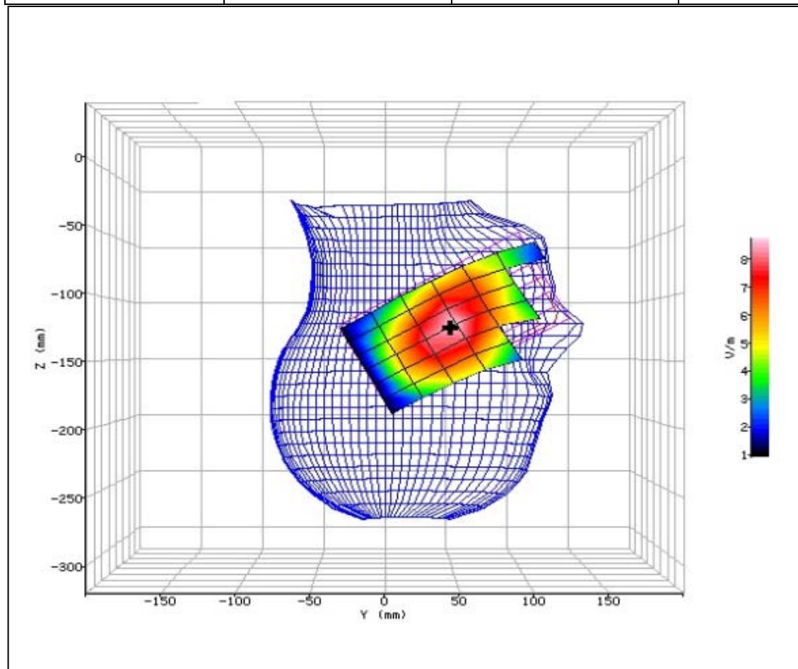
Figure 31: SAR Head Testing Results for the Sharp Smart phone at 709.0MHz.
