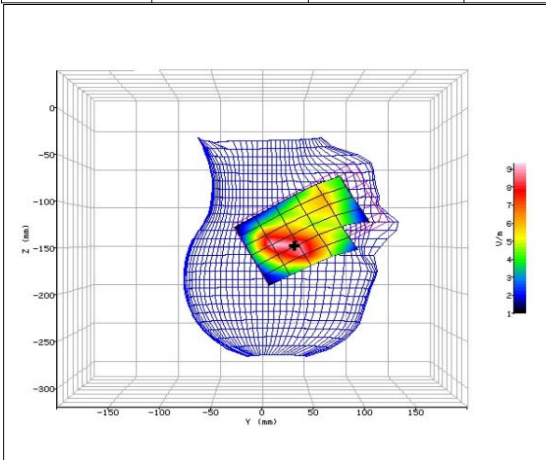
Figure 49: SAR Head Testing Results for the Sharp Smart phone at 1909.8MHz.
