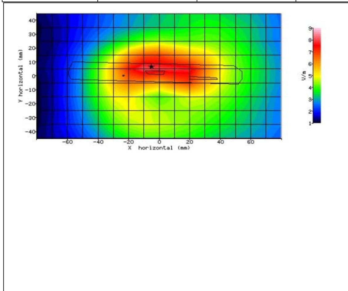
Figure 27: SAR Body Testing Results for the Sharp Smart phone at 835MHz.
