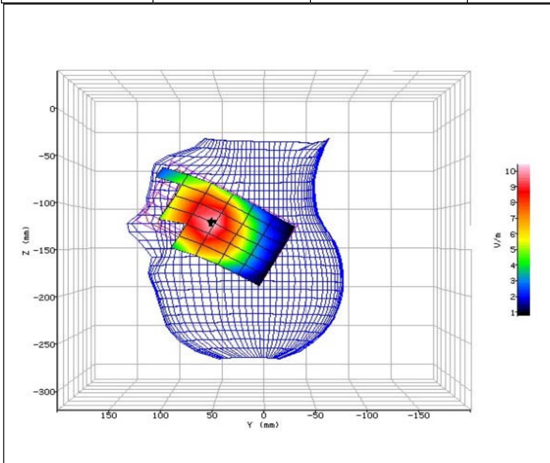
Figure 28: SAR Head Testing Results for the Sharp Smart phone at 709.0MHz.
