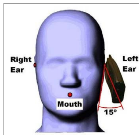
Figure 4 15° Tilt Position
