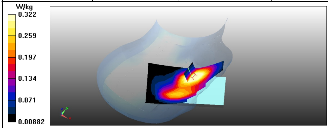
Figure 26: SAR Head Testing Results for the Sharp Smart phone at 1850.2 MHz.
