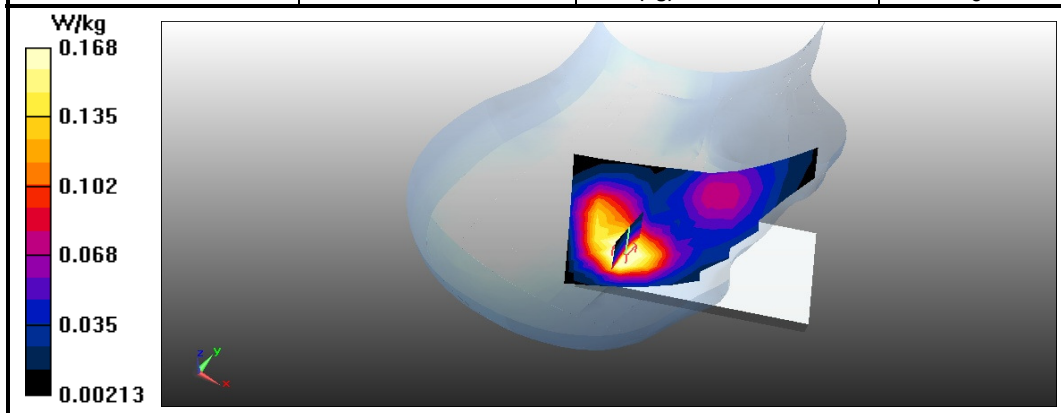
Figure 27 SAR Head Testing Results for the Sharp Smart phone at 1850.2 MHz.
