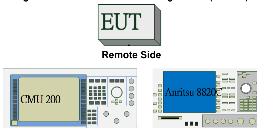
Fig. 2-2 Radiated Emission Configuration (WWAN)
