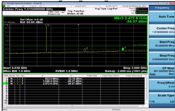
30MHz~3GHz GPRS 850MHz LowCH128-824.2
