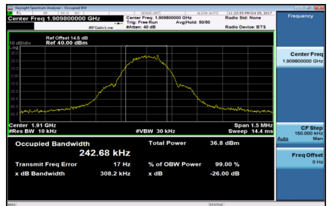
GPRS_1900MHz_HighCH810-1909.8
