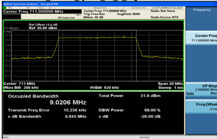
Band17_10MHz_QPSK_50_0_HighCH23800-711
