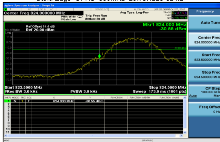
Band Edge GPRS 850MHz LowCH128-824.2
