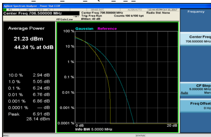
LTE_Band17_5MHz_16QAM_25_0_Channel Low
