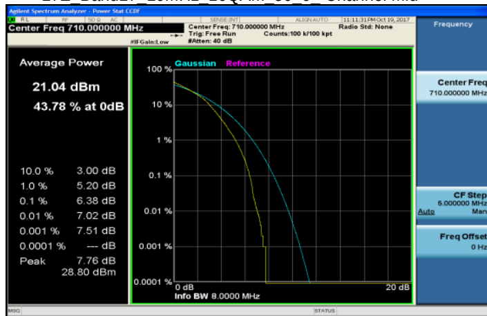
LTE_Band17_10MHz_16QAM_50_0_Channel Mid
