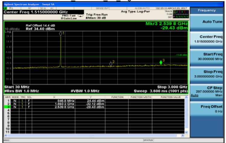
30MHz~3GHz WCDMA B5 HighCH4233-846.6
