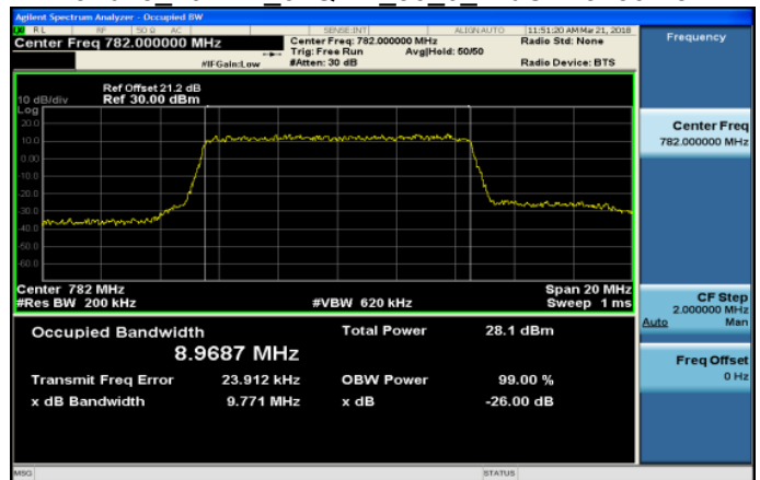
Band13 10MHz 64QAM 50 0 MidCH23230-782
