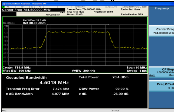
Band13 5MHz 64QAM 25 0 HighCH23255-784.5
