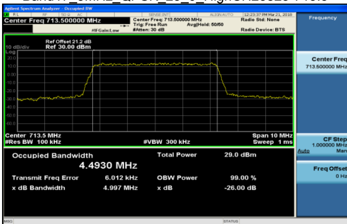
Band17 5MHz QPSK 25 0 HighCH23825-713.5
