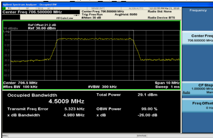
Band17 5MHz QPSK 25 0 LowCH23755-706.5
