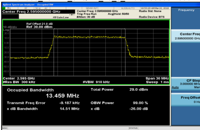
Band38 15MHz 64QAM 75 0 MidCH38000-2595
