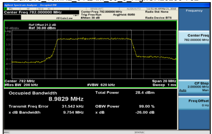
Band13 10MHz 64QAM 50 0 HighCH23230-782
