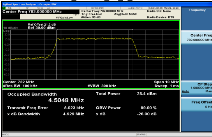
Band13 5MHz 64QAM 25 0 MidCH23230-782
