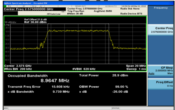
Band38 10MHz 64QAM 50 0 LowCH37800-2575
