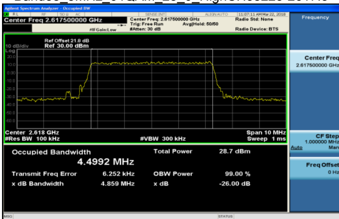
Band38 5MHz 64QAM 25 0 HighCH38225-2617.5
