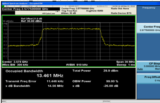
Band38 15MHz QPSK 75 0 LowCH37825-2577.5
