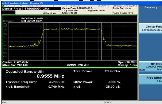
Band38 10MHz 16QAM 50 0 LowCH37800-2575
