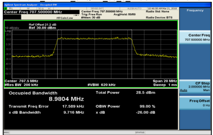
Band12 10MHz 64QAM 50 0 MidCH23095-707.5
