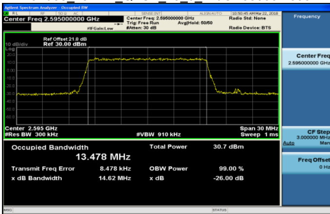
Band38 15MHz QPSK 75 0 MidCH38000-2595
