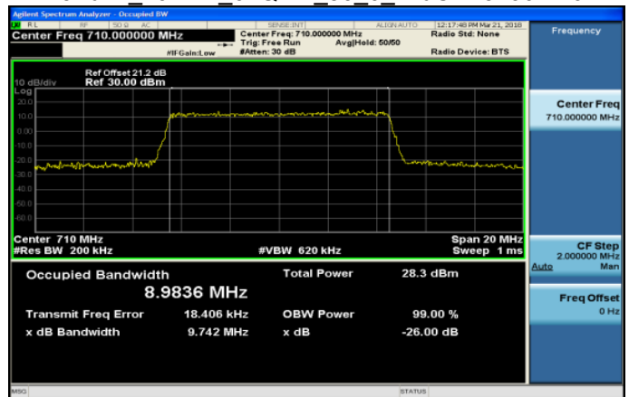
Band17 10MHz 64QAM 50 0 MidCH23790-710
