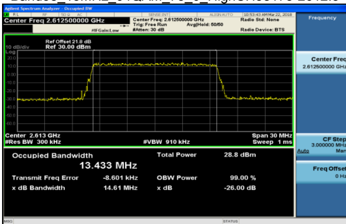
Band38 15MHz 64QAM 75 0 HighCH38175-2612.5
