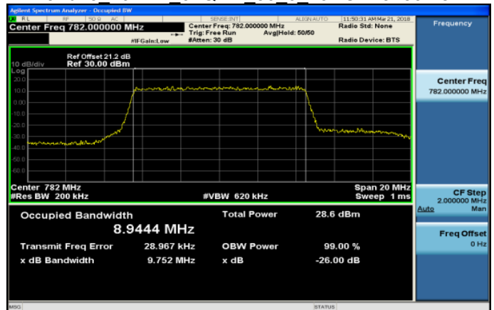
Band13 10MHz 64QAM 50 0 LowCH23230-782
