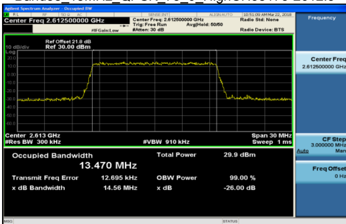
Band38 15MHz QPSK 75 0 HighCH38175-2612.5
