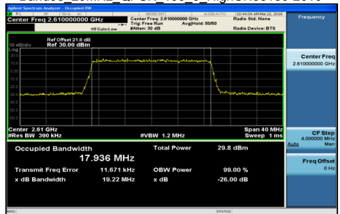
Band38 20MHz QPSK 100 0 HighCH38150-2610
