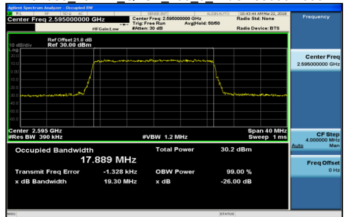
Band38 20MHz QPSK 100 0 MidCH38000-2595
