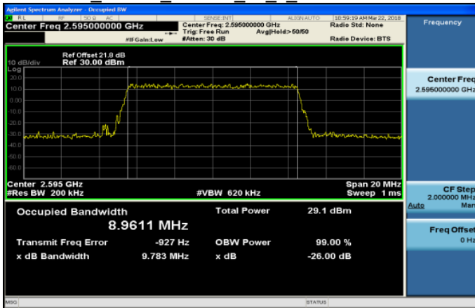
Band38 10MHz 16QAM 50 0 MidCH38000-2595
