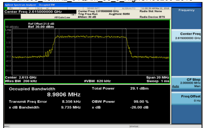
Band38 10MHz 64QAM 50 0 HighCH38200-2615
