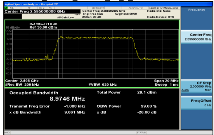
Band38 10MHz 64QAM 50 0 MidCH38000-2595
