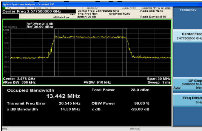
Band38 15MHz 64QAM 75 0 LowCH37825-2577.5
