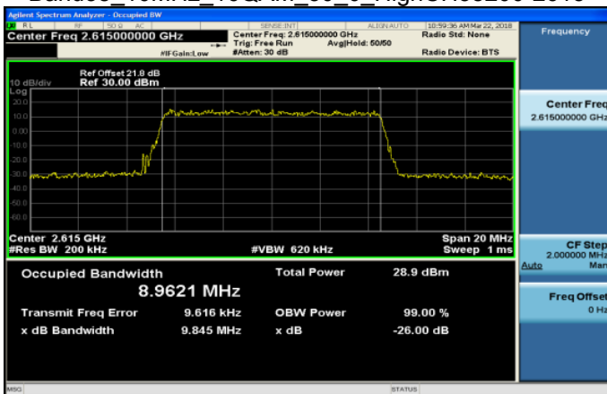
Band38 10MHz 16QAM 50 0 HighCH38200-2615
