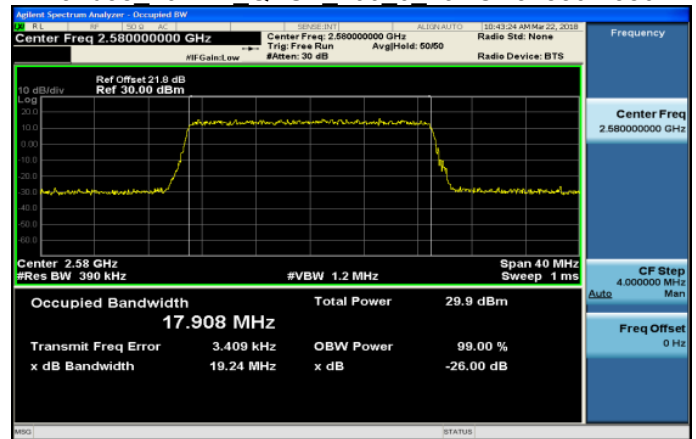
Band38 20MHz QPSK 100 0 LowCH37850-2580
