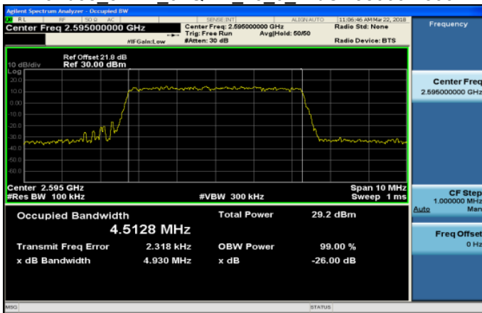
Band38 5MHz 64QAM 25 0 MidCH38000-2595
