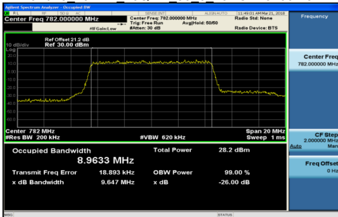
Band13 10MHz 16QAM 50 0 LowCH23230-782
