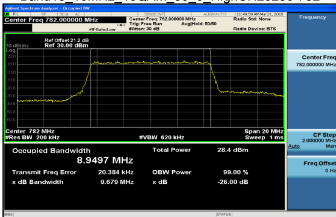
Band13 10MHz 16QAM 50 0 HighCH23230-782
