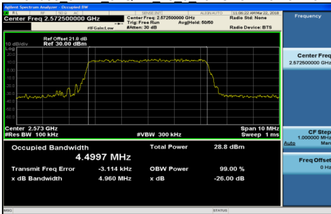
Band38 5MHz 64QAM 25 0 LowCH37775-2572.5
