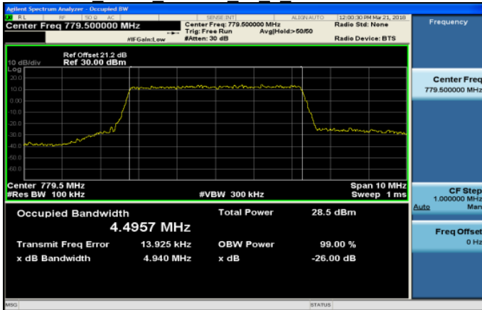
Band13 5MHz 64QAM 25 0 LowCH23205-779.5
