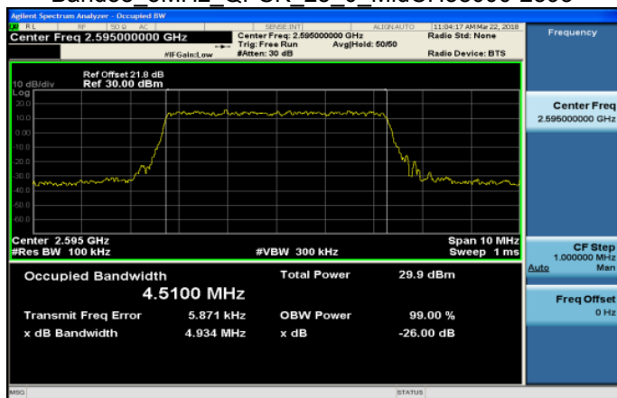
Band38 5MHz QPSK 25 0 MidCH38000-2595
