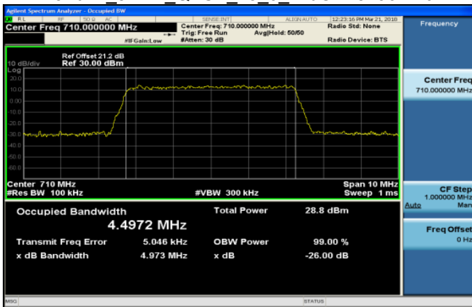
Band17 5MHz QPSK 25 0 MidCH23790-710
