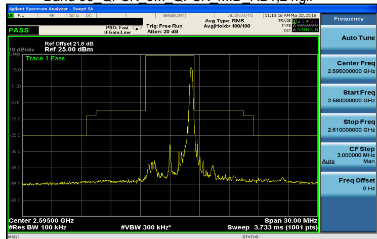
Band 38_QPSK_5M_QPSK_MID_RB25,0.gif
