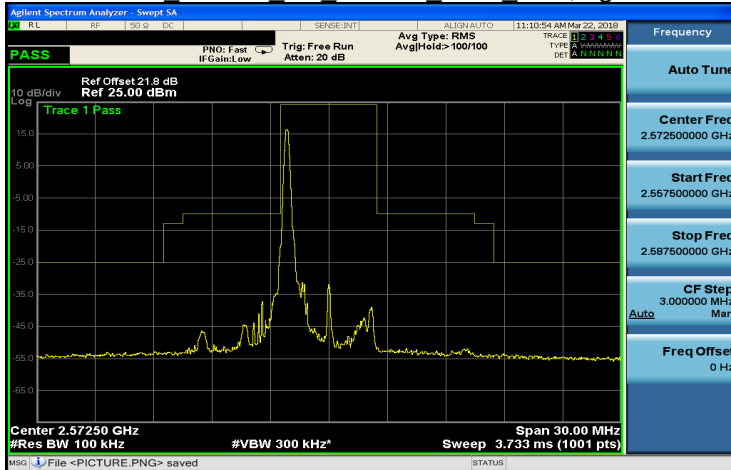
Band 38 64QAM 5M 64QAM LOW RB1,24.gif
