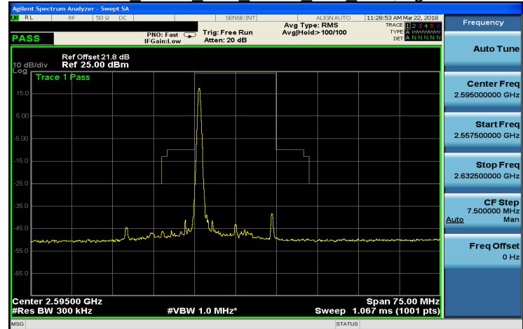
Band 38 QPSK 15M QPSK MID RB1,74.gif
