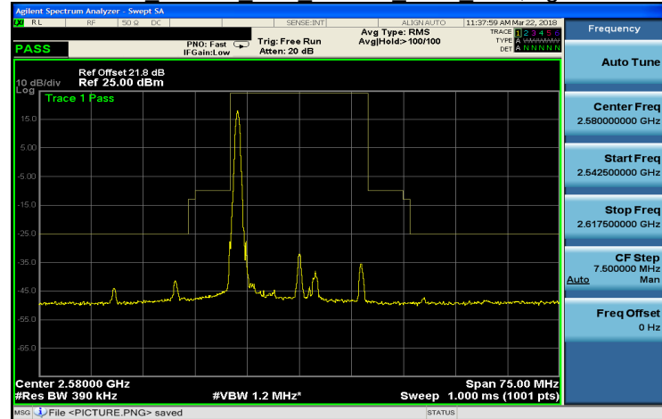
Band 38 64QAM 20M 64QAM LOW RB1,99.gif
