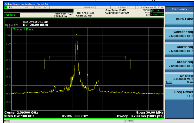
Band 38_QPSK_5M_QPSK_MID_RB1,24.gif
