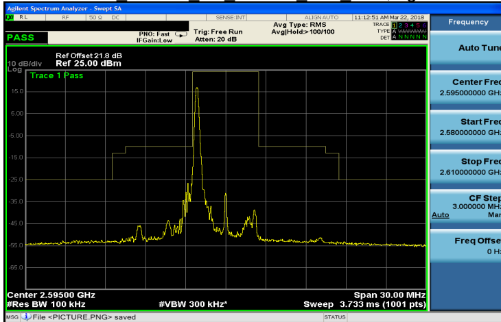
Band 38 16QAM 5M 16QAM MID RB1,24.gif
