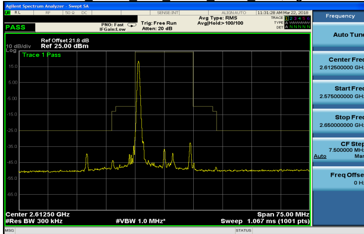
Band 38 QPSK 15M QPSK HIGH RB1,74.gif
