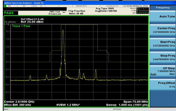
Band 38 QPSK 20M QPSK HIGH RB1,99.gif
