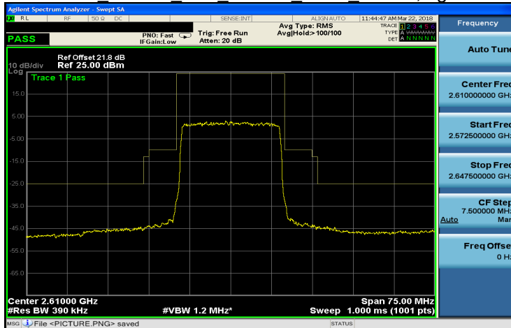
Band 38 16QAM 20M 16QAM HIGH RB100,0.gif
