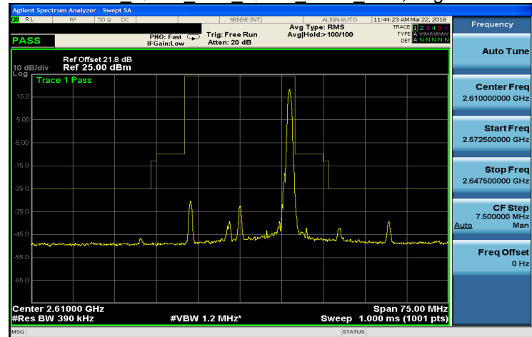
Band 38 QPSK 20M QPSK HIGH RB100,0.gif
