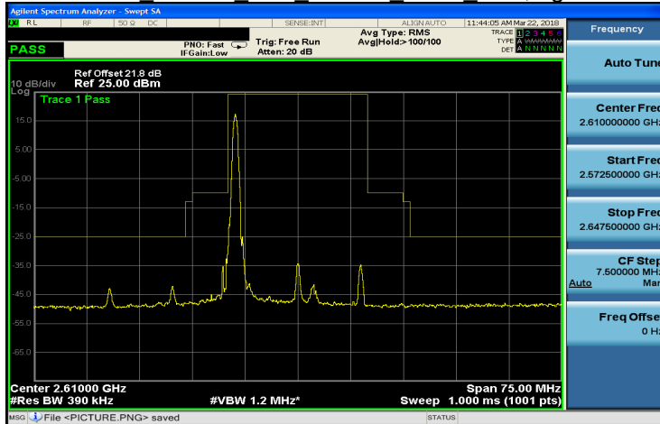
Band 38 16QAM 20M 16QAM HIGH RB1,99.gif
