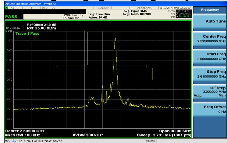
Band 38 64QAM 5M 64QAM MID RB25,0.gif
