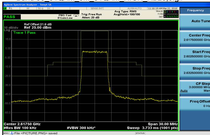
Band 38 64QAM 5M 64QAM HIGH RB25,0.gif
