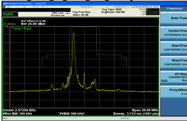
Band 38_QPSK_5M_QPSK_LOW_RB1,24.gif
