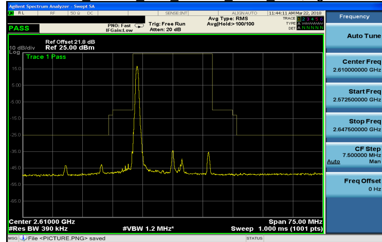
Band 38 64QAM 20M 64QAM HIGH RB1,99.gif
