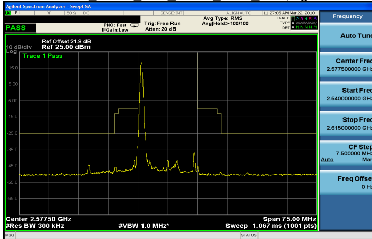
Band 38 QPSK 15M QPSK LOW RB1,74.gif
