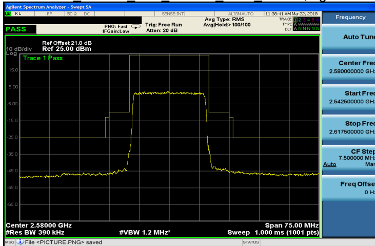
Band 38 16QAM 20M 16QAM LOW RB100,0.gif
