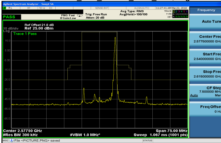
Band 38 64QAM 15M 64QAM LOW RB75,0.gif
