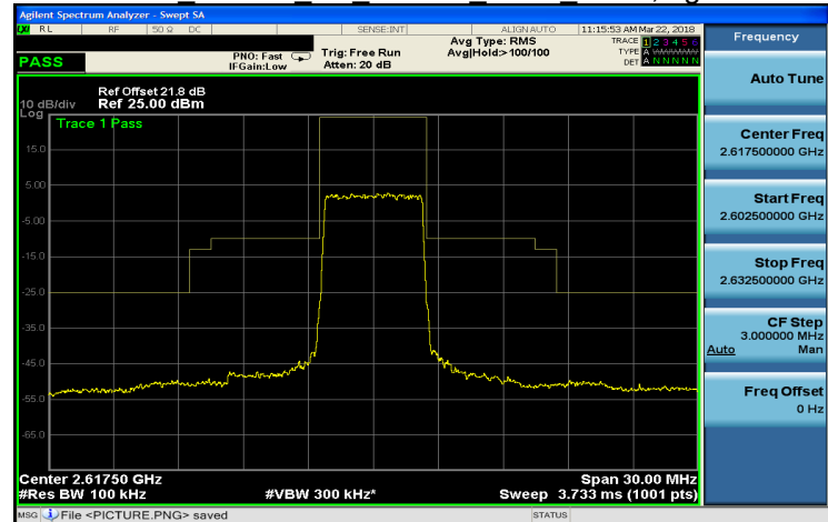
Band 38 16QAM 5M 16QAM HIGH RB25,0.gif
