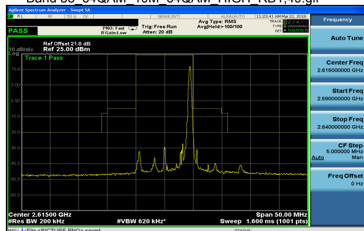
Band 38 64QAM 10M 64QAM HIGH RB50,0.gif
