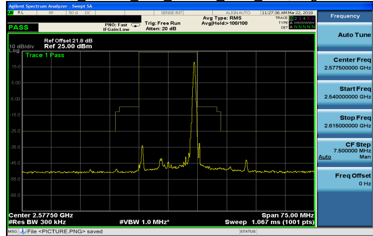
Band 38 16QAM 15M 16QAM LOW RB75,0.gif
