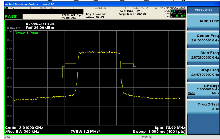
Band 38 QPSK 20M QPSK HIGH RB100,0.gif
