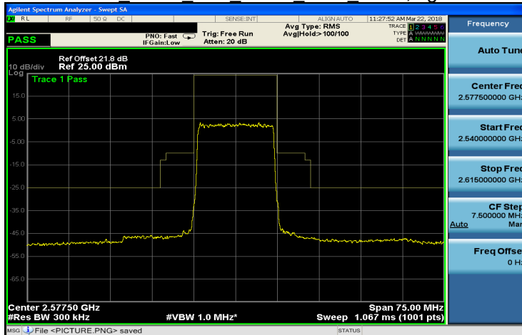
Band 38 QPSK 15M QPSK LOW RB75,0.gif
