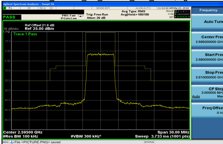
Band 38 16QAM 5M 16QAM MID RB25,0.gif
