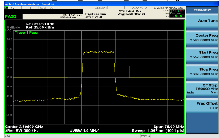
Band 38 QPSK 15M QPSK MID RB75,0.gif
