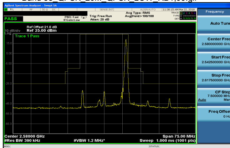
Band 38 QPSK 20M QPSK LOW RB100,0.gif
