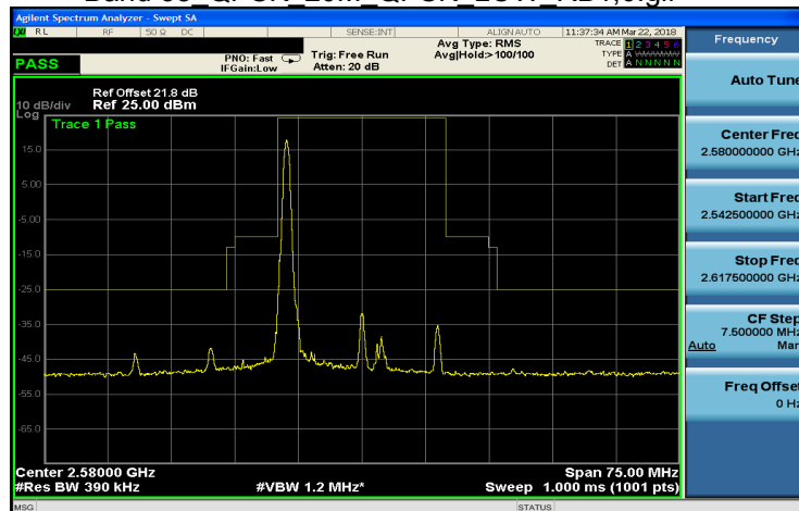
Band 38 QPSK 20M QPSK LOW RB1,99.gif
