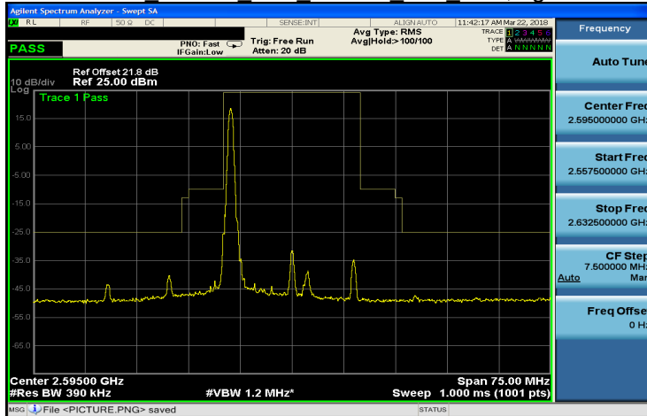
Band 38 64QAM 20M 64QAM MID RB1,99.gif
