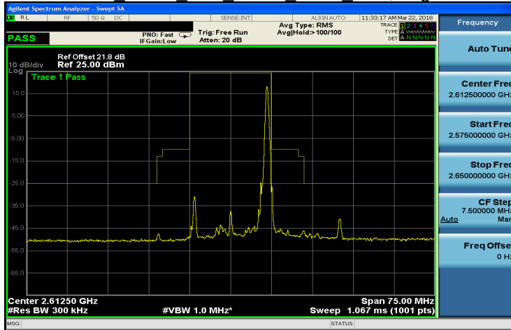
Band 38 QPSK 15M QPSK HIGH RB75,0.gif
