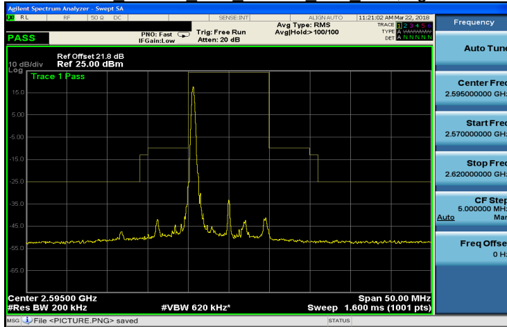
Band 38 64QAM 10M 64QAM MID RB1,49.gif
