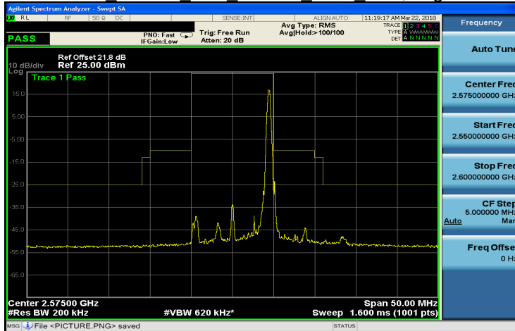
Band 38 16QAM 10M 16QAM LOW RB50,0.gif
