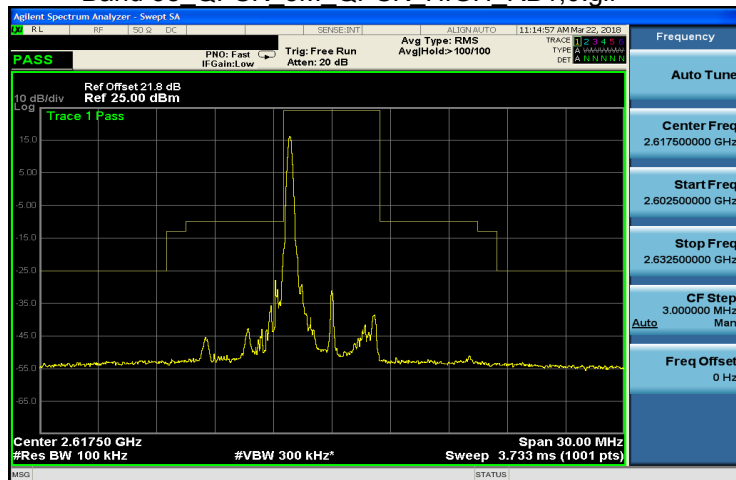
Band 38 QPSK 5M QPSK HIGH RB1,24.gif
