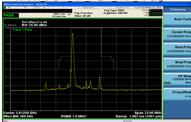
Band 38 64QAM 15M 64QAM HIGH RB1,74.gif
