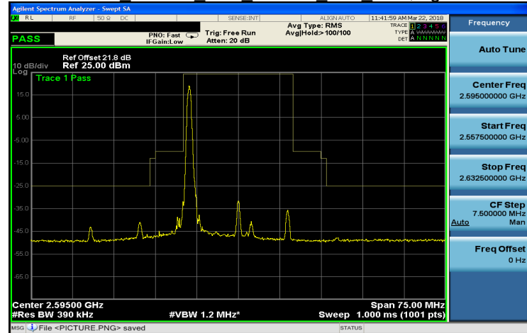
Band 38 16QAM 20M 16QAM MID RB1,99.gif
