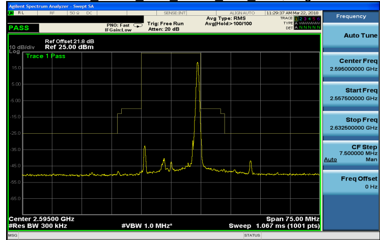
Band 38 QPSK 15M QPSK MID RB75,0.gif
