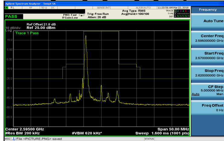
Band 38 16QAM 10M 16QAM MID RB1,49.gif
