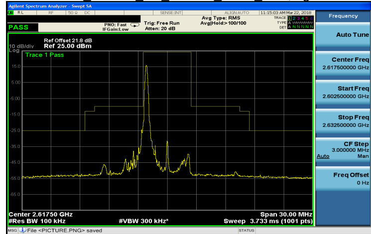
Band 38 16QAM 5M 16QAM HIGH RB1,24.gif
