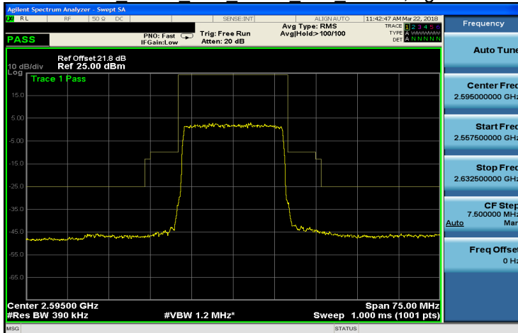
Band 38 QPSK 20M QPSK MID RB100,0.gif
