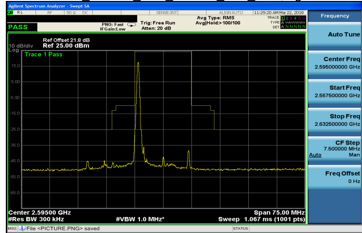
Band 38 64QAM 15M 64QAM MID RB1,74.gif
