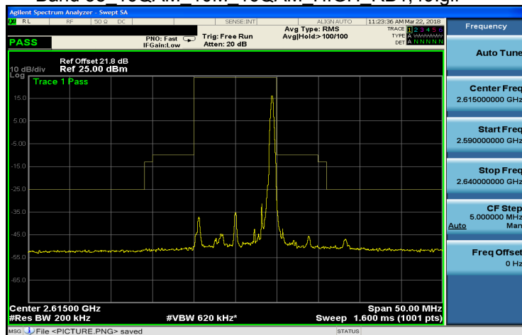
Band 38 16QAM 10M 16QAM HIGH RB50,0.gif
