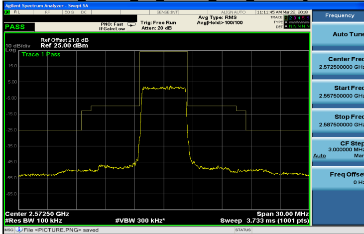
Band 38 64QAM 5M 64QAM LOW RB25,0.gif
