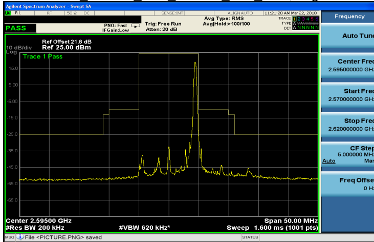
Band 38 64QAM 10M 64QAM MID RB50,0.gif
