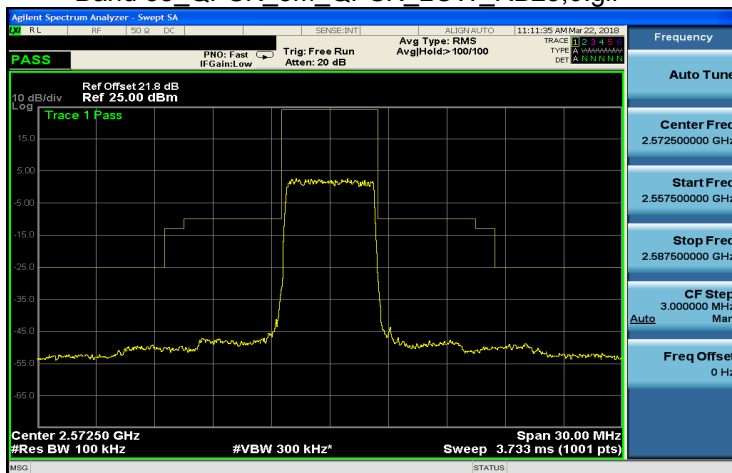
Band 38_QPSK_5M_QPSK_LOW_RB25,0.gif
