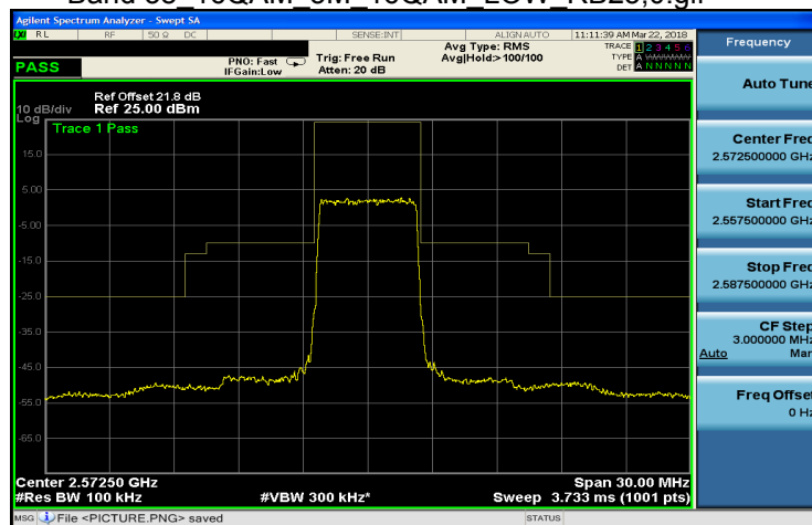
Band 38 16QAM 5M 16QAM LOW RB25,0.gif
