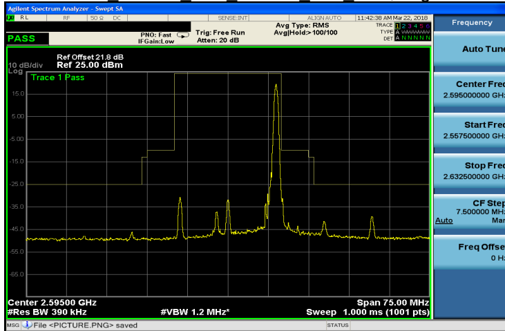
Band 38 64QAM 20M 64QAM MID RB100,0.gif
