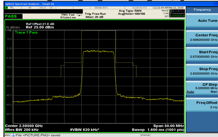
Band 38 16QAM 10M 16QAM MID RB50,0.gif
