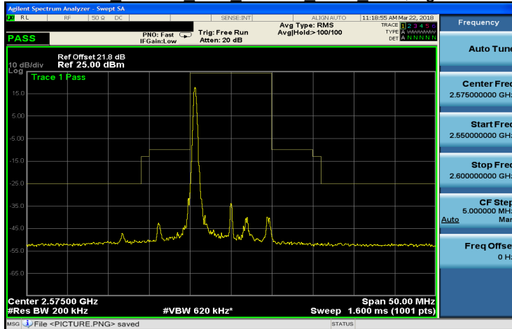
Band 38 16QAM 10M 16QAM LOW RB1,49.gif
