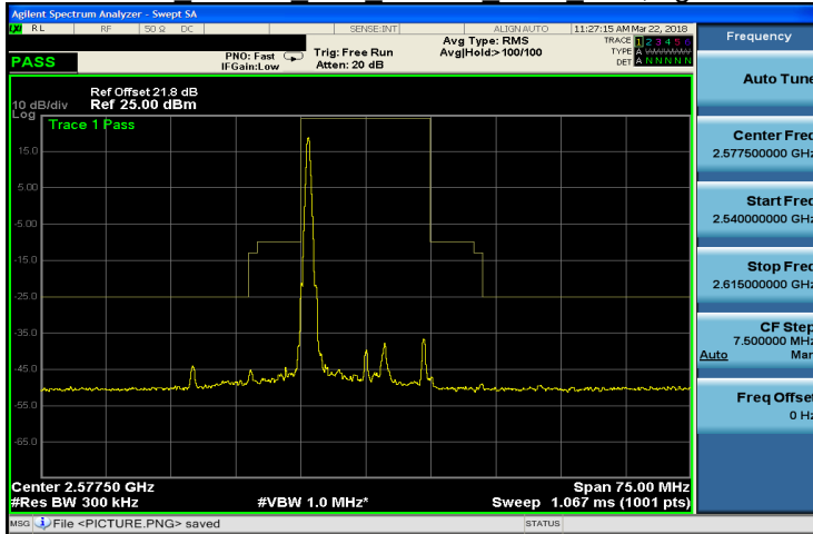
Band 38 64QAM 15M 64QAM LOW RB1,74.gif
