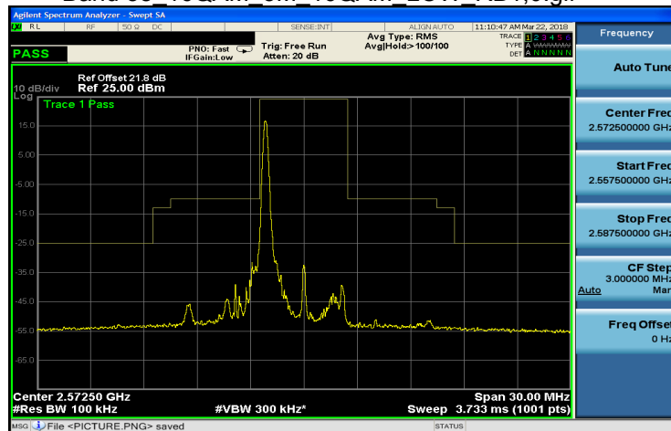
Band 38 16QAM 5M 16QAM LOW RB1,24.gif
