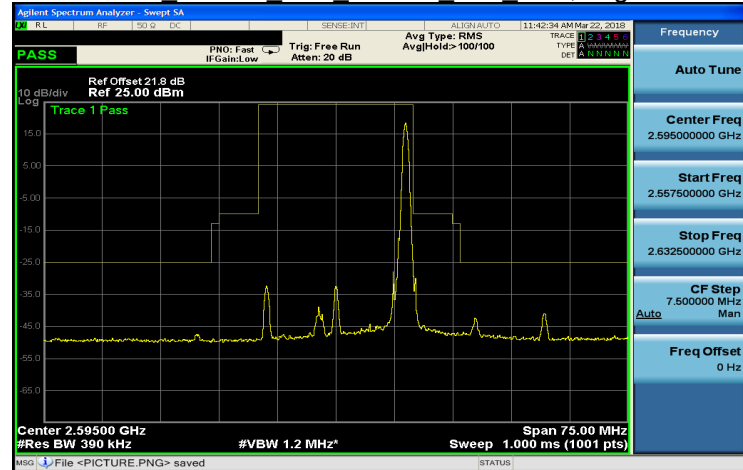
Band 38 16QAM 20M 16QAM MID RB100,0.gif
