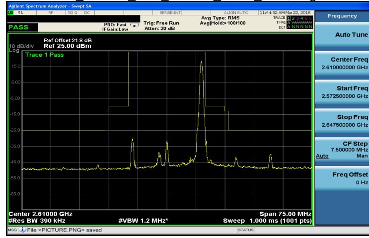
Band 38 64QAM 20M 64QAM HIGH RB100,0.gif
