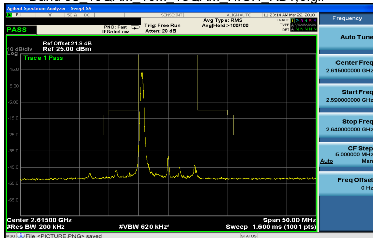
Band 38 16QAM 10M 16QAM HIGH RB1,49.gif
