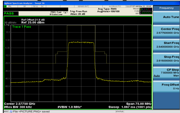
Band 38 16QAM 15M 16QAM LOW RB75,0.gif
