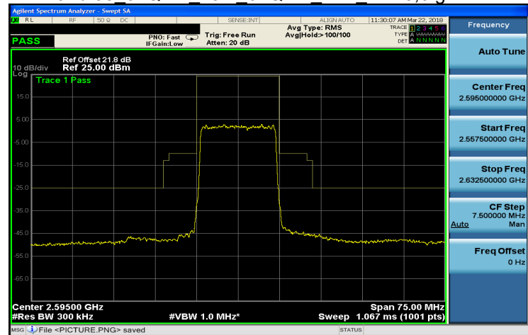
Band 38 64QAM 15M 64QAM MID RB75,0.gif
