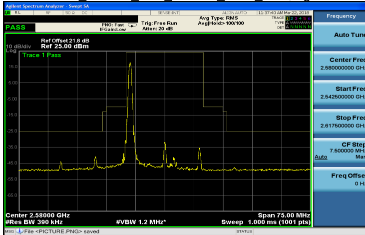
Band 38 16QAM 20M 16QAM LOW RB1,99.gif
