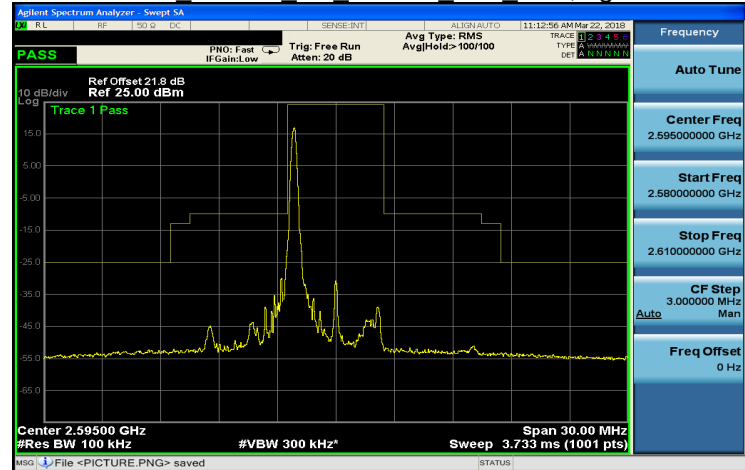
Band 38 64QAM 5M 64QAM MID RB1,24.gif
