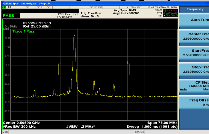
Band 38 QPSK 20M QPSK MID RB1,99.gif
