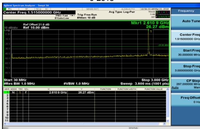
30MHz~3GHz_Band38_10MHz_QPSK_1_0_HighCH382000-2615
