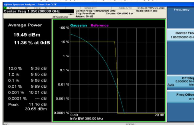
GSM_1900MHz_LowCH512-1850.2
