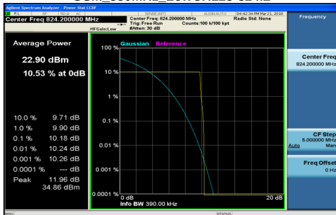
GSM_850MHz_LowCH128-824.2
