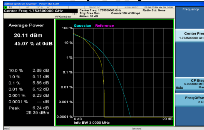
LTE_Band4_3MHz_64QAM_15_0_HighCH20385-1753.5
