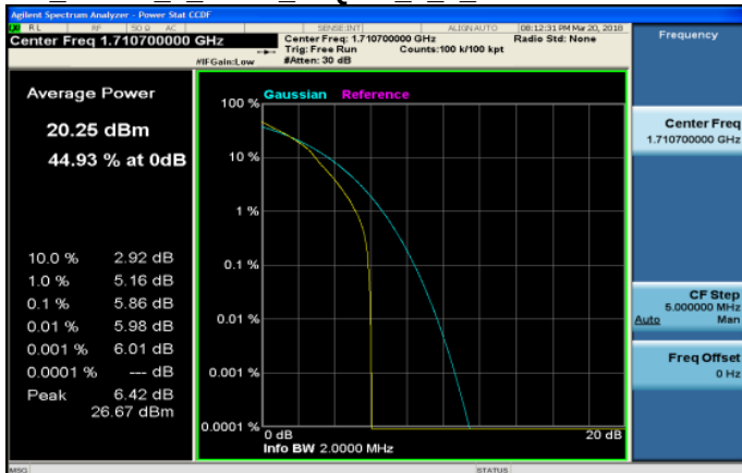
LTE_Band4_1_4MHz_64QAM_6_0_LowCH19957-1710.7
