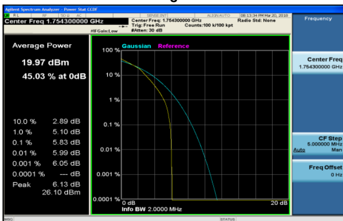
LTE_Band4_1_4MHz_64QAM_6_0_HighCH20393-1754.
