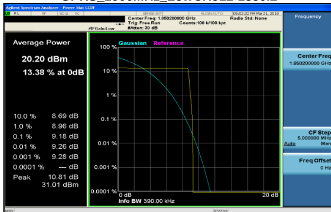
GPRS_1900MHz_LowCH512-1850.2
