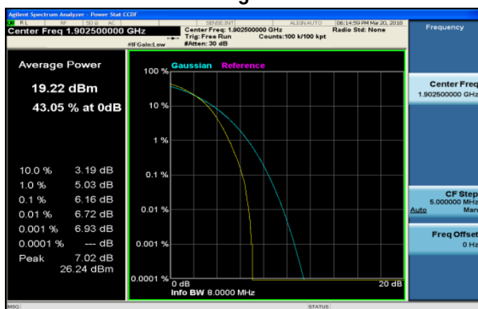
LTE_Band2_15MHz_64QAM_75_0_HighCH19125-1902.
