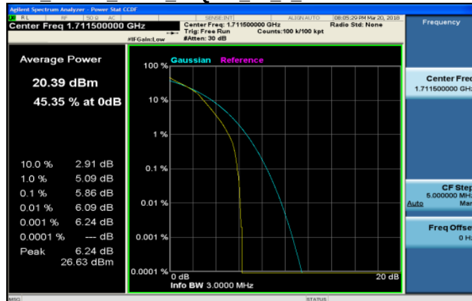
LTE_Band4_3MHz_64QAM_15_0_LowCH19965-1711.5
