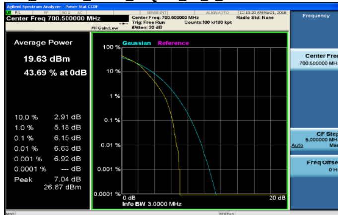
LTE_Band12_3MHz_64QAM_15_0_LowCH23025-700.5
