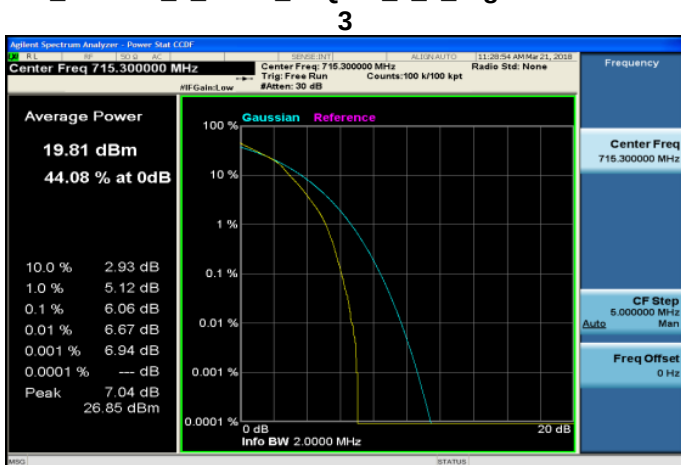
LTE_Band12_1_4MHz_64QAM_6_0_HighCH23173-715.
