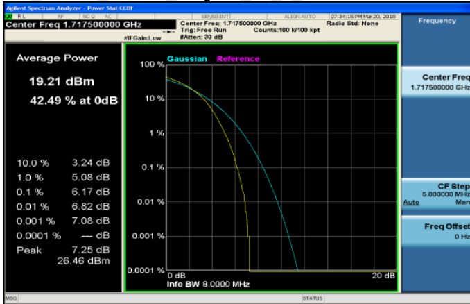
LTE_Band4_15MHz_64QAM_75_0_LowCH20025-1717.5
