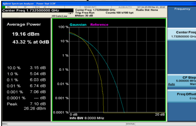
LTE_Band4_15MHz_64QAM_75_0_MidCH20175-1732.5
