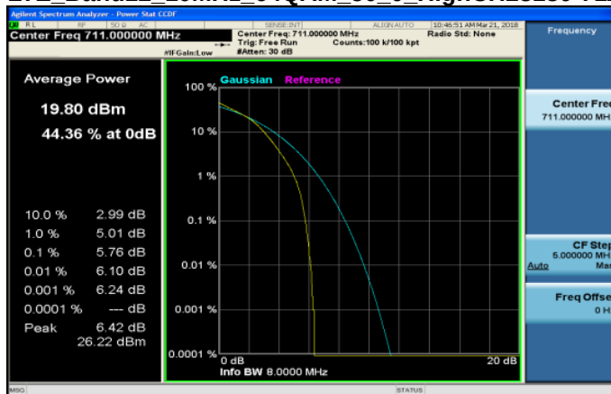
LTE_Band12 10MHz 64QAM 50 0 HighCH23130-711
