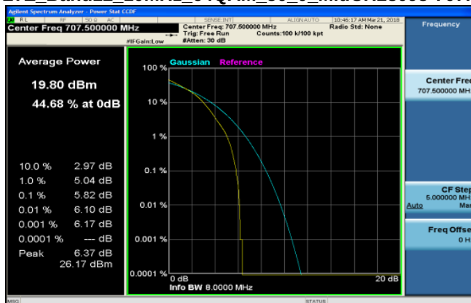
LTE_Band12 10MHz 64QAM 50 0 MidCH23095-707.5
