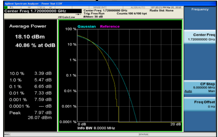
LTE_Band4_20MHz_64QAM_100_0_LowCH20050-1720
