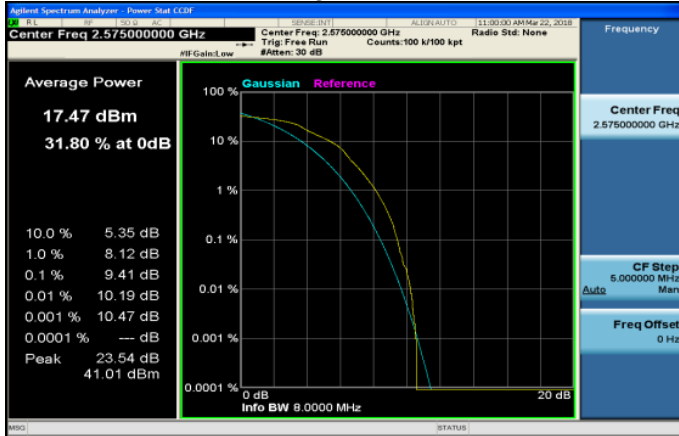
LTE_Band38_10MHz_64QAM_50_0_LowCH37800-2575
