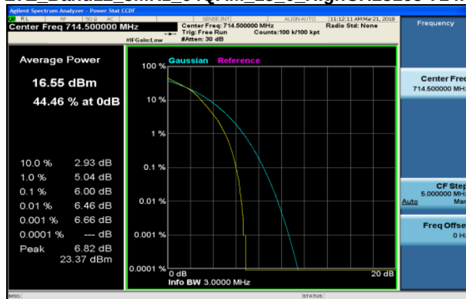
LTE_Band12_3MHz_64QAM_15_0_HighCH23165-714.5
