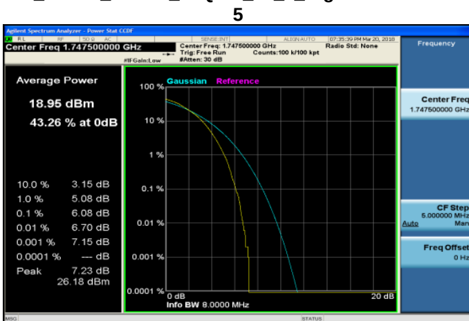
LTE_Band4_15MHz_64QAM_75_0_HighCH20325-1747.5
