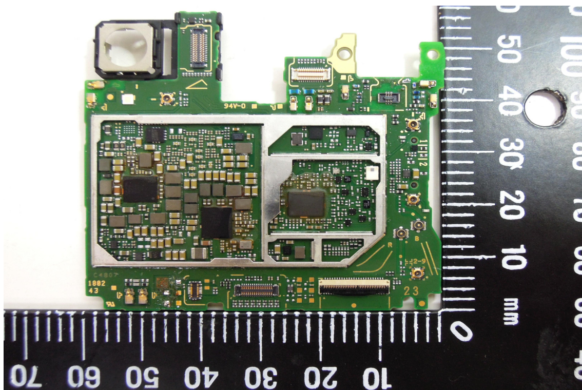
Internal View of EUT –4 (Model A)
