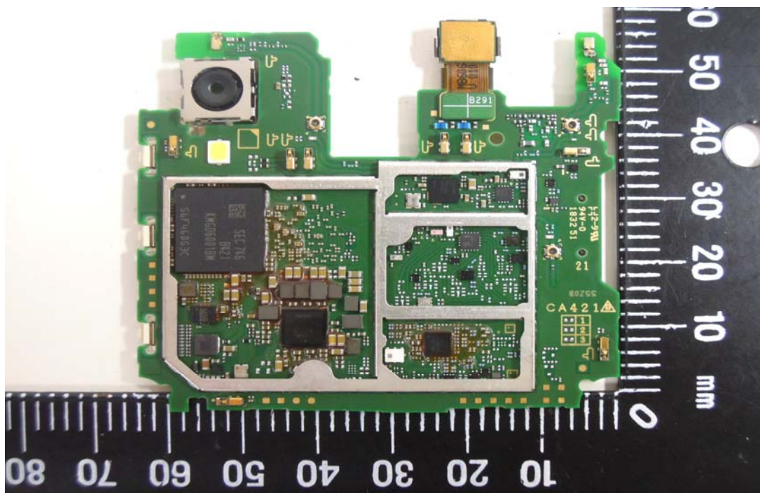
Internal View of EUT -6
