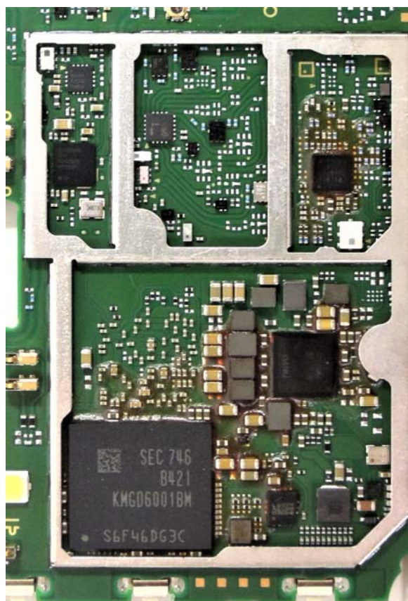
Internal View of EUT -6
