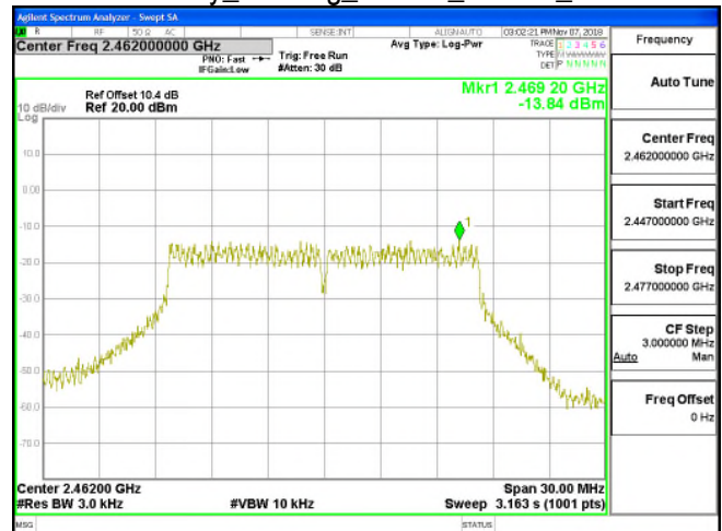
Power Density_802.11g_20MHz_Chain0_2462MHz
