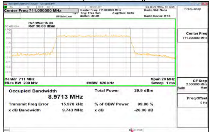
Band17 10MHz 16QAM 50 0 Main HighCH23800-711
