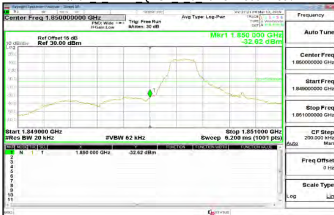
LTE\Band2 1 4MHz QPSK 1 0 LowCH18607-1850.7
