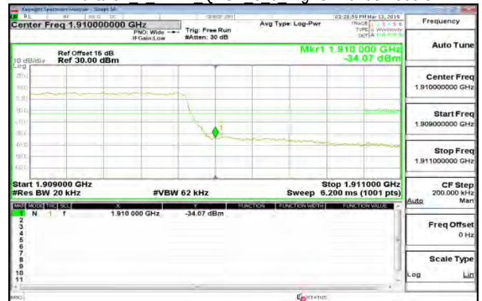
LTE\Band2 1 4MHz QPSK 6 0 HighCH19193-1909.3
