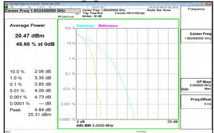
HSDPA B2 LowCH9262-1852.4
