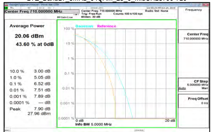
LTE Band17 5MHz 64QAM 25 0 MidCH23790-710
