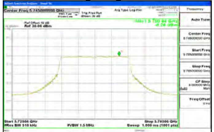
802.11a_20MHz_5745MHz
