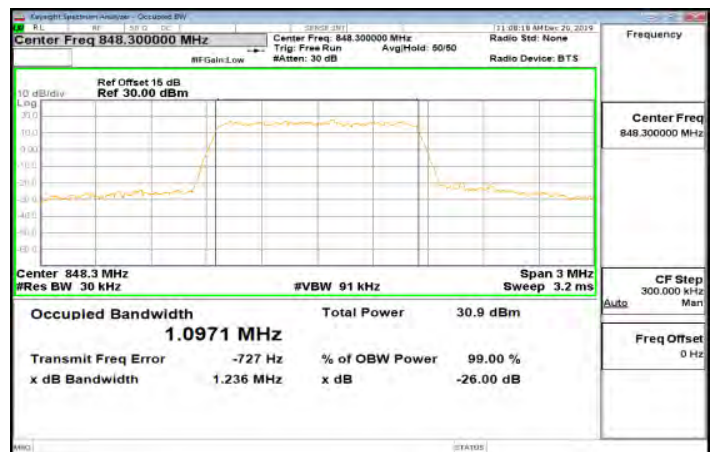
Band5_1_4MHz_QPSK_6_0_Main_HighCH20643-848.3
