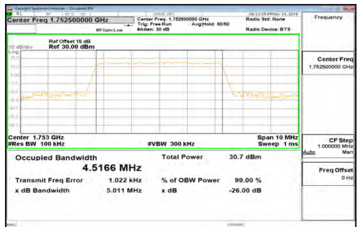
Band4_5MHz_QPSK_25_0_Main_HighCH20375-1752.5
