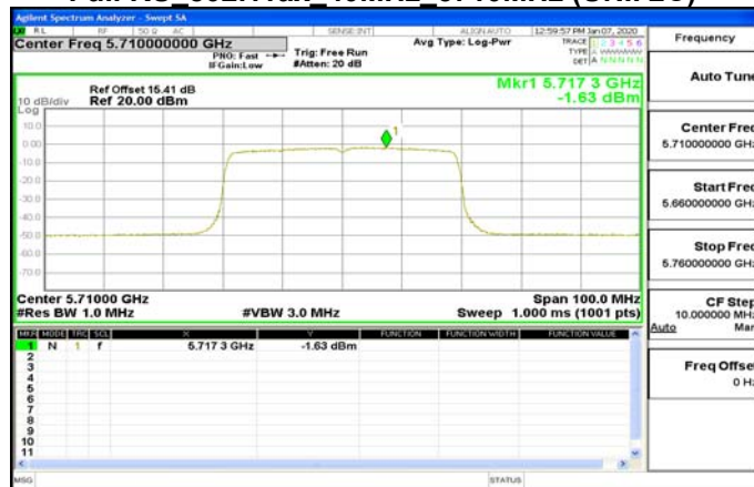
Full RU 802.11ax 40MHz 5710MHz (UNII 2C)
