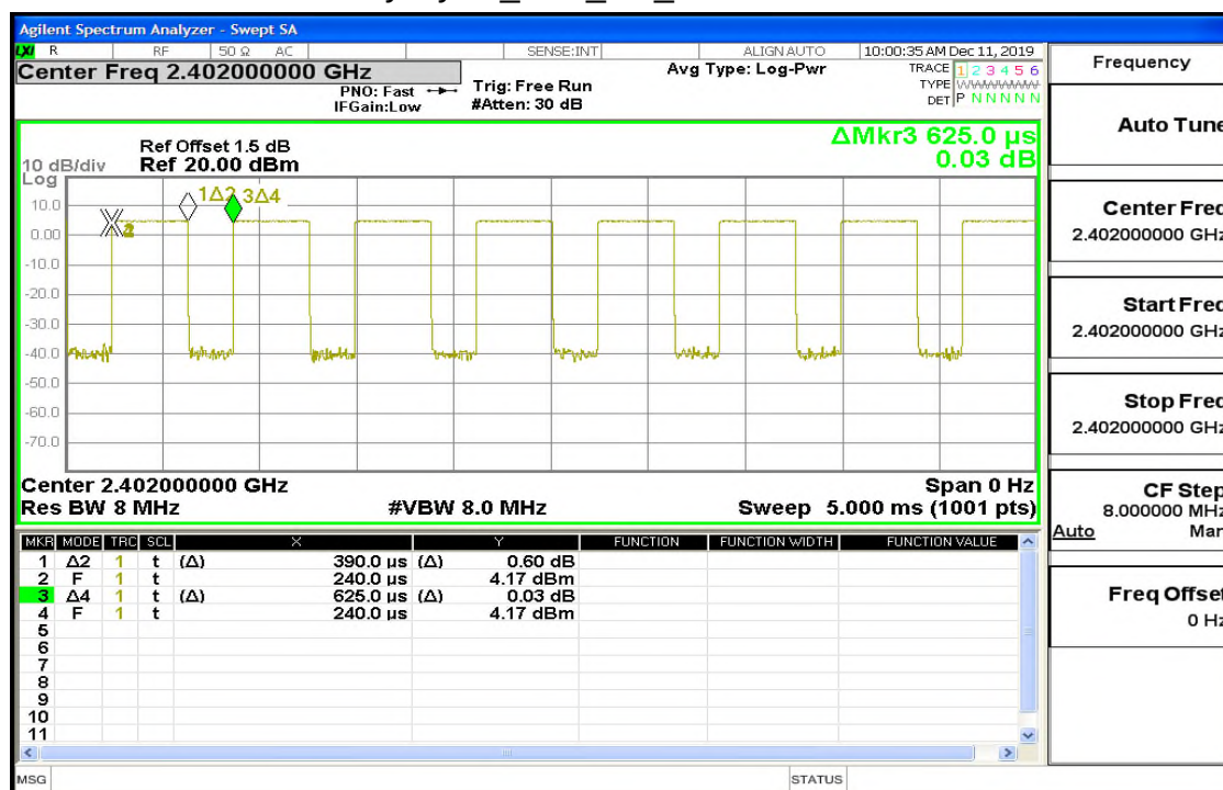
Duty Cycle_BLE_1M_LowCH00-2402
