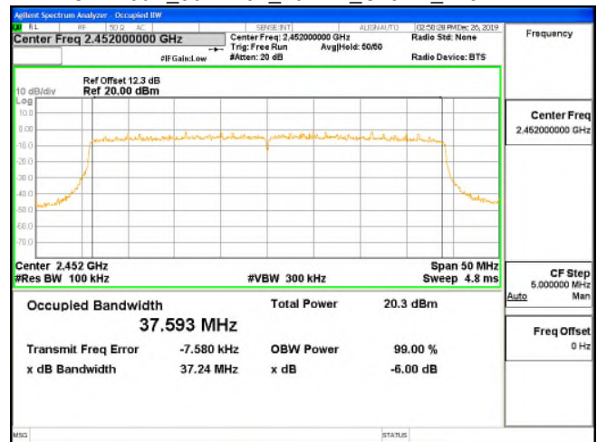
OBW 6dB_802.11ax_40MHz_Chain1_2452MHz
