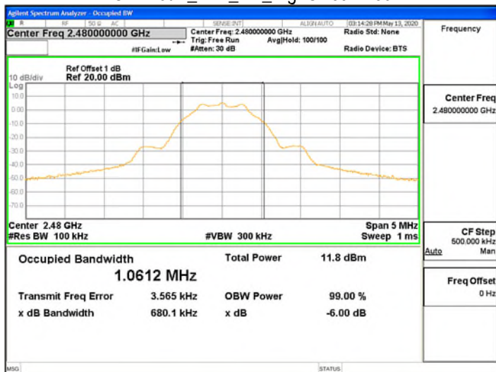
OBW 6dB_BLE_1M_HighCH39-2480
