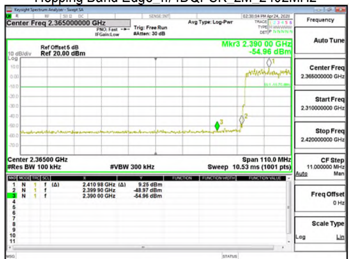
Hopping Band Edge_π/4QPSK_2M_2402MHz
