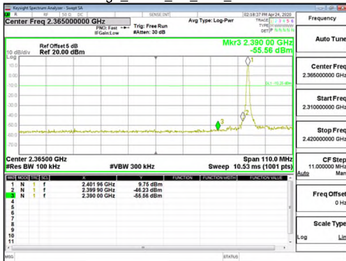
Hopping Band Edge_GFSK_1M_DH5_2402MHz
