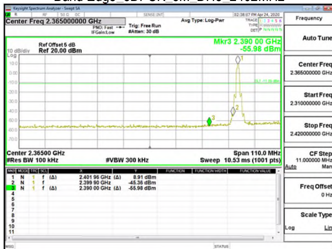
Band Edge_8DPSK_3M_DH5_2402MHz
