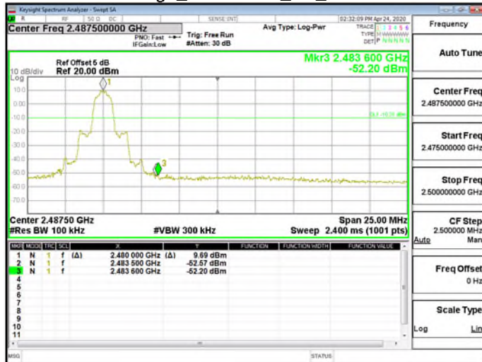
Hopping Band Edge_π/4DQPSK_2M_2480MHz
