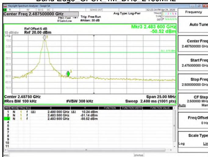
Band Edge_GFSK_1M_DH5_2480MHz
