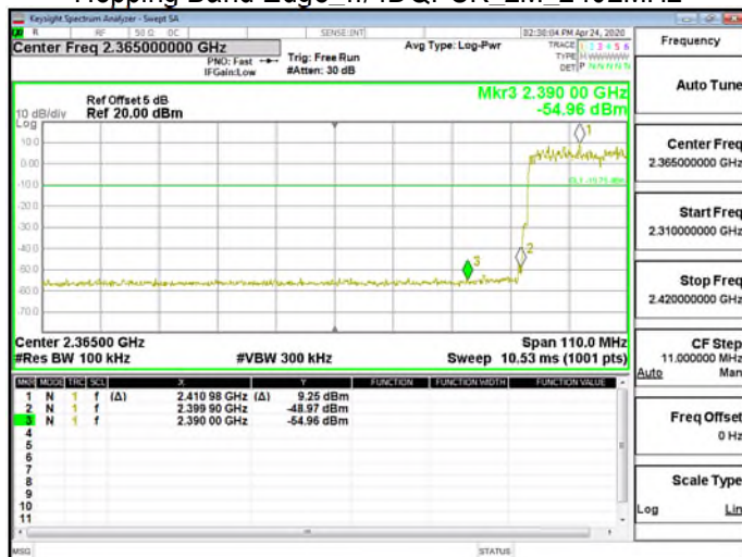
Hopping Band Edge_π/4QPSK_2M_2402MHz
