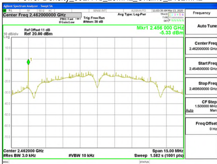
Power Density_802.11b_20MHz_Chain0_2462MHz
