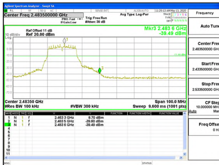
Band Edge_802.11g_20MHz_Chain0_2462MHz
