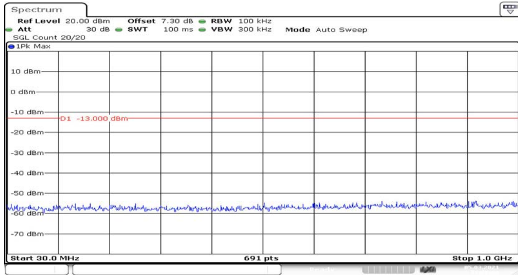
Channel 661 30MHz~1GHz(dBm)
