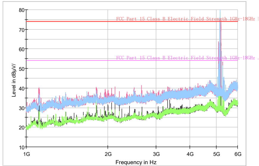
Full Spectrum
