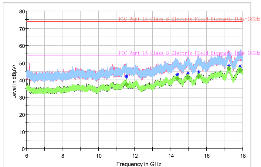
Full Spectrum
