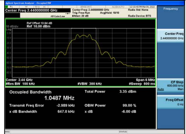
Test Mode:Coded 500K MHz
