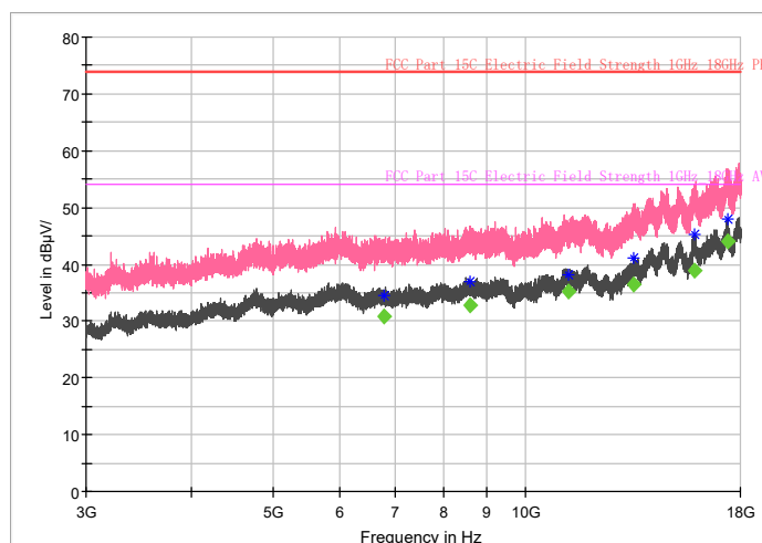
Full Spectrum
