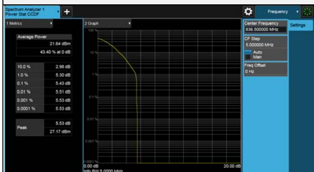
64QAM CH 20525 (836.5MHz)
