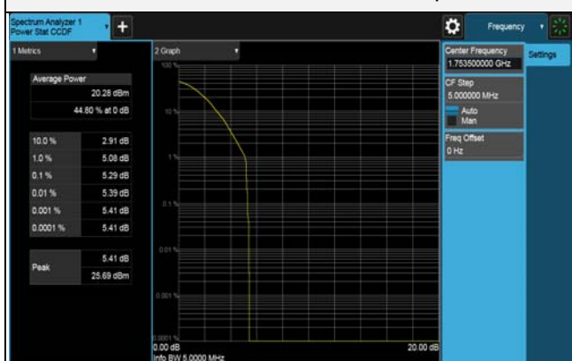
64QAM CH 20385 (1753.5MHz)
