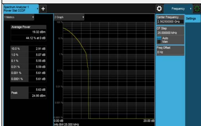
64QAM CH 21375 (2562.5MHz)
