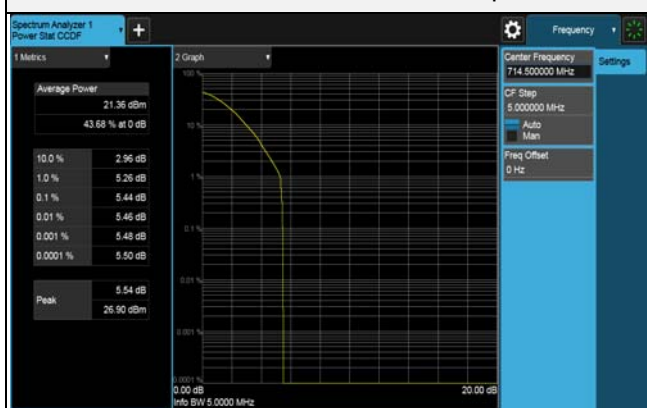
64QAM CH 23165 (714.5MHz)
