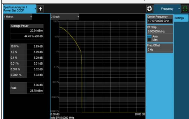
64QAM CH 19957 (1710.7MHz)
