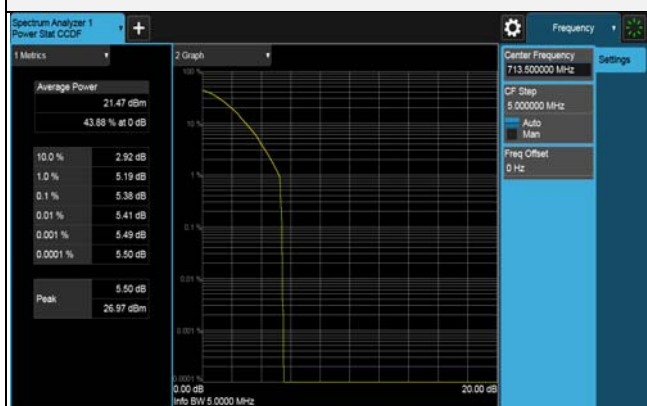
64QAM CH 23825 (713.5MHz)
