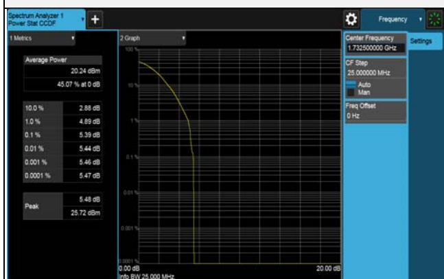
64QAM CH 20175 (1732.5MHz)
