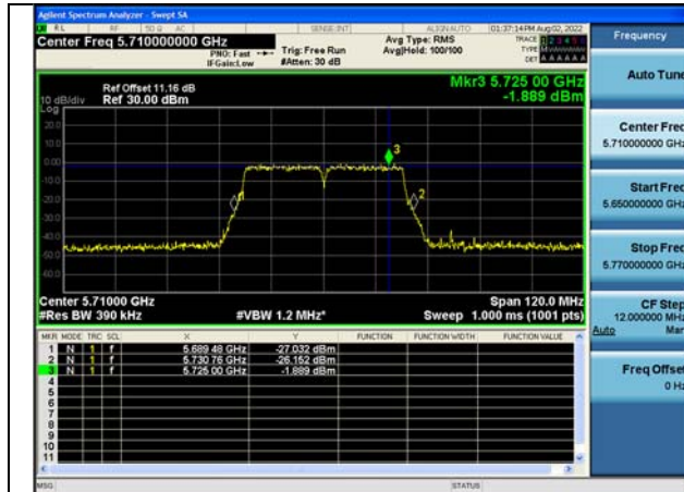
Test Mode:802.11ac VHT40 5710MHz Chain0 NII2C
