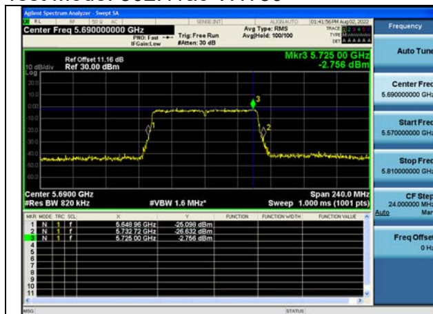
Test Mode:802.11ac VHT80 5690MHz Chain0 NII2C
