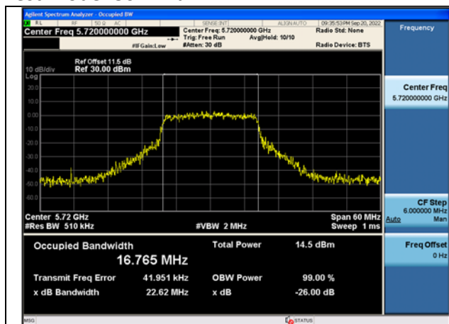
Test Mode:802.11a 5720MHz Chain0
