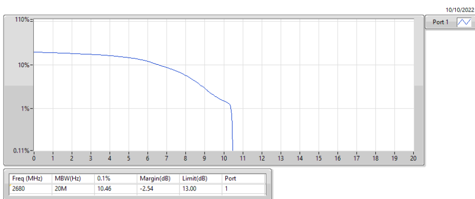
Band 41_LTE_20MHz_Nss1,16QAM_1TX 2680MHz_16QAM_RB 1,#RB M
