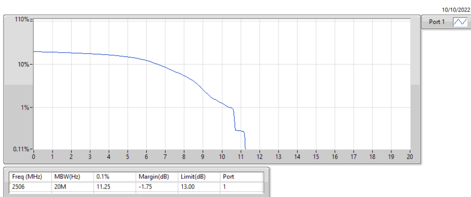
Band 41_LTE_20MHz_Nss1,64QAM_1TX 2506MHz_64QAM_RB 1,#RB M
