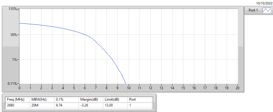
Band 41_LTE_20MHz_Nss1,16QAM_1TX 2680MHz_16QAM_RB 100,#RB 0
