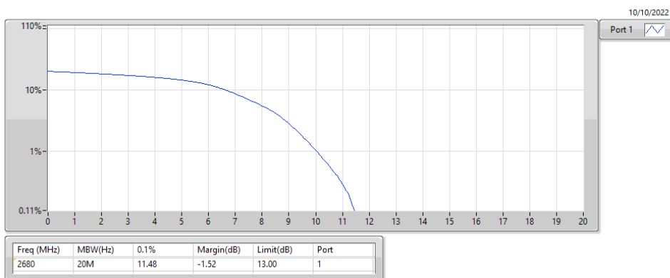
Band 41_LTE_20MHz_Nss1,16QAM_1TX 2680MHz_16QAM_RB 50,#RB M
