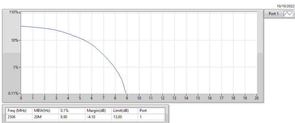
Band 41_LTE_20MHz_Nss1,64QAM_1TX 2506MHz_64QAM_RB 50,#RB M
