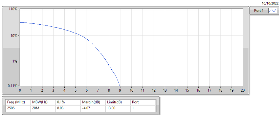
Band 41_LTE_20MHz_Nss1,64QAM_1TX 2506MHz_64QAM_RB 100,#RB 0
