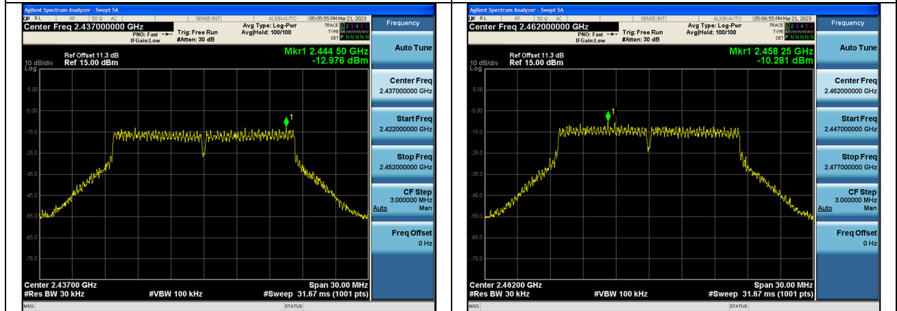
Test Mode:802.11g 2437MHz Chain1
