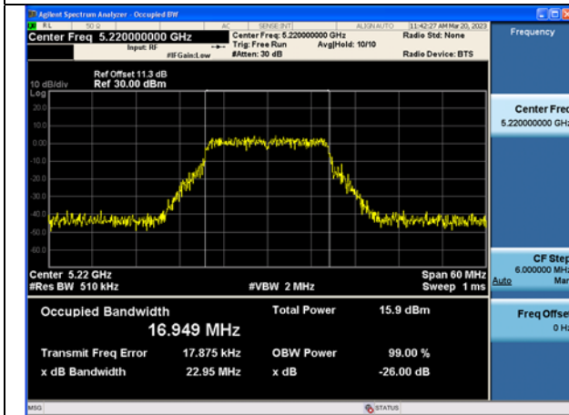
Test Mode:802.11a 5220MHz Chain1
