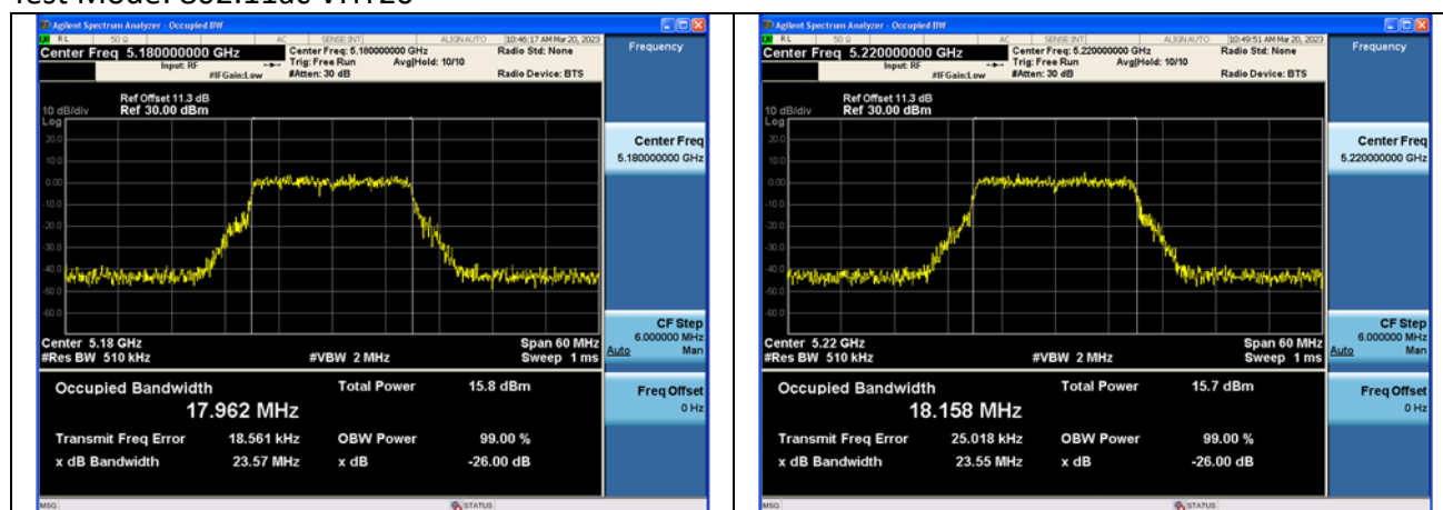
Test Mode:802.11ac VHT20 5180MHz Chain0
