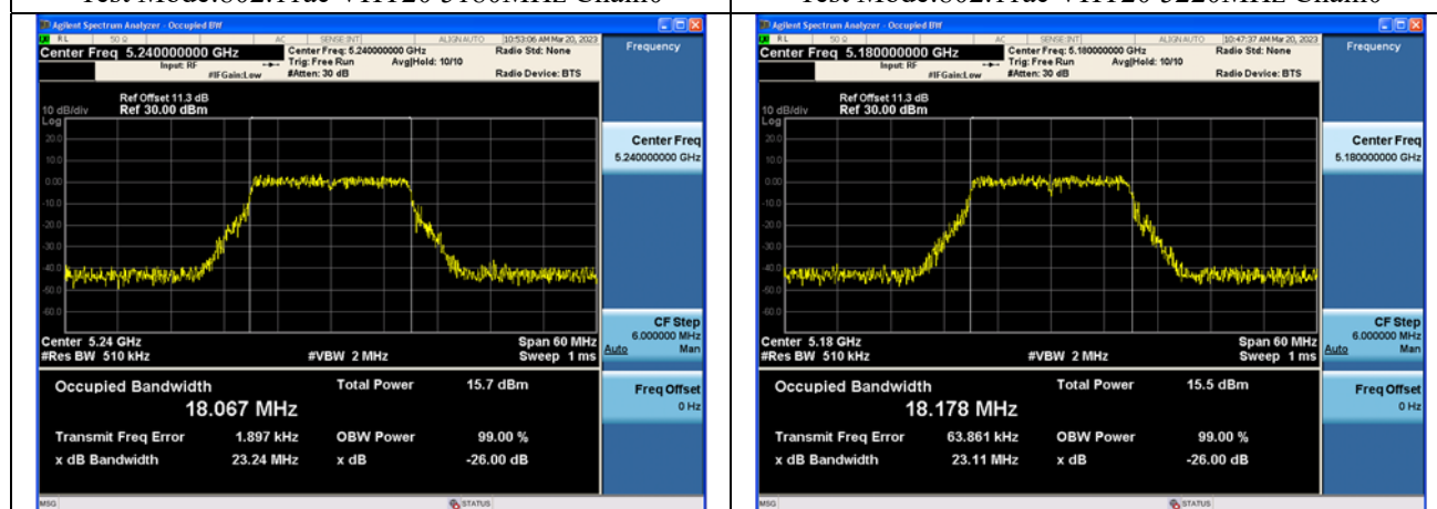
Test Mode:802.11ac VHT20 5240MHz Chain0
