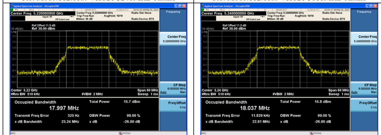
Test Mode:802.11ac VHT20 5220MHz Chain1
