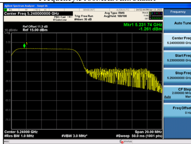
Mode:802.11ax HE20 Tone:106T Frequency:5240MHz Ant:Chain1
