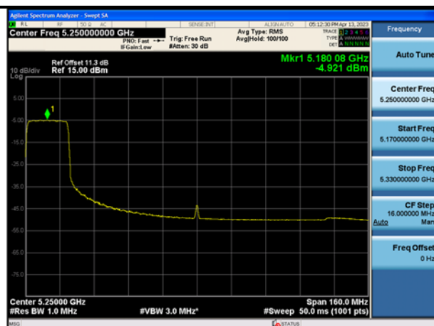
Mode:802.11ax HE160 Tone:242T Frequency:5250MHz Ant:Chain1
