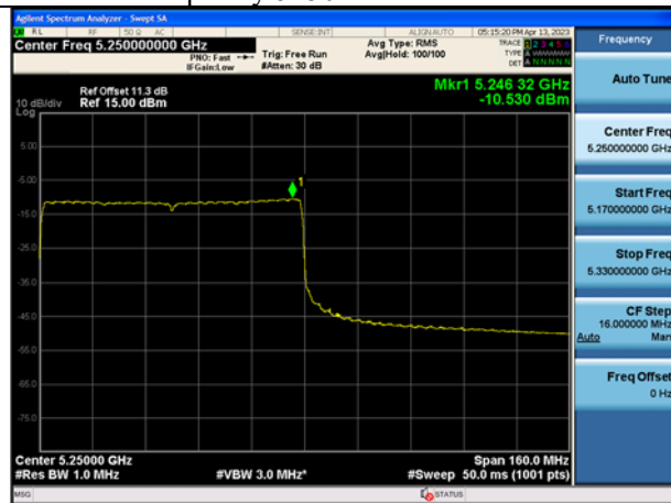
Mode:802.11ax HE160 Tone:996T Frequency:5250MHz Ant:Chain1
