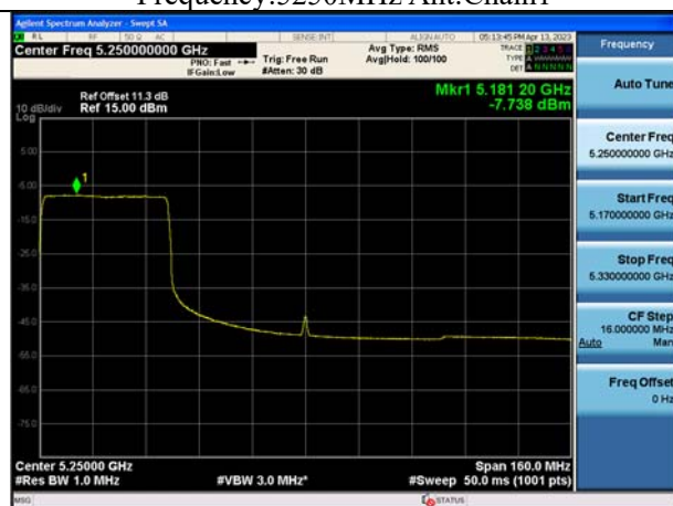
Mode:802.11ax HE160 Tone:484T Frequency:5250MHz Ant:Chain1
