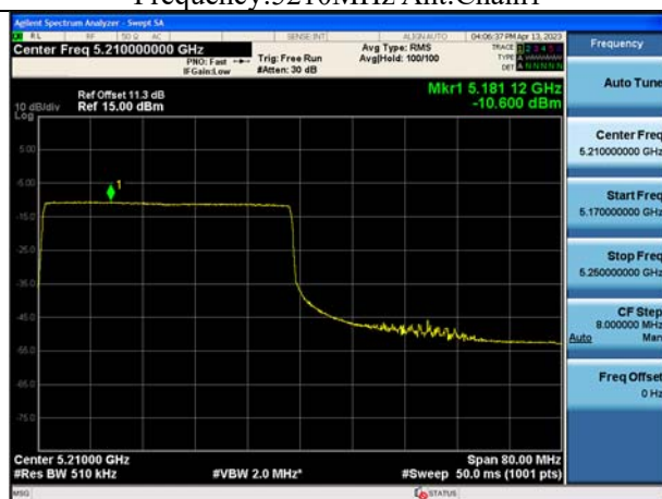
Mode:802.11ax HE80 Tone:484T Frequency:5210MHz Ant:Chain1
