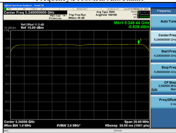
Mode:802.11ax HE20 Tone:242T Frequency:5240MHz Ant:Chain1
