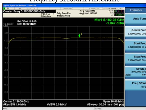
Mode:802.11ax HE20 Tone:242T Frequency:5180MHz Ant:Chain1
