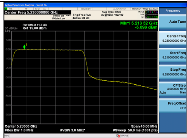
Mode:802.11ax HE40 Tone:242T Frequency:5230MHz Ant:Chain0
