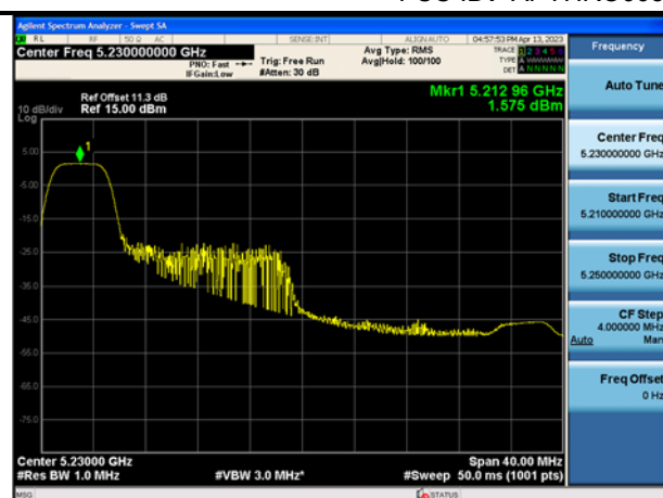
Mode:802.11ax HE40 Tone:52T Frequency:5230MHz Ant:Chain1
