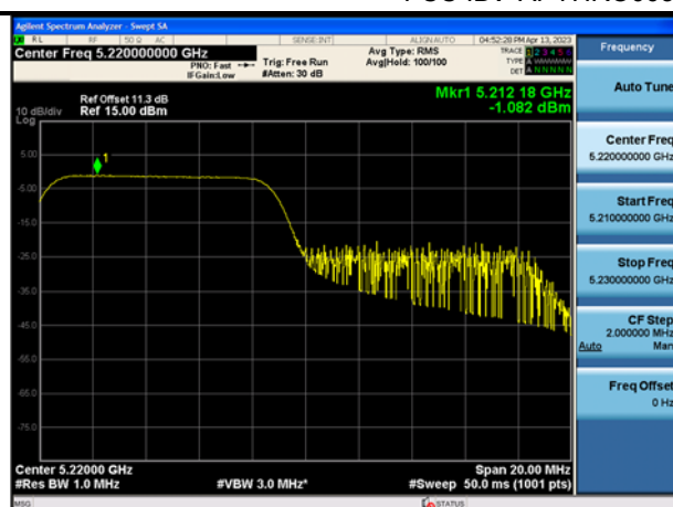
Mode:802.11ax HE20 Tone:106T Frequency:5220MHz Ant:Chain0
