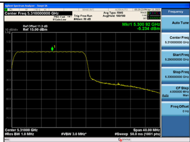
Mode:802.11ax HE40 Tone:242T Frequency:5310MHz Ant:Chain0
