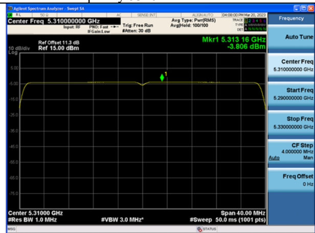
Mode:802.11ax HE40 Tone:484T Frequency:5310MHz Ant:Chain0
