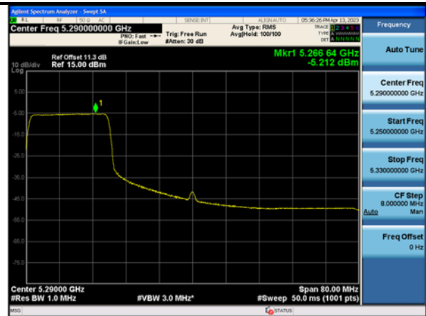
Mode:802.11ax HE80 Tone:242T Frequency:5290MHz Ant:Chain1
