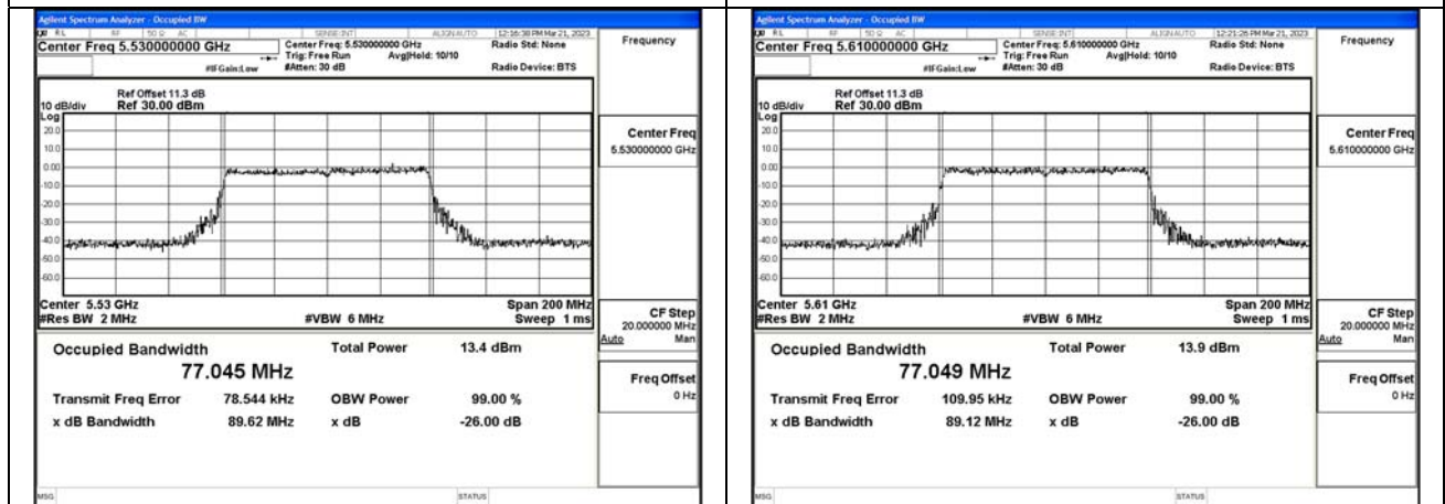
Test Mode:802.11ac VHT80 5530MHz Chain1
