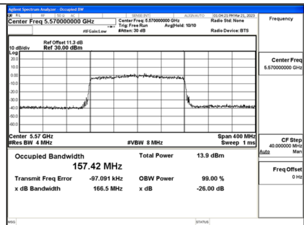
Test Mode:802.11ax HE160 5570MHz Chain1
