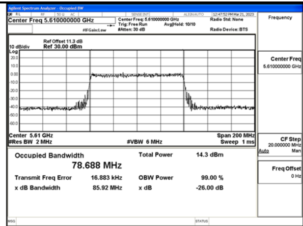
Test Mode:802.11ax HE80 5610MHz Chain1
