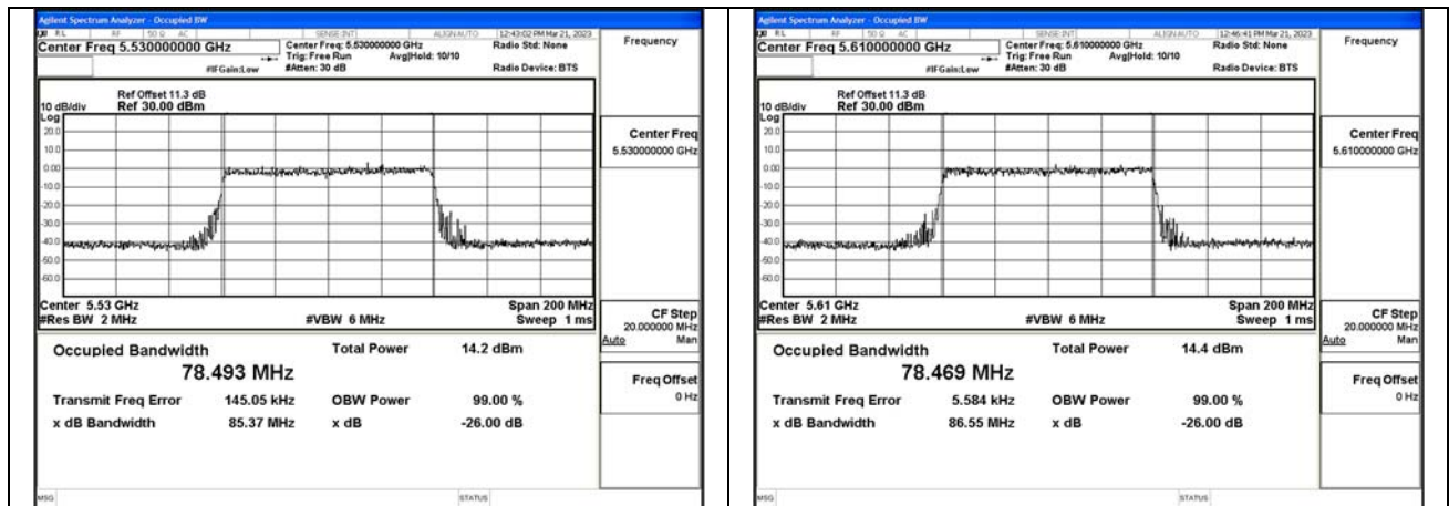
Test Mode:802.11ax HE80 5530MHz Chain0
