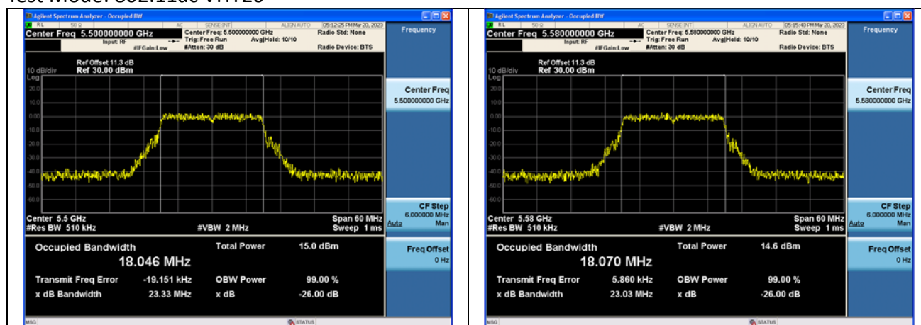
Test Mode:802.11ac VHT20 5500MHz Chain0
