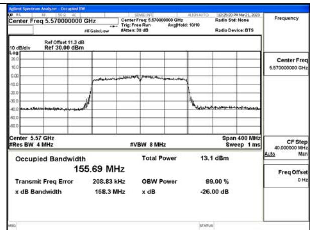
Test Mode:802.11ac VHT160 5570MHz Chain1
