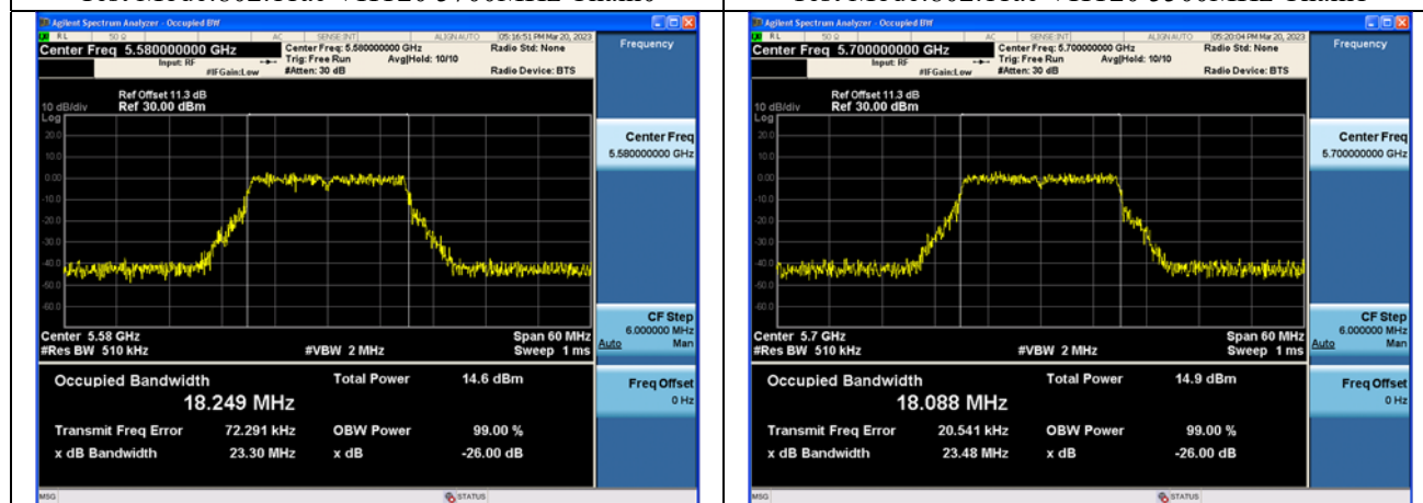
Test Mode:802.11ac VHT20 5580MHz Chain1
