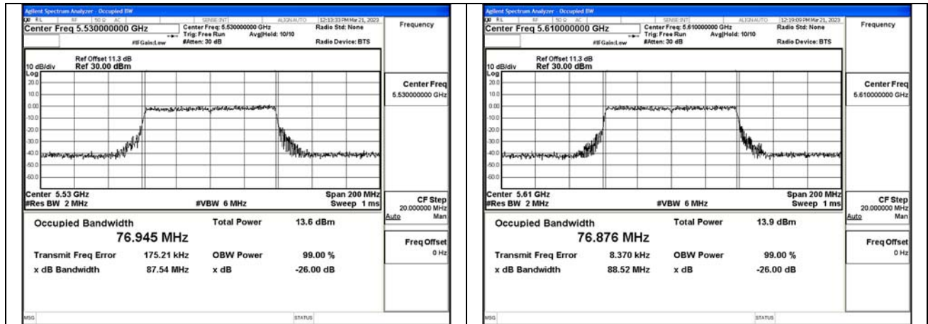
Test Mode:802.11ac VHT80 5530MHz Chain0
